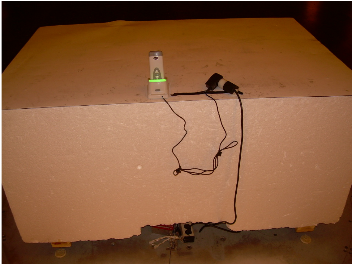
Photograph 7 – Front View CR2611_01 Radiated Emissions Setup – Charging Base Configuration
