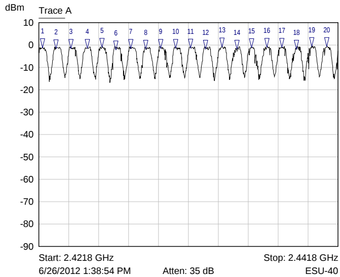
Trace A middle lower 20 channels
