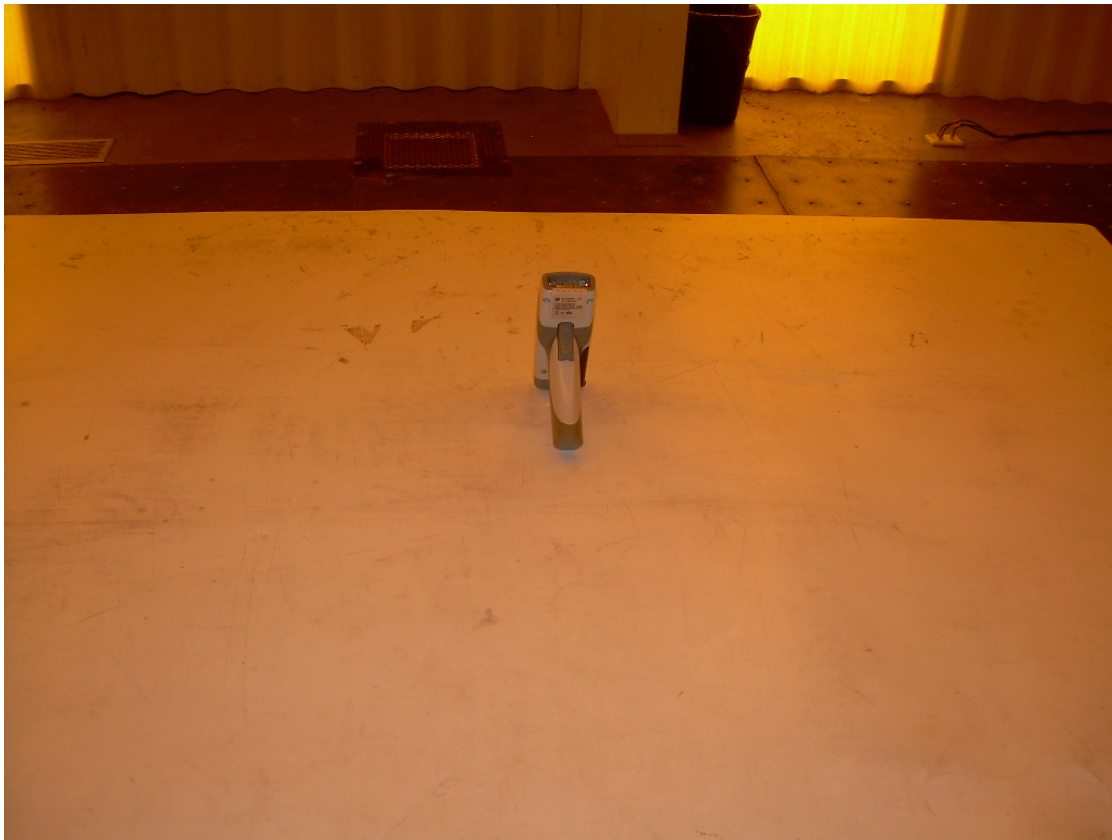
Photograph 1 – Front View CR2612_01 Radiated Emissions Setup – Vertical Configuration
