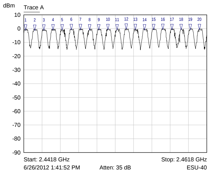
Trace A middle upper 20 channels
