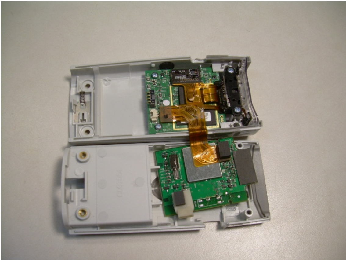
Photograph 16 – View with the Housing Opened Showing PCB Placement
