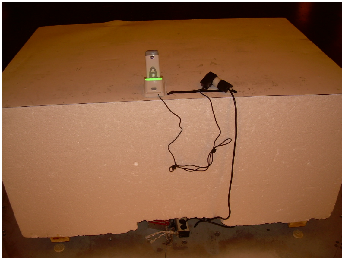
Front View CR2611_01 Radiated Emissions Setup – Charging Base Configuration
