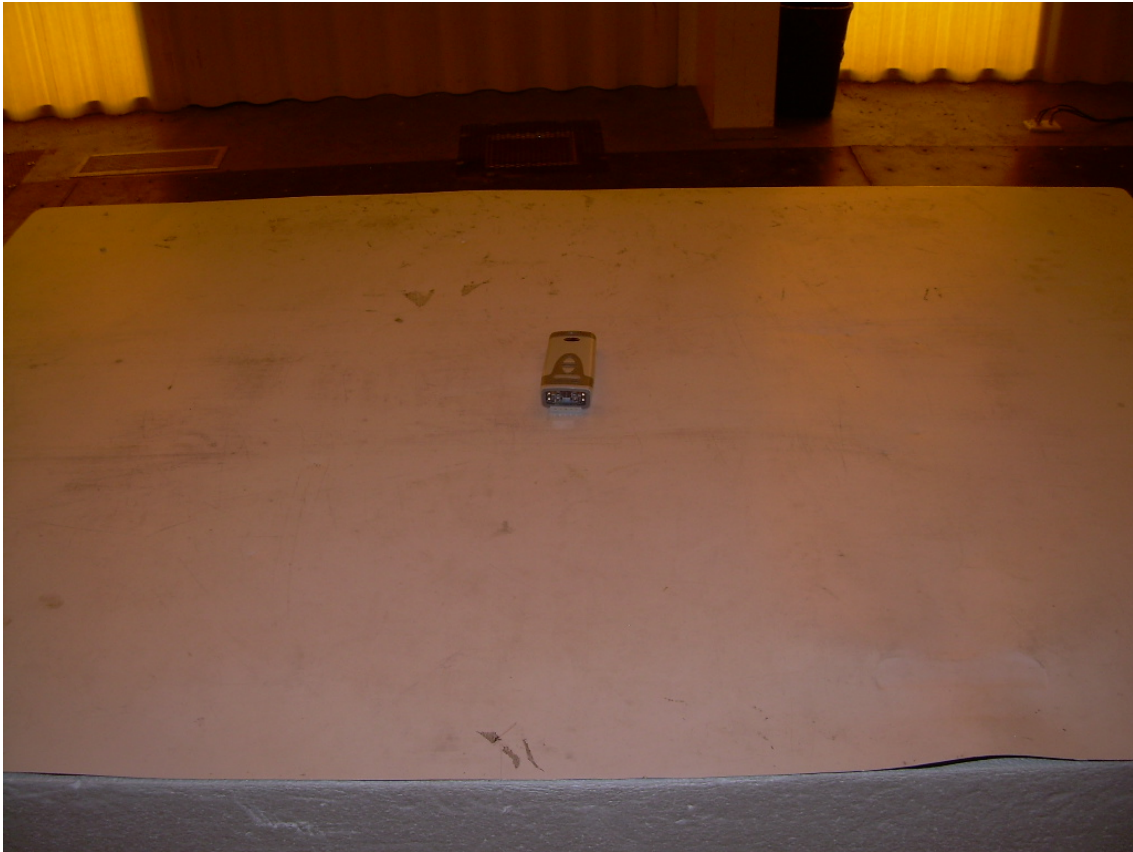
Front View CR2611_01 Radiated Emissions Setup – Horizontal Configuration
