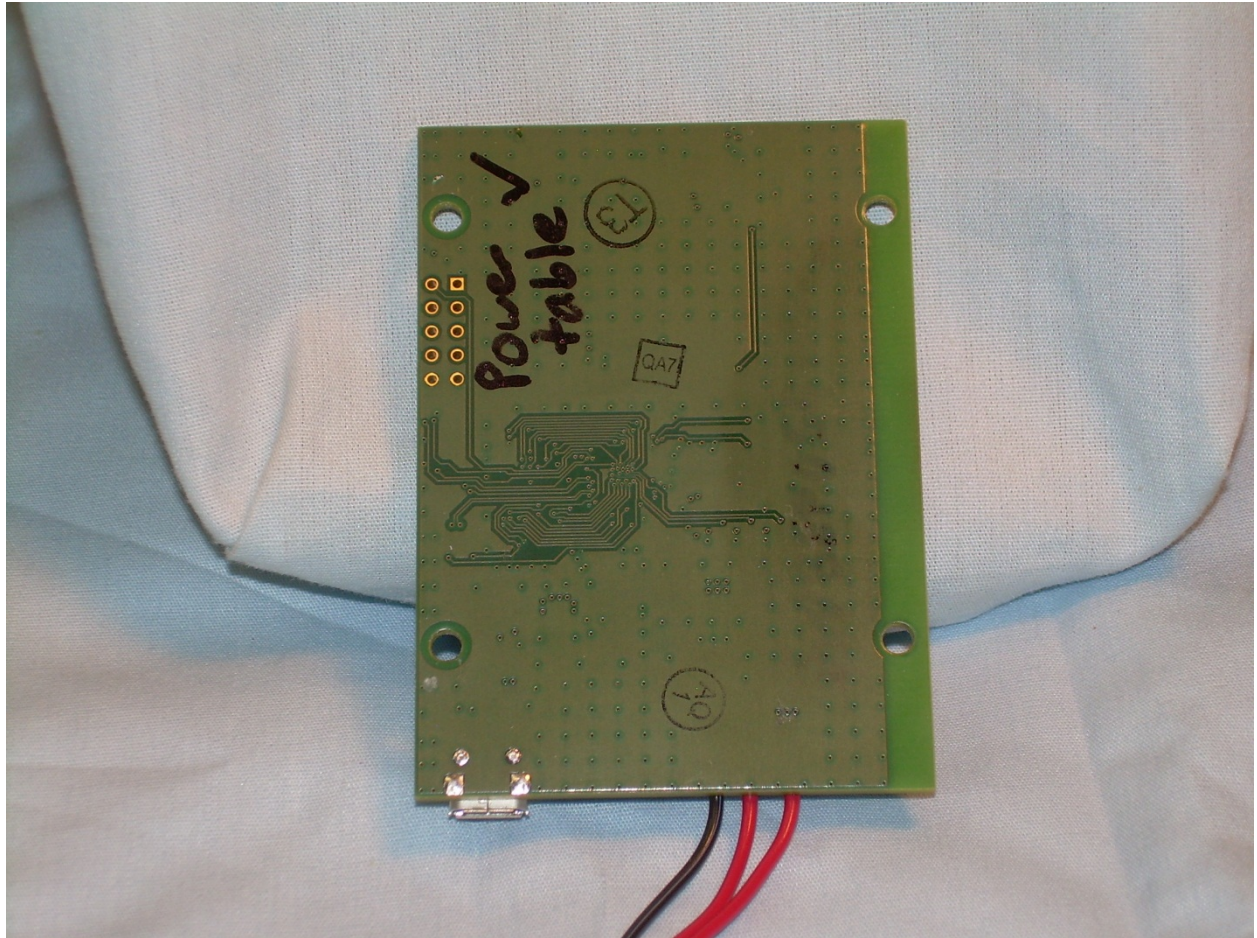
View of the Trace Side of the Main PCB
