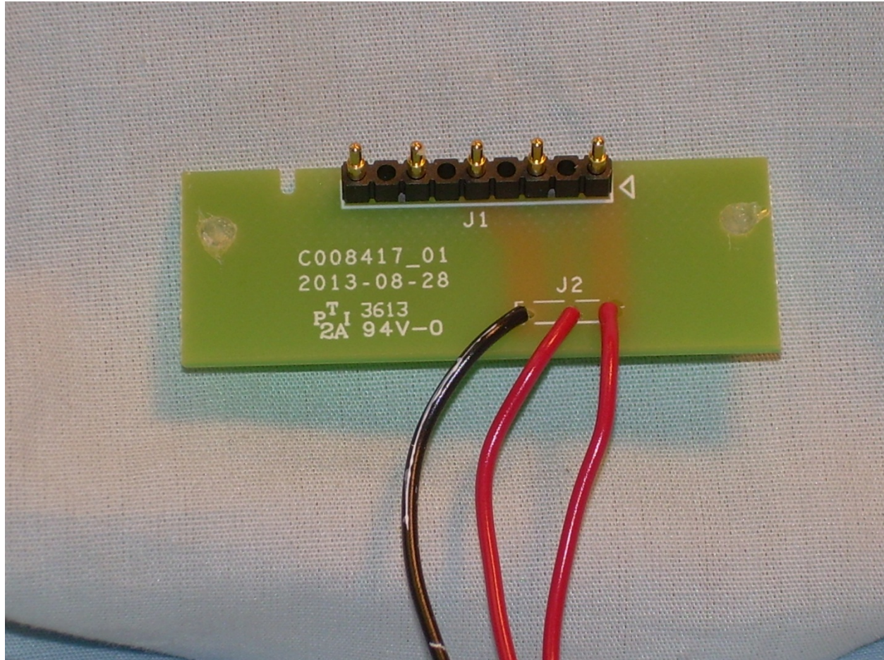
View of the Top Side of the Scanner Interface PCB
