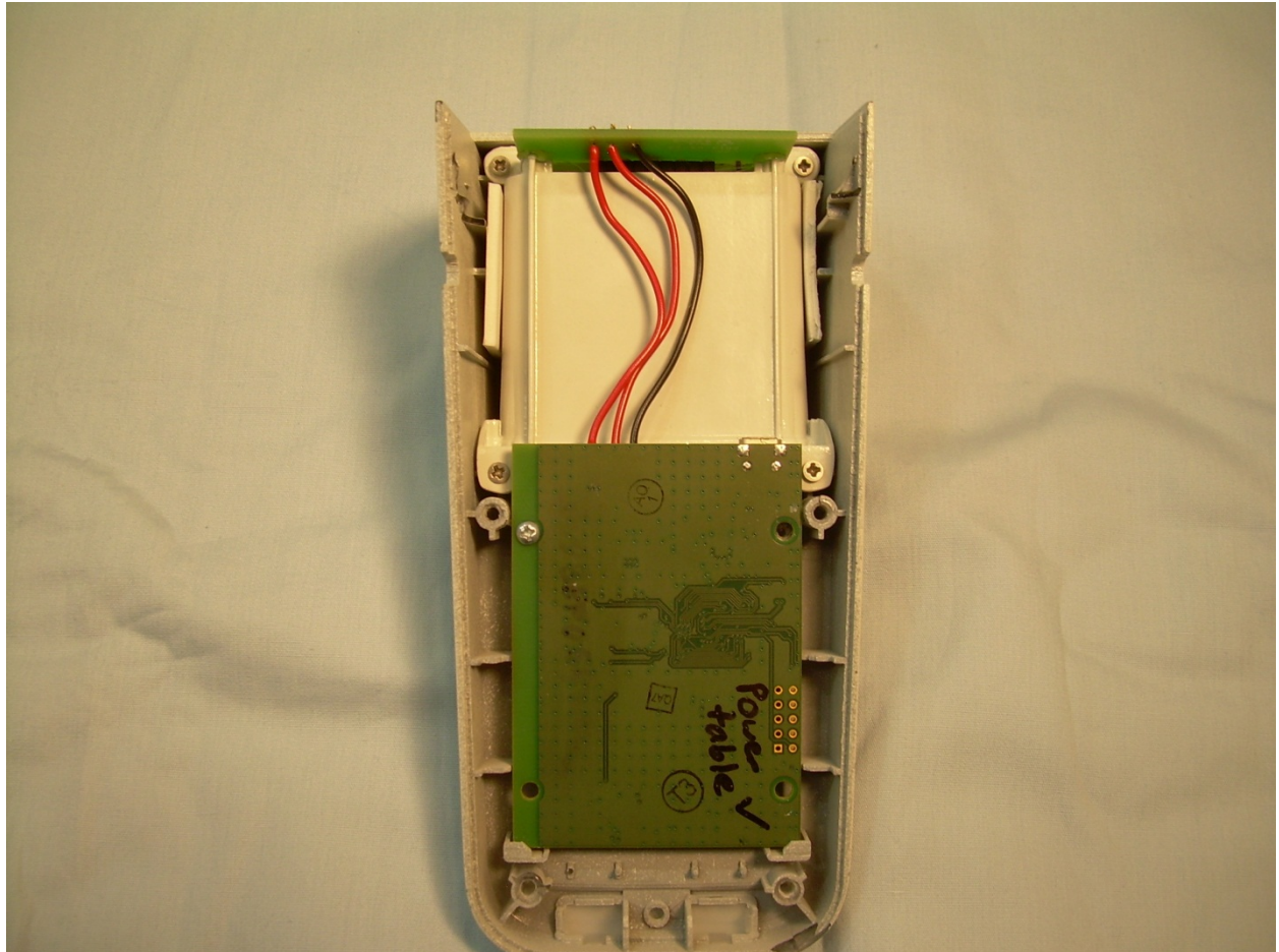
View of the EUT with Back and Bottom Cover Removed
