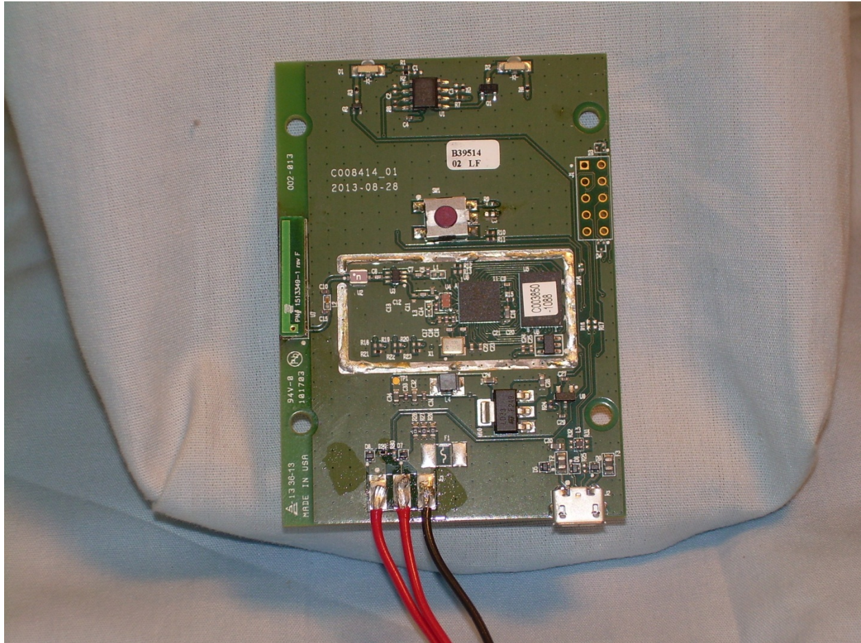
View of the Component Side of the Main PCB
