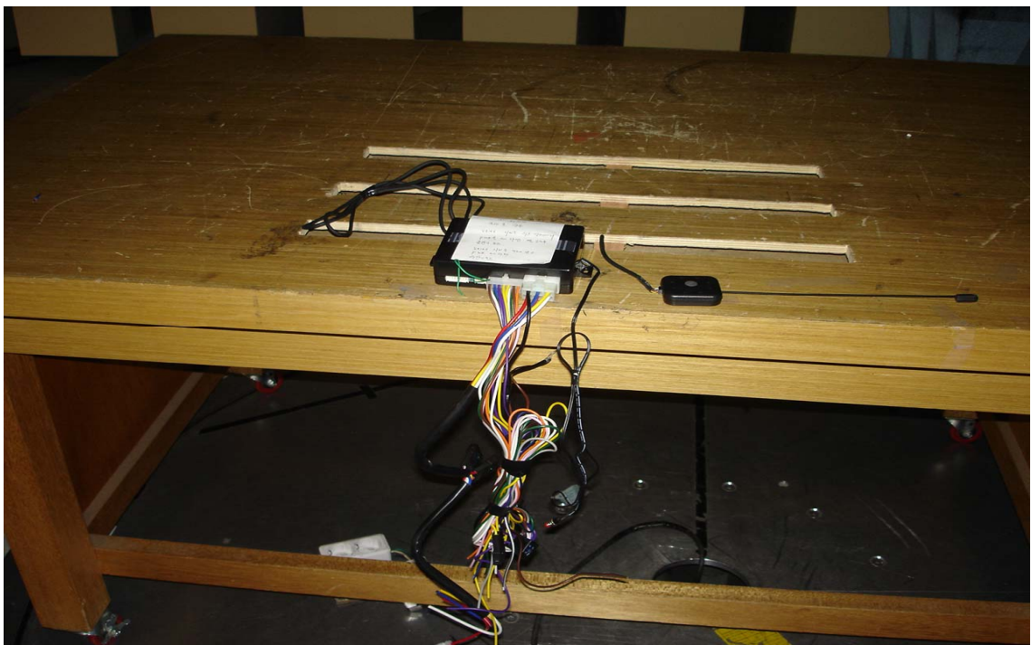
< Radiated emission – Rear >
