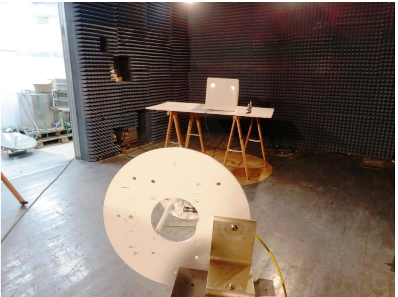
Photograph for Radiated Emission Test Setup/ 5
