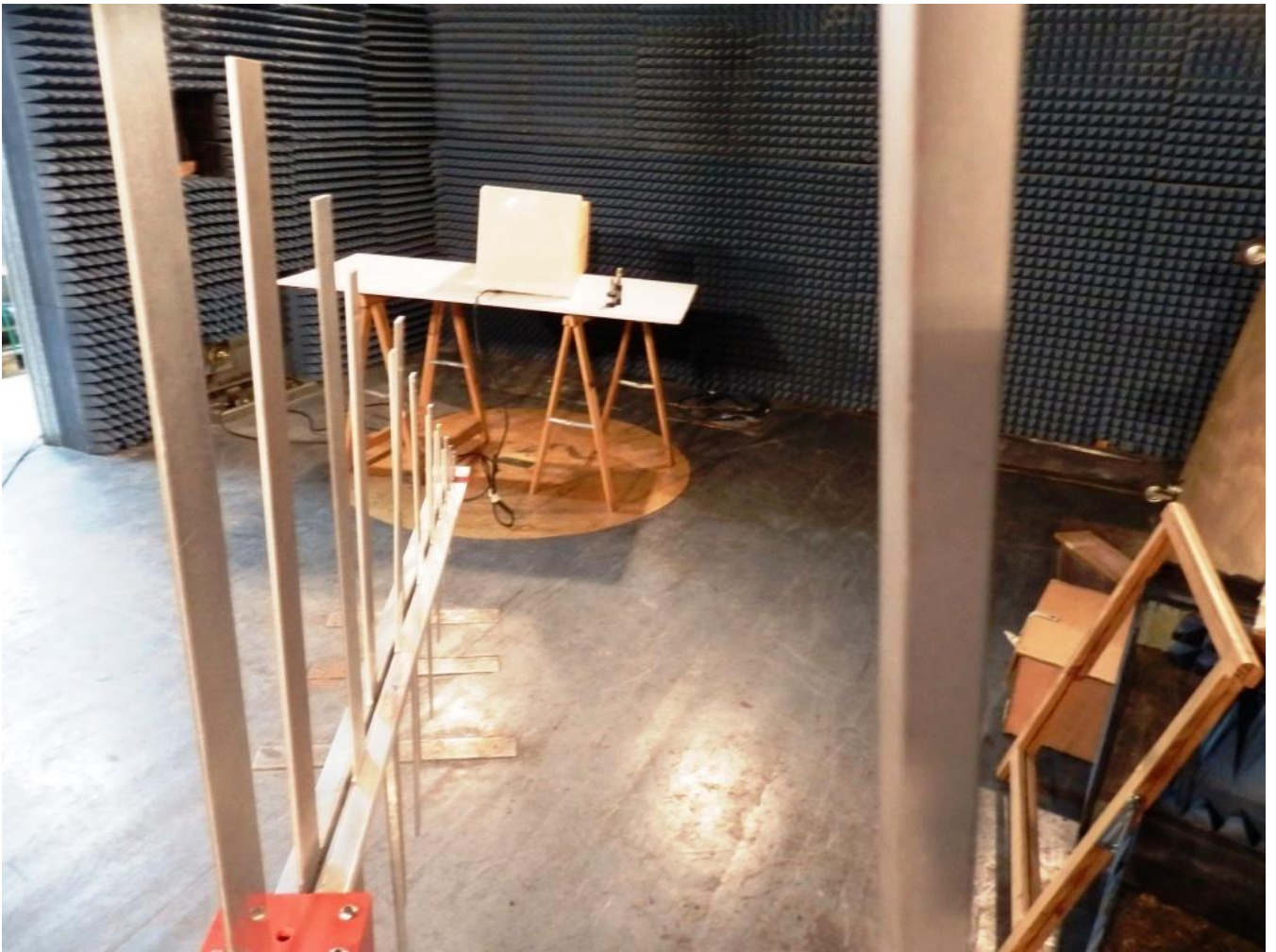
Photograph for Radiated Emission Test Setup/ 6
