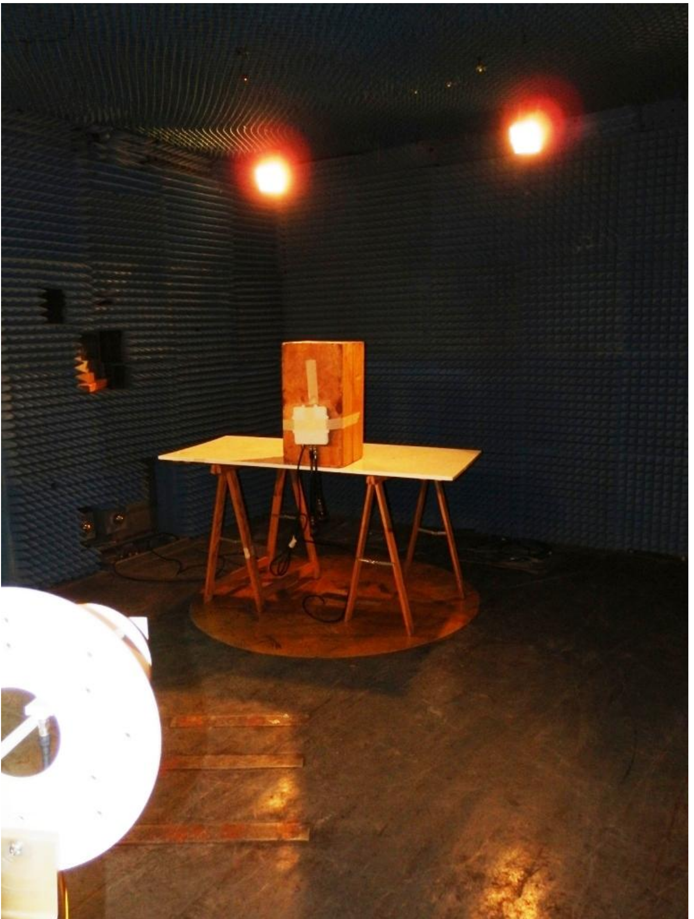
Photograph for Radiated Emission Test Setup/ 2
