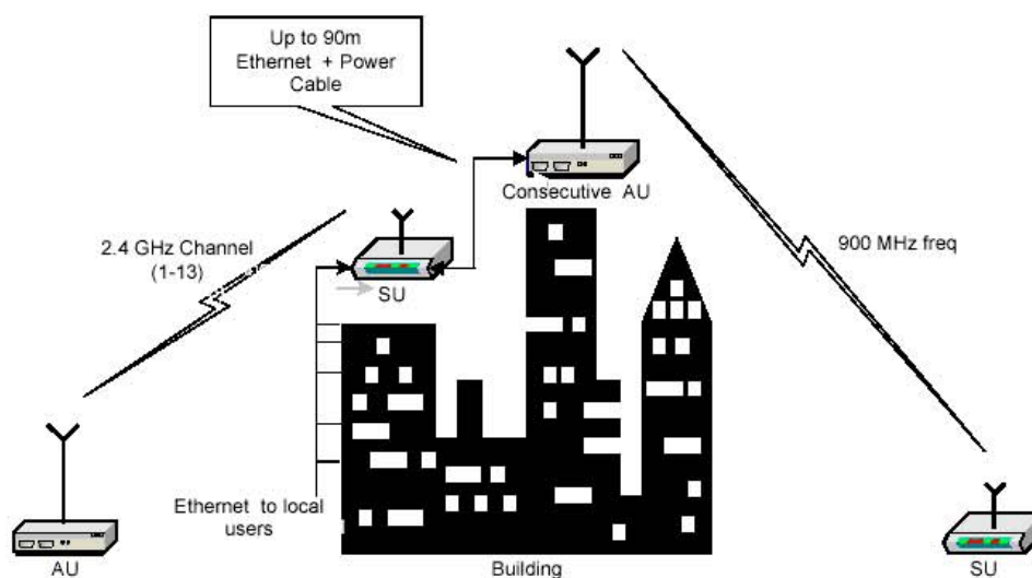
Figure 1-3: Consecutive Sector principle
