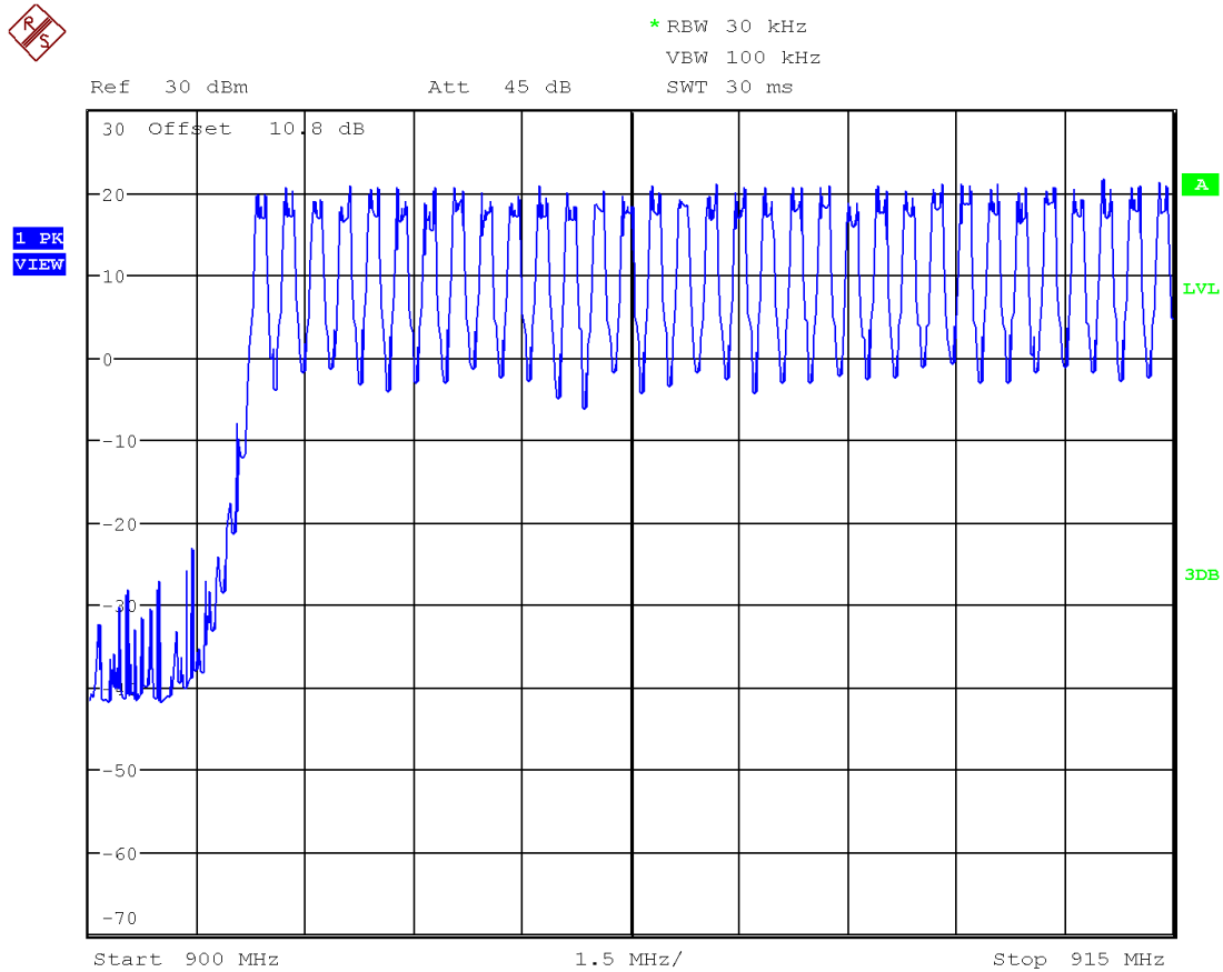
Plot 4.1 - Number of hopping channels, 900 - 915MHz
