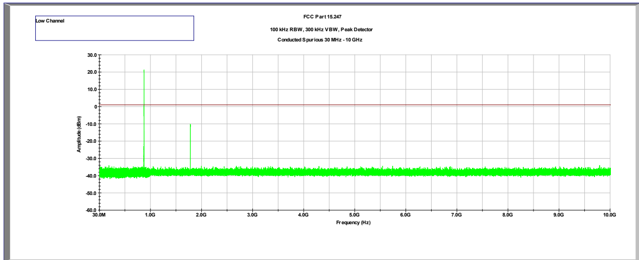
Plot 4.1 Transmitter Spurious, Low Channel
