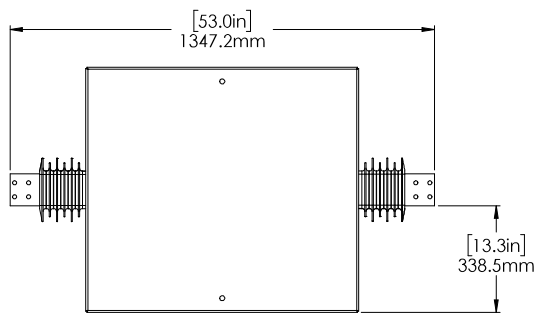
SmartBypass 4000-XX Dimensions
