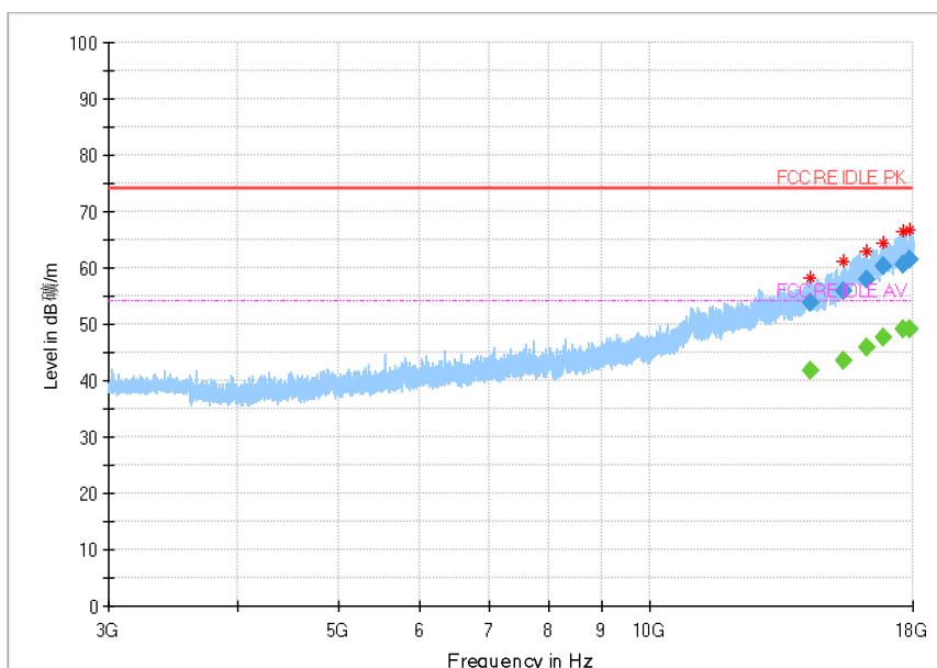
Fig.111 Radiated Spurious Emission (802.11 n-20MHz,Ch11,3GHz~18GHz)
