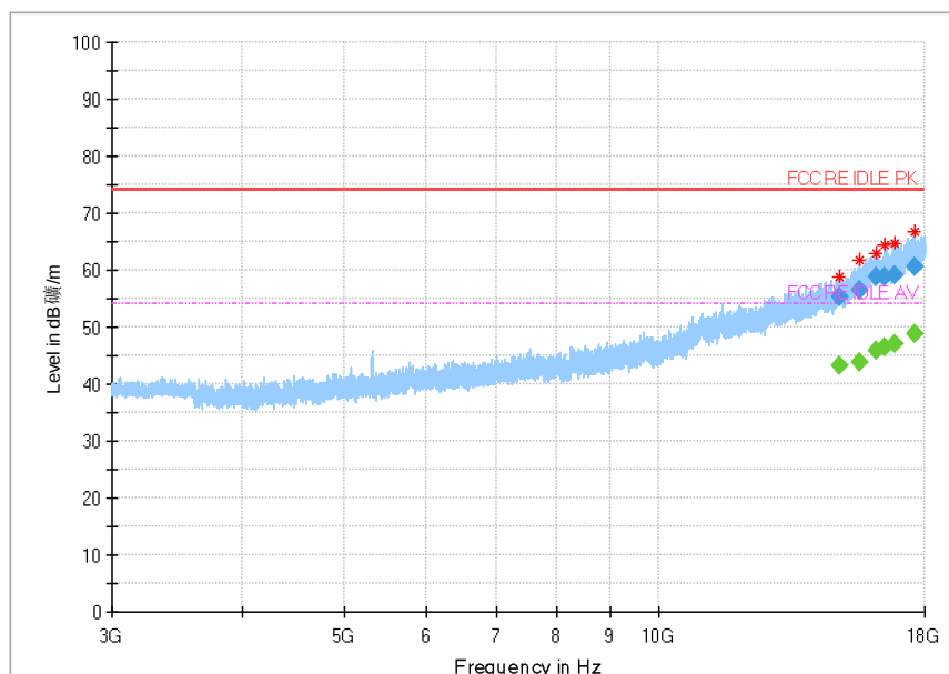
Fig.116 Radiated Spurious Emission (802.11 n-40MHz,Ch3,3GHz~18GHz)
