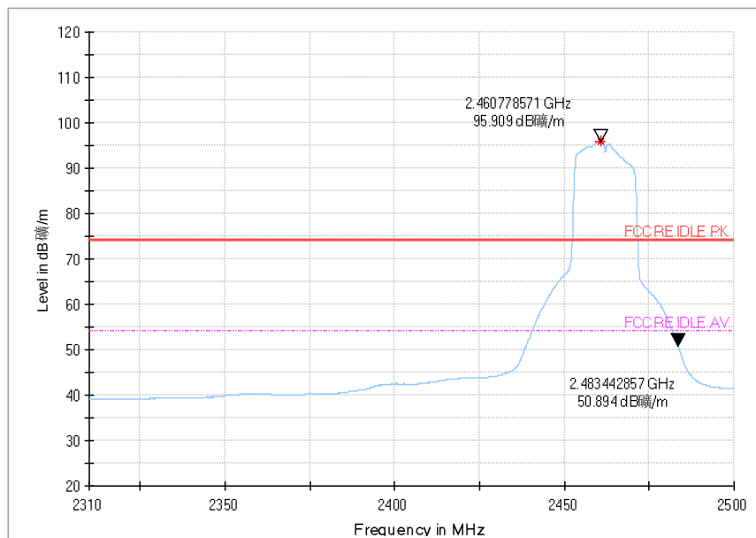
Fig.108 Radiated emission (Power): 802.11n, high channel
