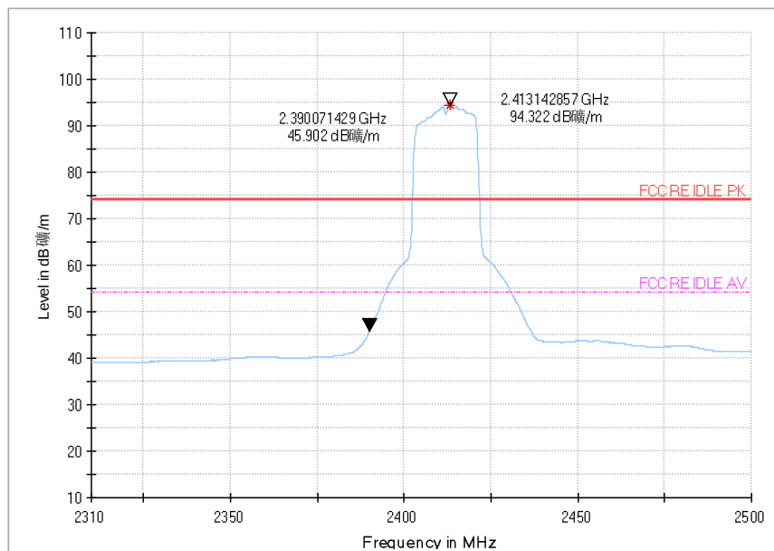
Fig.107 Radiated emission (Power): 802.11n, low channel
