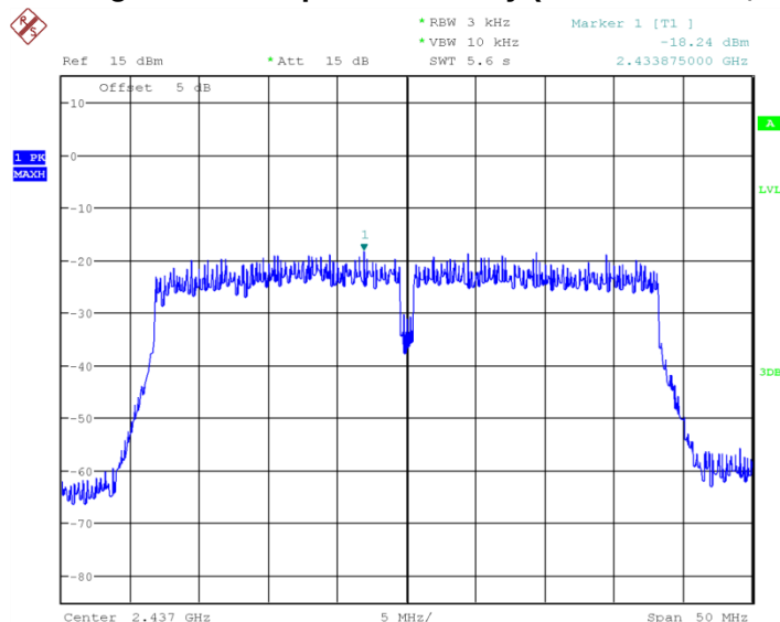
Fig.17 Power Spectral Density (802.1n-40MHz,Ch6)
