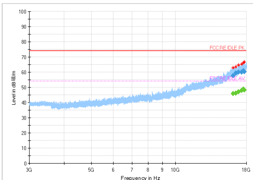
Fig.101 Radiated Spurious Emission (802.11b,Ch11,3GHz~18GHz)
