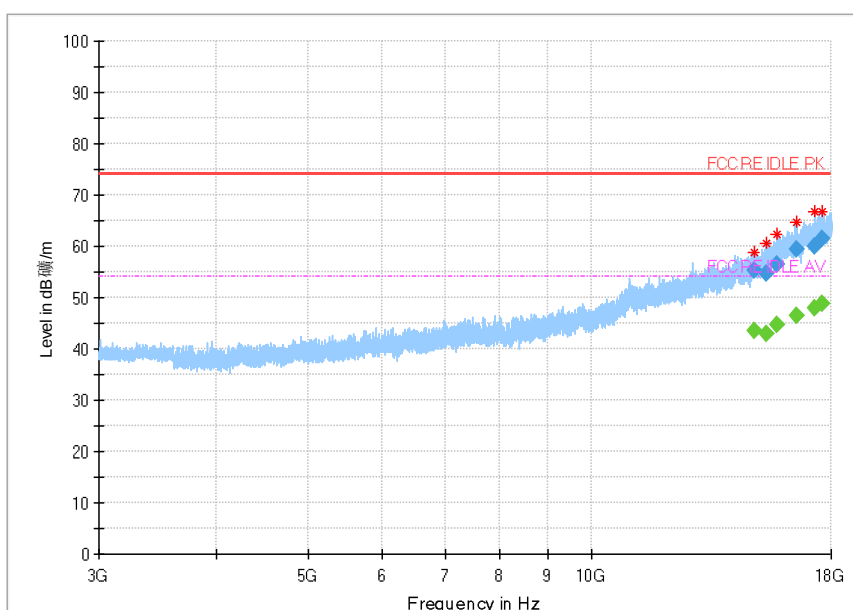
Fig.106 Radiated Spurious Emission (802.11g, Ch11, 3GHz~18GHz)
