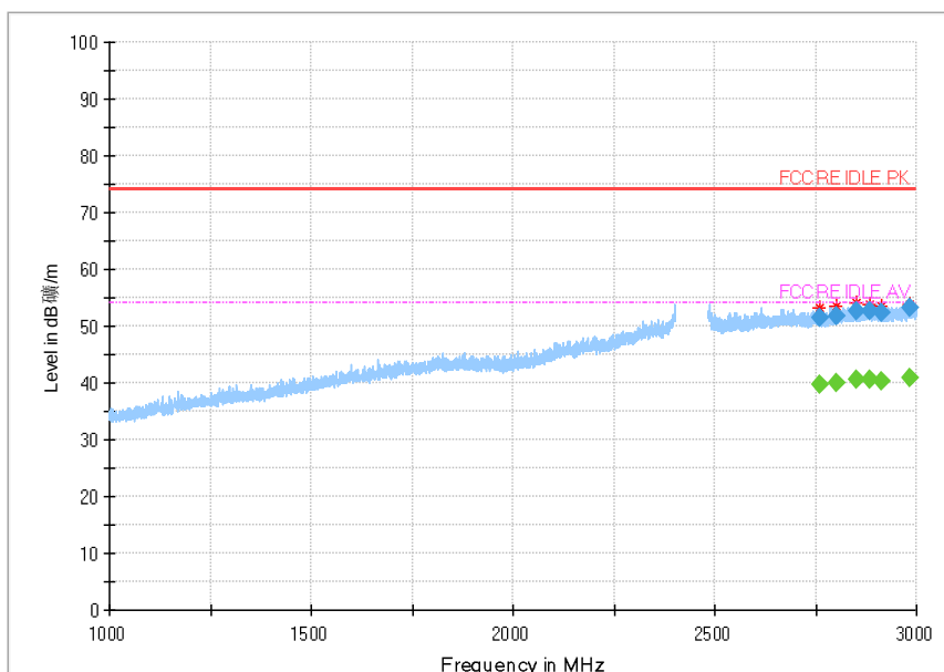
Fig.100 Radiated Spurious Emission (802.11b, Ch11, 1GHz~3GHz)
