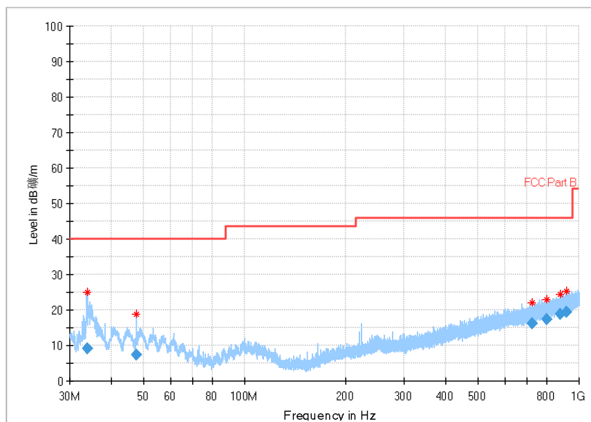
Fig.104 Radiated Spurious Emission (802.11g, Ch11, 30MHz~1GHz)
