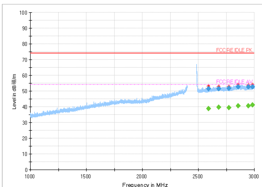
Fig.105 Radiated Spurious Emission (802.11g, Ch11, 1GHz~3GHz)
