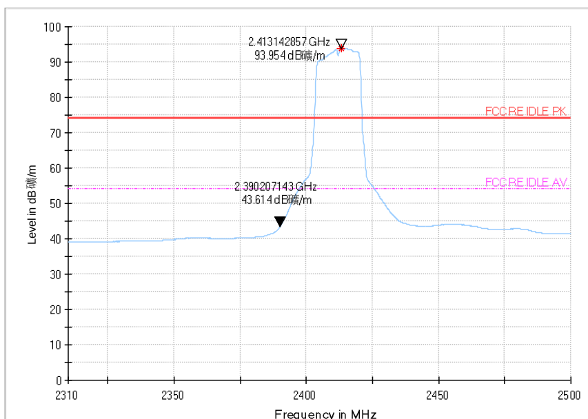
Fig.102 Radiated emission (Power): 802.11g, low channel
