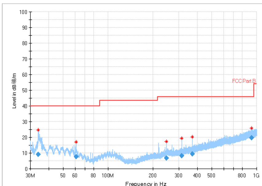
Fig.99 Radiated Spurious Emission (802.11b, Ch11, 30MHz~1GHz)
