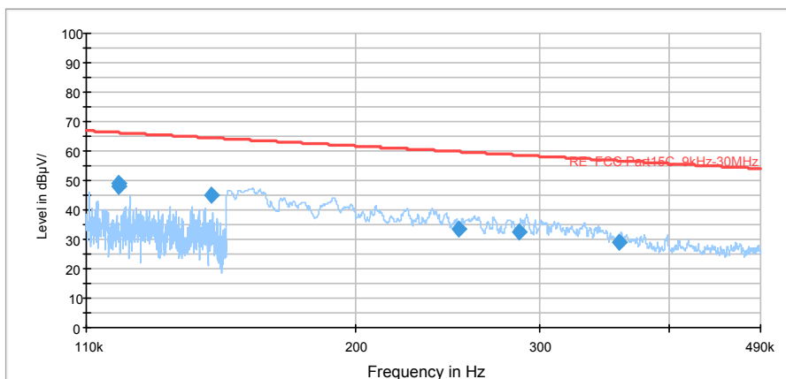
Radiates Emission from 110kHz to 490kHz
