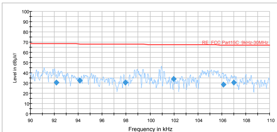
Radiates Emission from 90kHz to 110kHz
