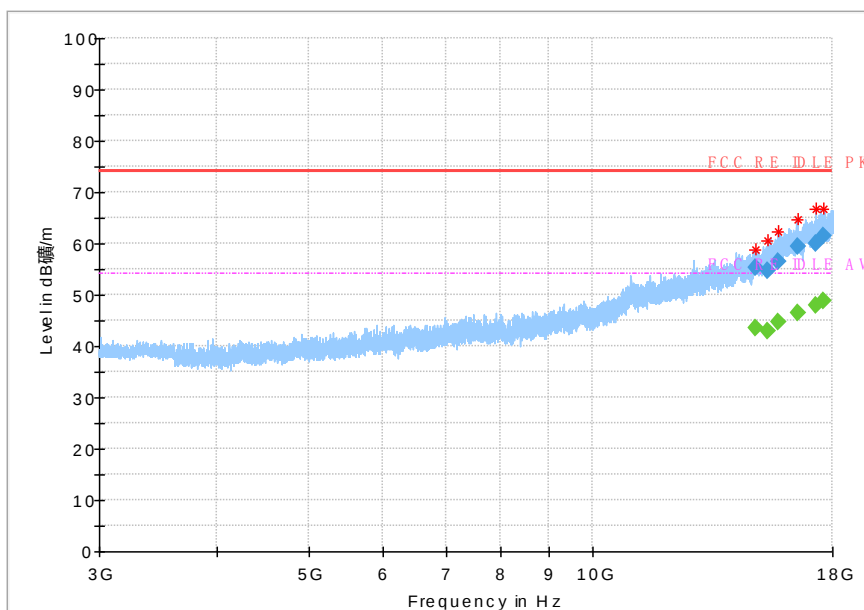
Fig.106 Radiated Spurious Emission (802.11g, Ch11, 3GHz~18GHz)
