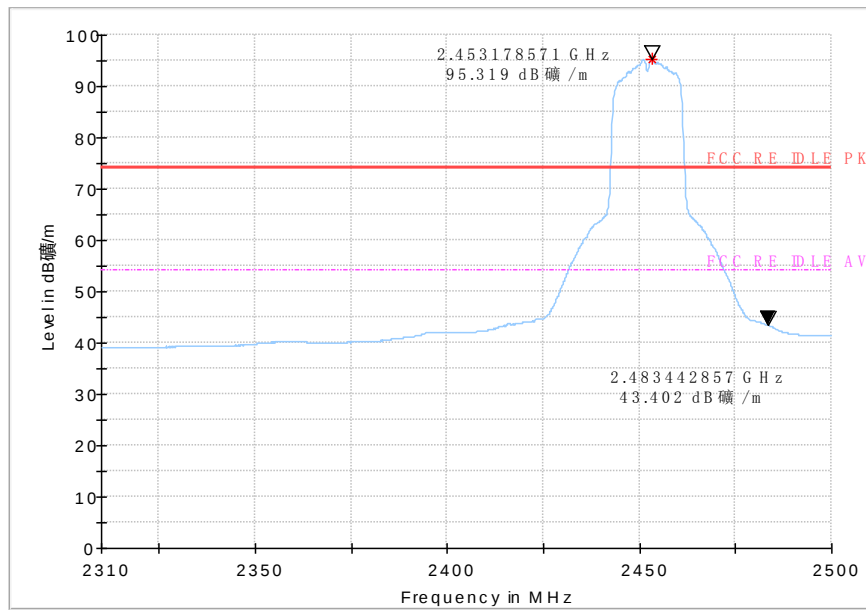
Fig.113 Radiated emission (Power): 802.11n (40M) , high channel
