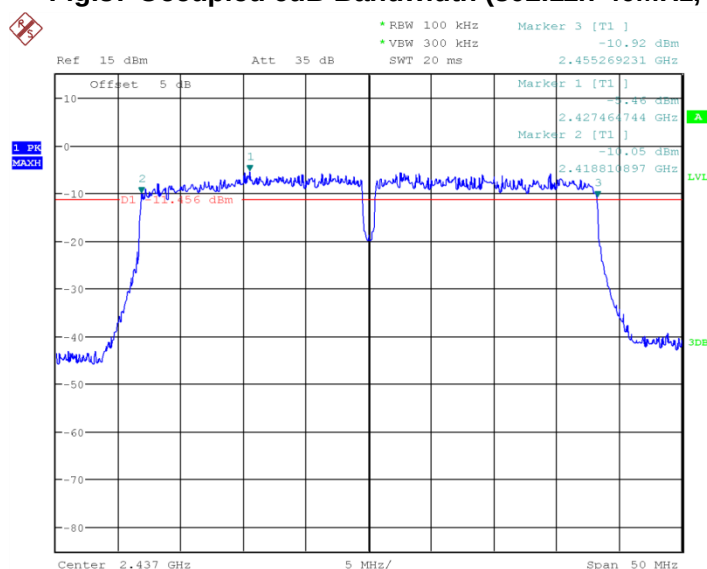
Fig.37 Occupied 6dB Bandwidth (802.11n-40MHz, Ch6)
