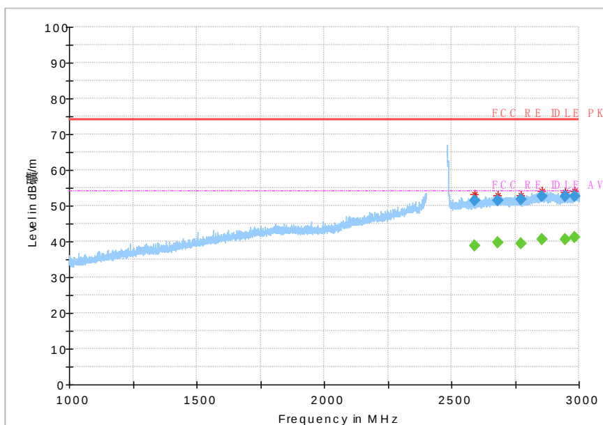
Fig.105 Radiated Spurious Emission (802.11g, Ch11, 1GHz~3GHz)
