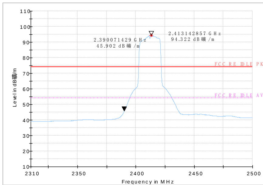
Fig.107 Radiated emission (Power): 802.11n, low channel
