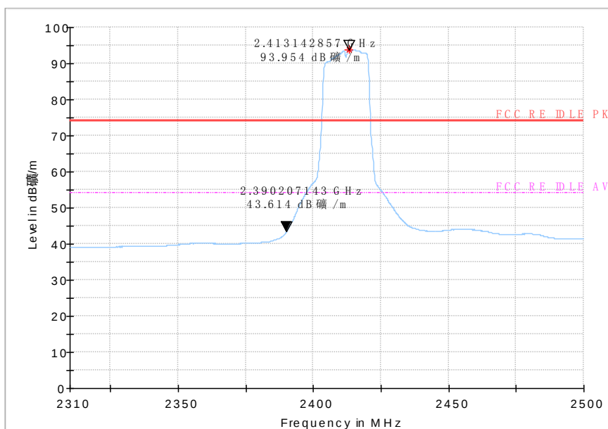
Fig.102 Radiated emission (Power): 802.11g, low channel
