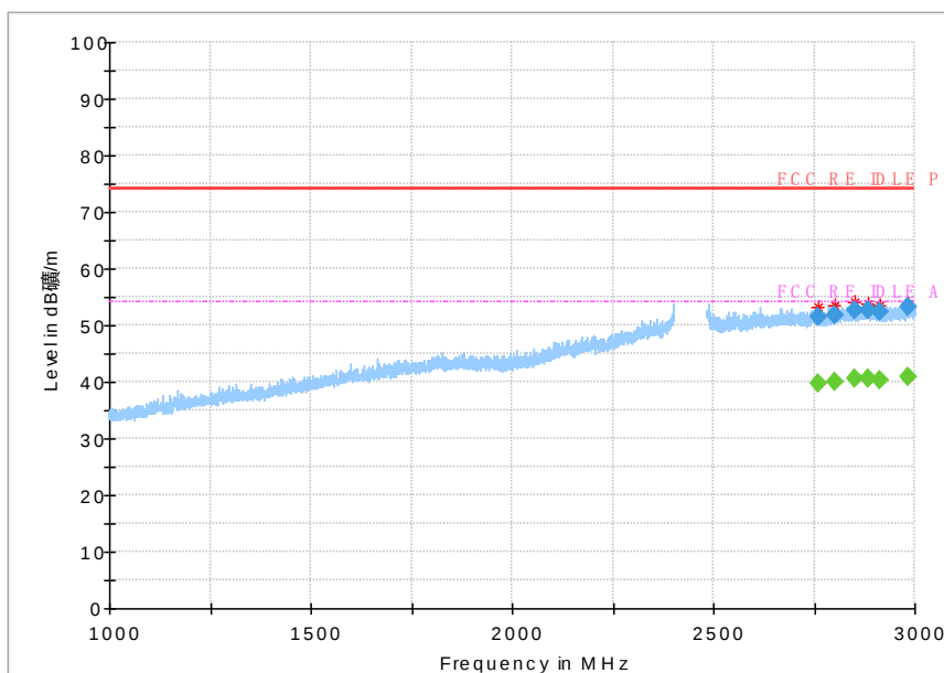
Fig.100 Radiated Spurious Emission (802.11b, Ch11, 1GHz~3GHz)
