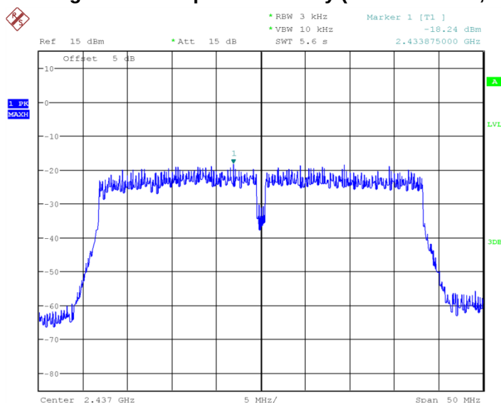
Fig.17 Power Spectral Density (802.1n-40MHz,Ch6)
