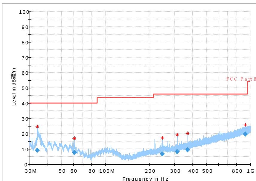
Fig.99 Radiated Spurious Emission (802.11b, Ch11, 30MHz~1GHz)
