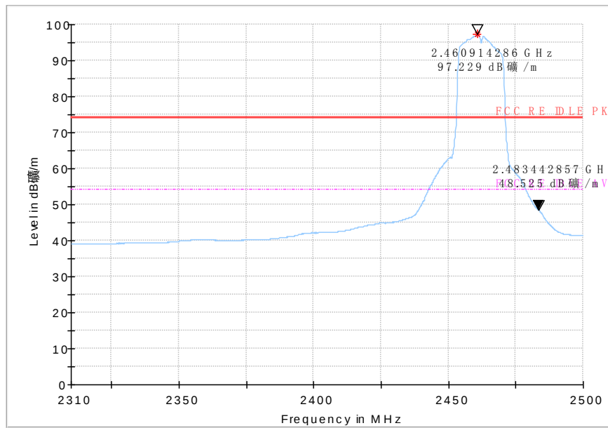
Fig.103 Radiated emission (Power): 802.11g, high channel
