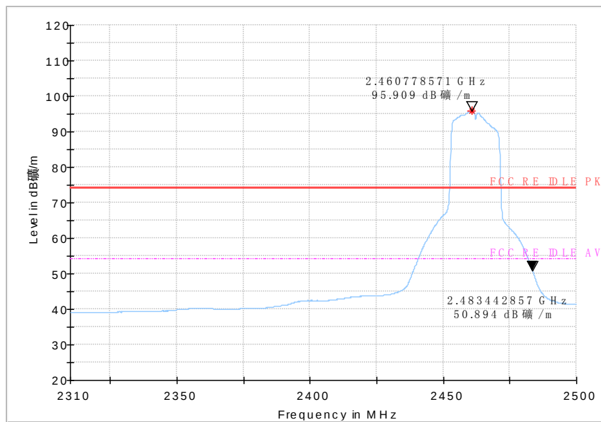
Fig.108 Radiated emission (Power): 802.11n, high channel
