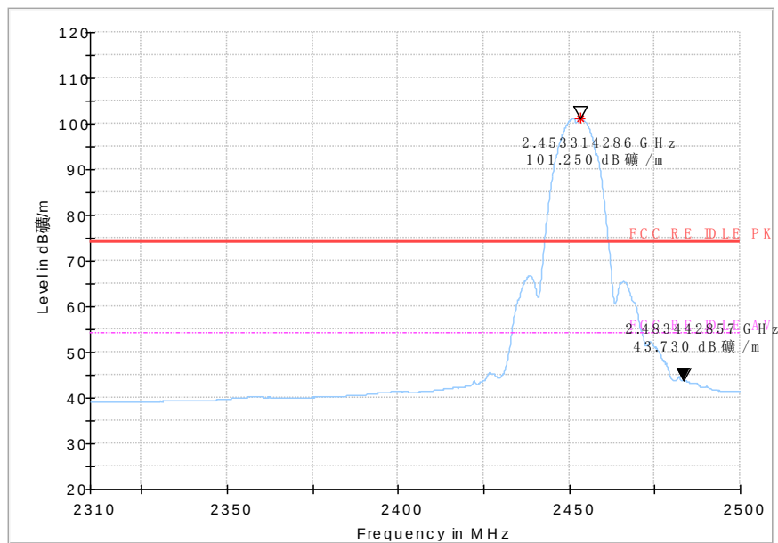
Fig.98 Radiated emission (Power): 802.11b, high channel
