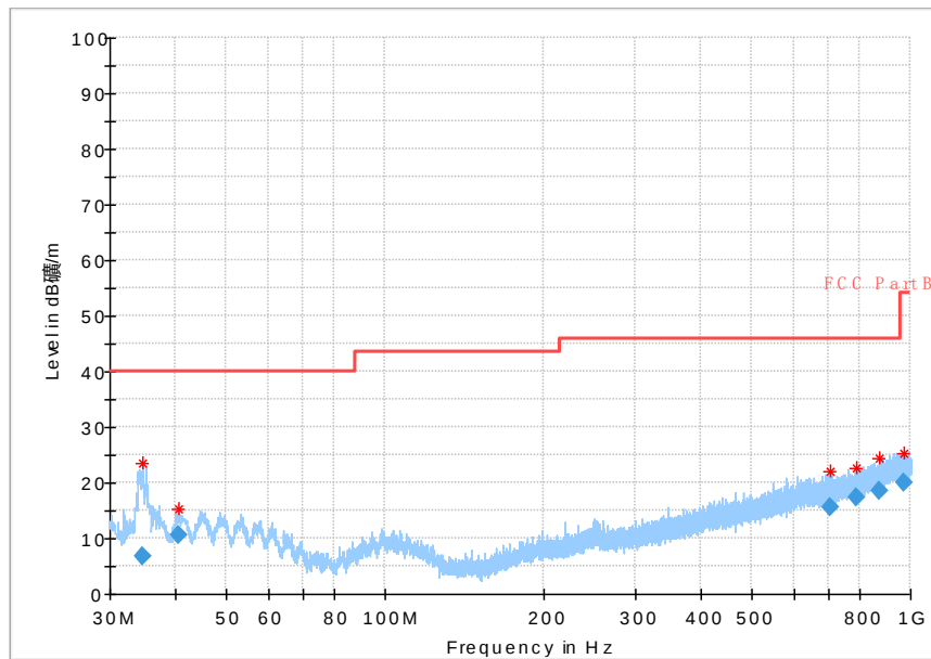
Fig.109 Radiated Spurious Emission (802.11 n-20MHz,Ch11,30MHz~1GHz)
