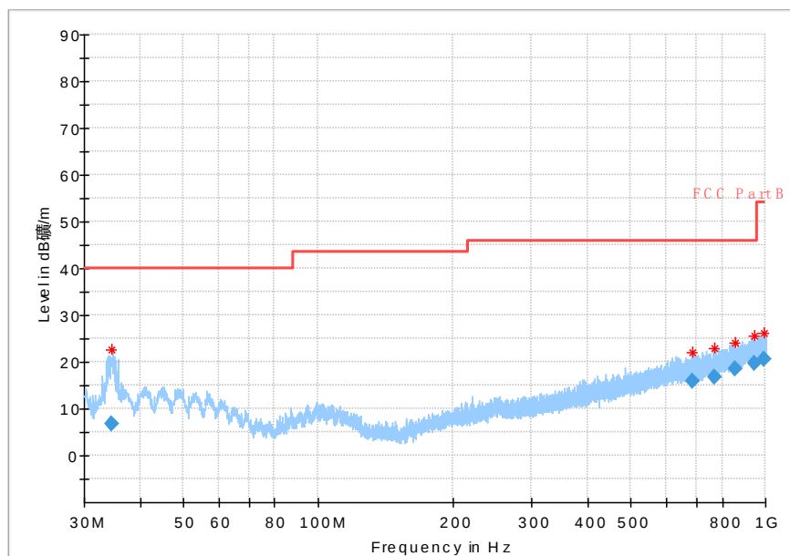
Fig.114 Radiated Spurious Emission (802.11 n-40MHz,Ch3,30MHz~1GHz)
