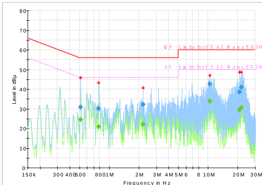
Fig.158 AC Powerline Conducted Emission
