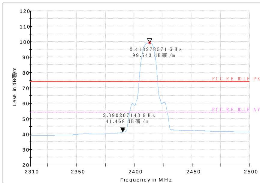
Fig.97 Radiated emission (Power): 802.11b, low channel
