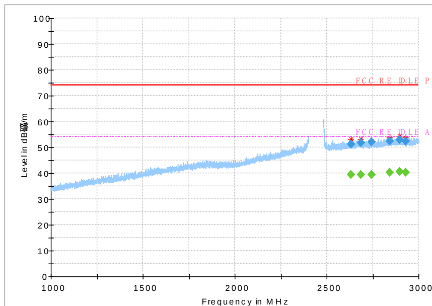
Fig.110 Radiated Spurious Emission (802.11 n-20MHz,Ch11,1GHz~3GHz)
