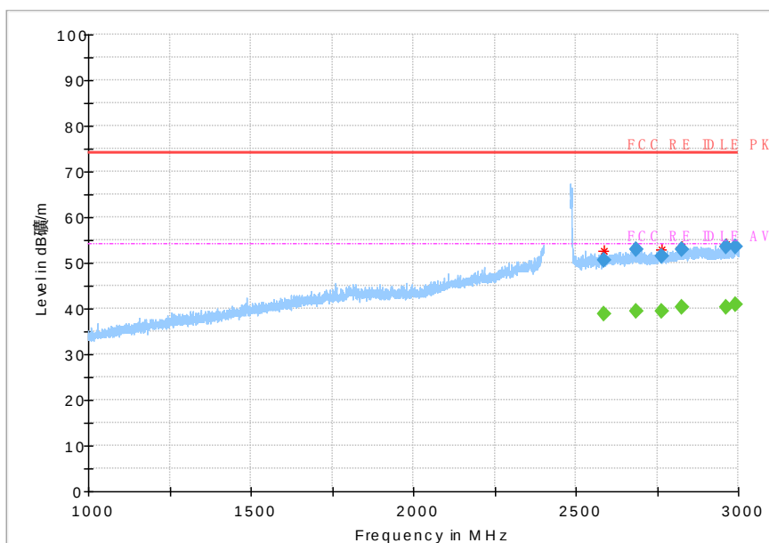
Fig.115 Radiated Spurious Emission (802.11 n-40MHz,Ch3,1GHz~3GHz)
