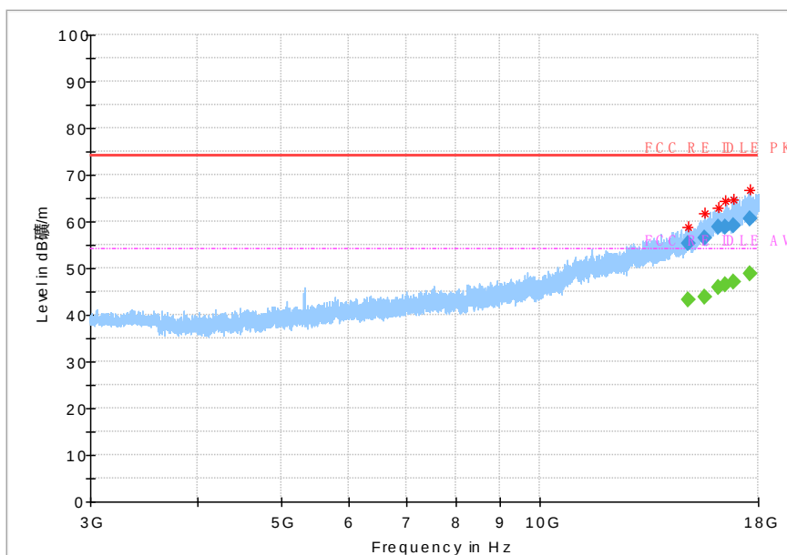
Fig.116 Radiated Spurious Emission (802.11 n-40MHz,Ch3,3GHz~18GHz)
