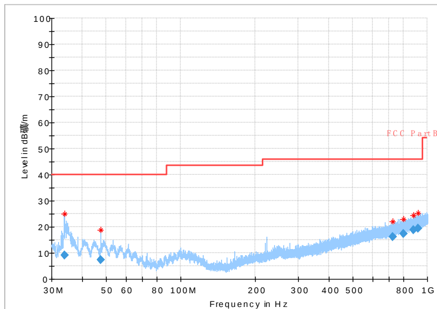
Fig.104 Radiated Spurious Emission (802.11g,Ch11,30MHz~1GHz)
