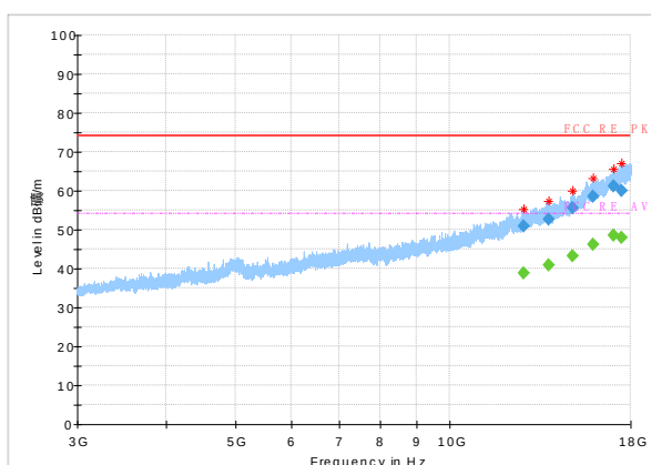
Radiated emission: Ch0, 3GHz~18GHz
