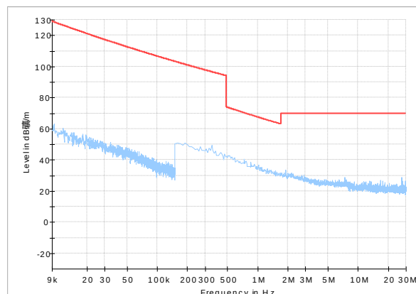
Radiated Spurious Emission (9kHz-30MHz)
