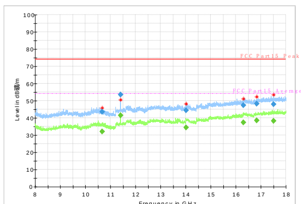
Radiated Spurious Emission (802.11a, ch140, 8GHz-18GHz)
