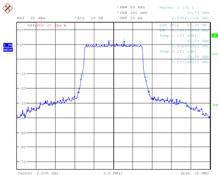
Fig.33 LTE band 7, 5MHz Bandwidth, QPSK (-26dBc BW)
