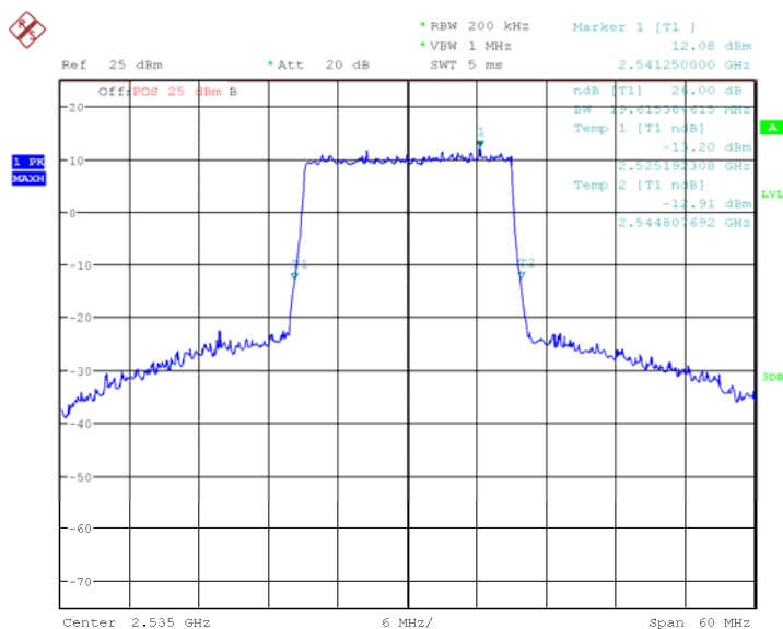
Fig.39 LTE band 7, 20MHz Bandwidth, QPSK (-26dBc BW)
