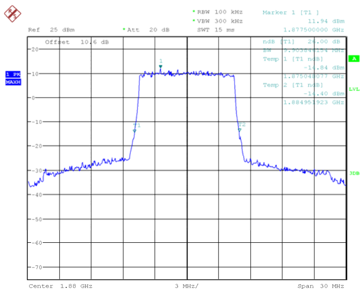
Fig.27 LTE band 2, 10MHz Bandwidth, QPSK (-26dBc BW)
