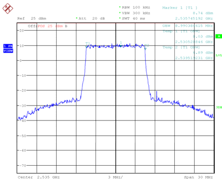
Fig.15 LTE band 7, 10MHz Bandwidth, QPSK (99% BW)
