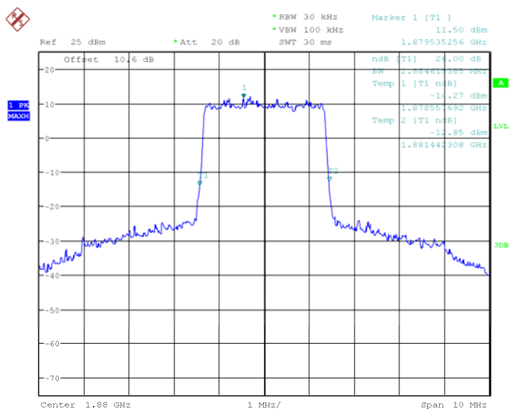
Fig.23 LTE band 2, 3MHz Bandwidth, QPSK (-26dBc BW)
