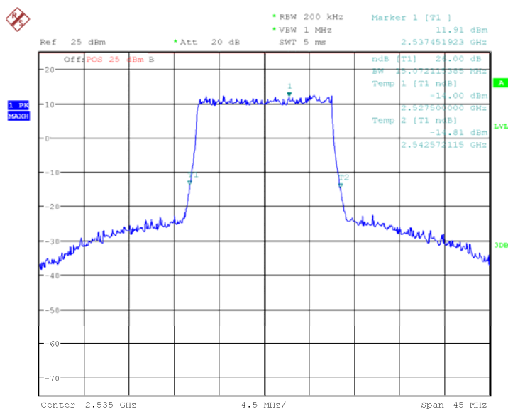
Fig.37 LTE band 7, 15MHz Bandwidth, QPSK (-26dBc BW)
