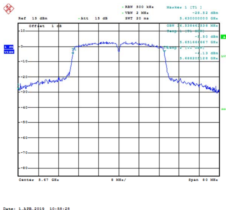
Fig. 75 99% Occupied Bandwidth (802.11n-HT40, 5670MHz)
