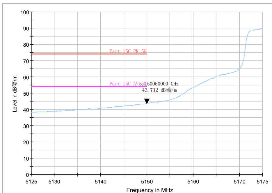
Fig. 88 Band Edges (802.11a, 5180MHz)
