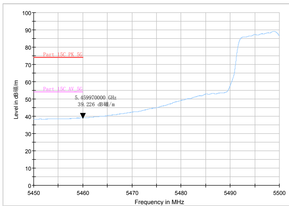
Fig. 90 Band Edges (802.11a, 5500MHz)
