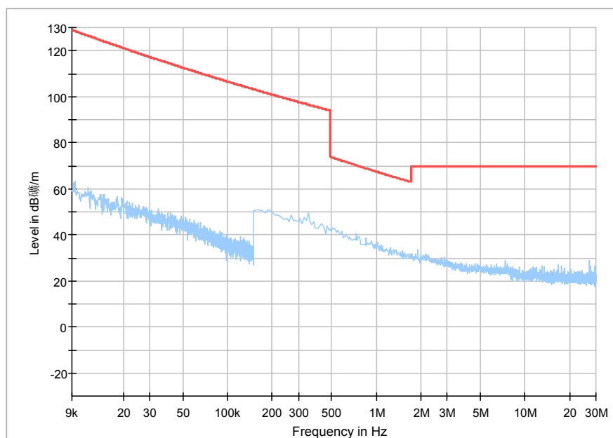
Fig. 115 Radiated Spurious Emission (9kHz-30MHz)
