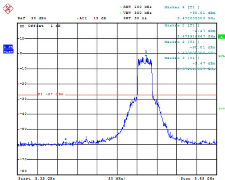
Fig. 86 Band Edges (802.11n-HT40, 5510MHz)
