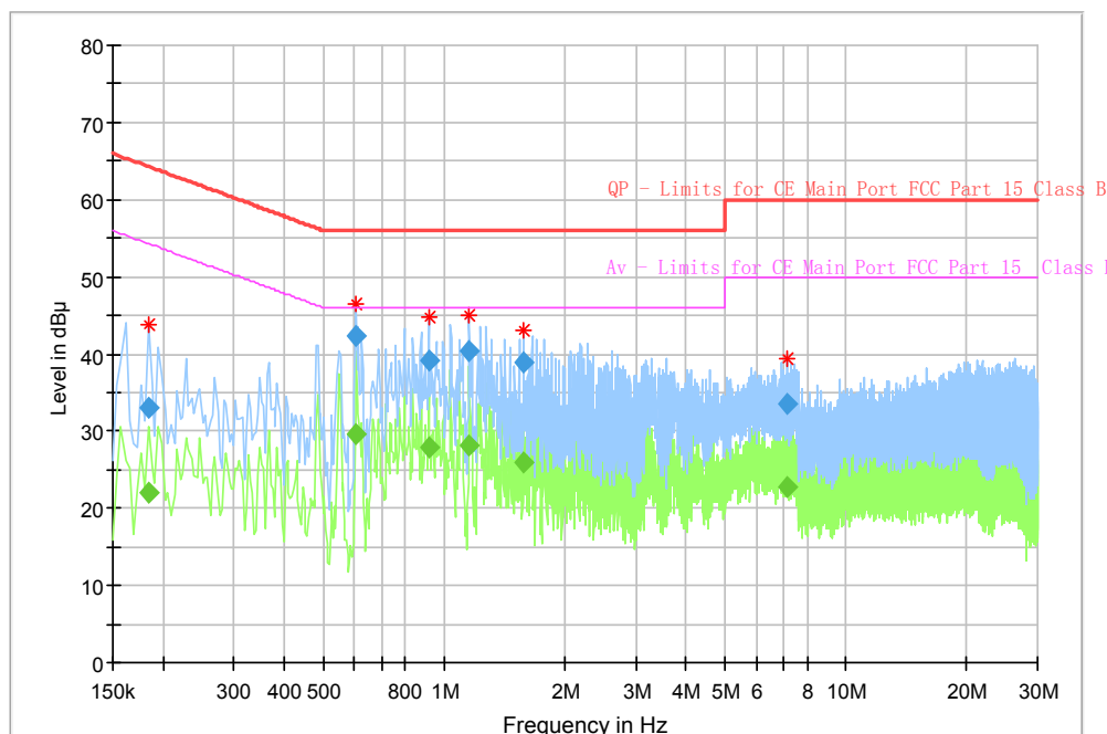
Fig. 116 Conducted Emission(802.11a, TX)
