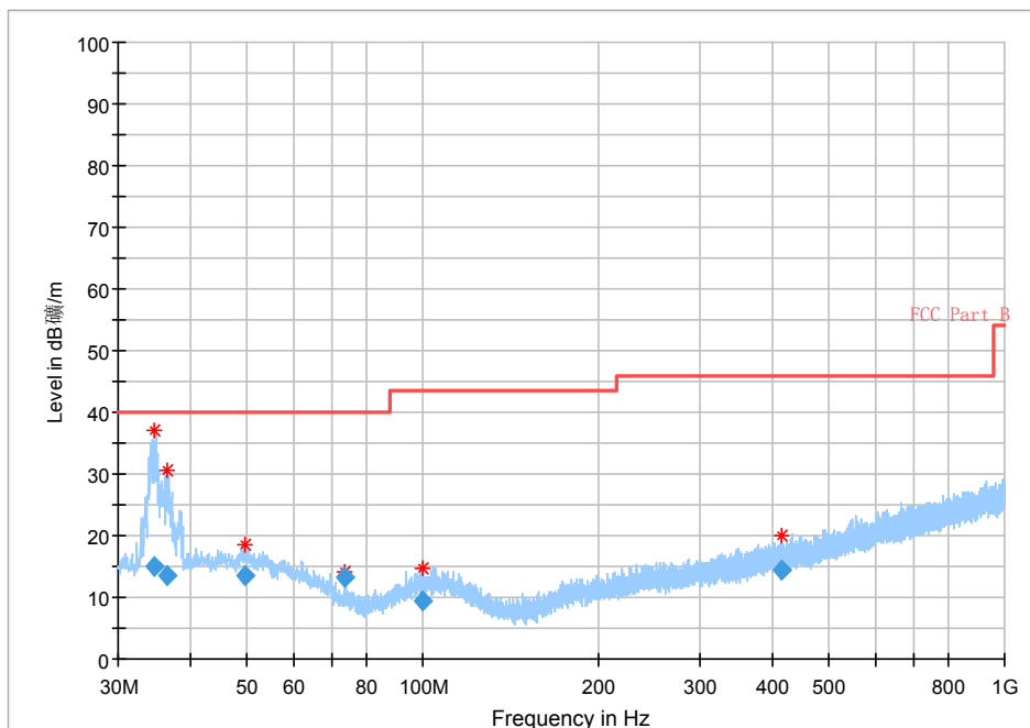
Fig 64. Radiated Spurious Emission (802.11g,Ch1, 30MHz~1GHz)
