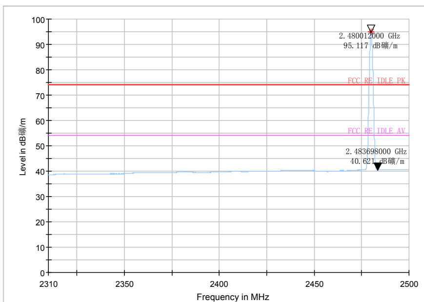
Fig.25 Bandedge:ch39
