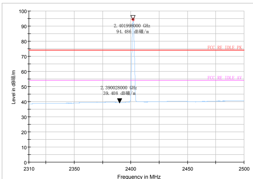
Fig.21 Bandedge:ch0
