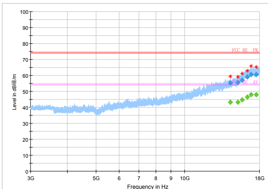
Fig.38 Radiated emission: \pi/4 DQPSK, Ch78, 3GHz~18GHz
