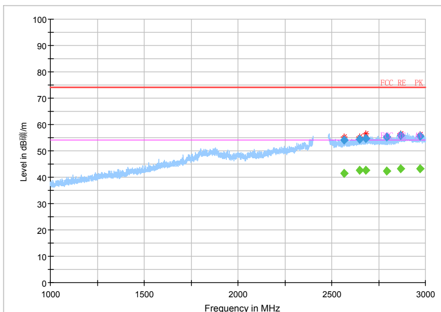
Fig.42 Radiated emission: 8DPSK, Ch78, 1GHz~3GHz
