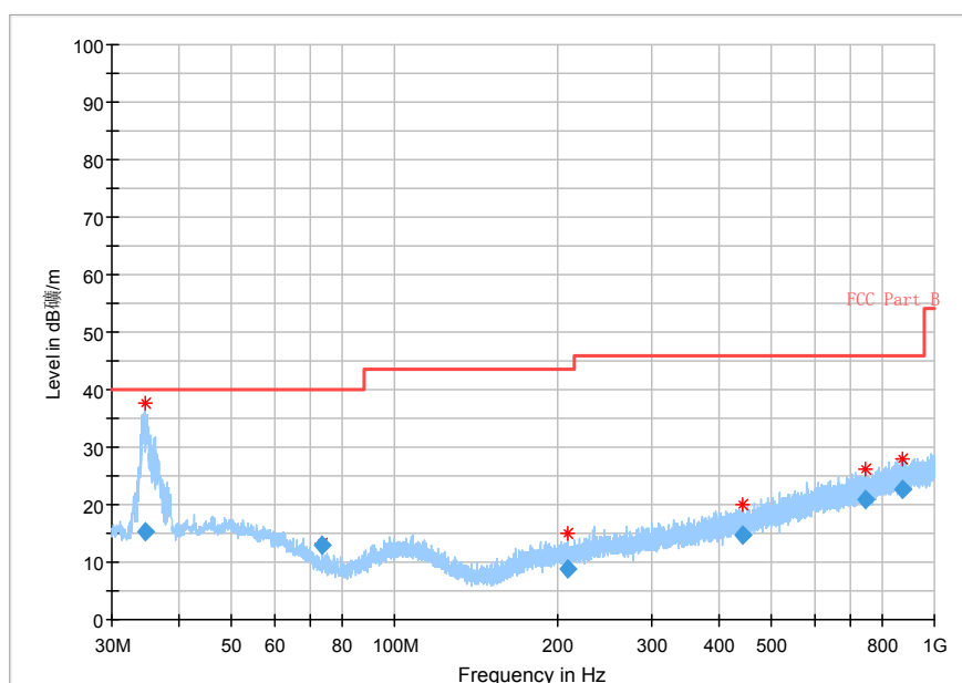
Fig.41 Radiated emission: 8DPSK, Ch78, 30MHz~1GHz
