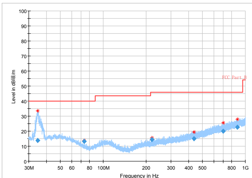
Fig.36 Radiated emission: \pi/4 DQPSK, Ch78, 30MHz~1GHz
