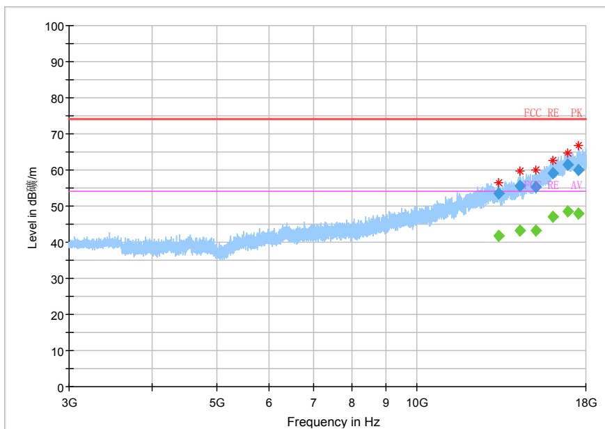
Fig.33 Radiated emission: GFSK, Ch78, 3GHz~18GHz
