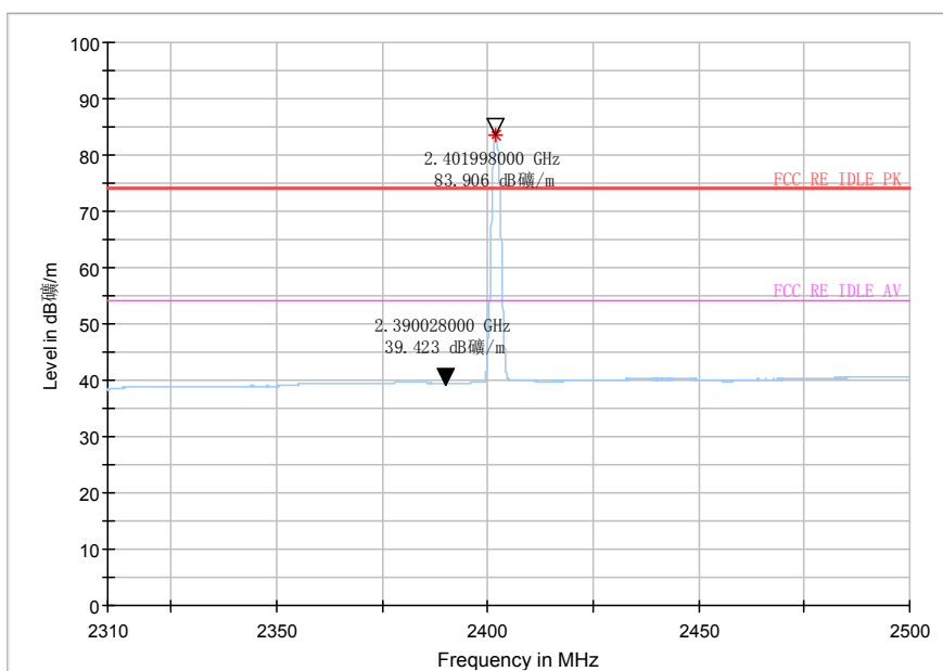
Fig.44 Bandedge (Low): 8DPSK, low channel
