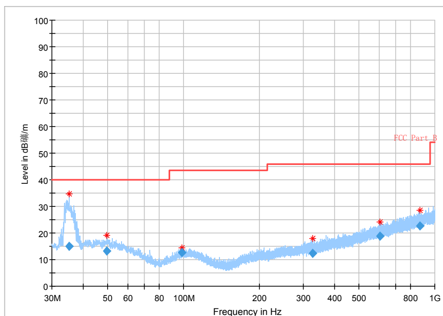
Fig.31 Radiated emission: GFSK, Ch78, 30MHz~1GHz
