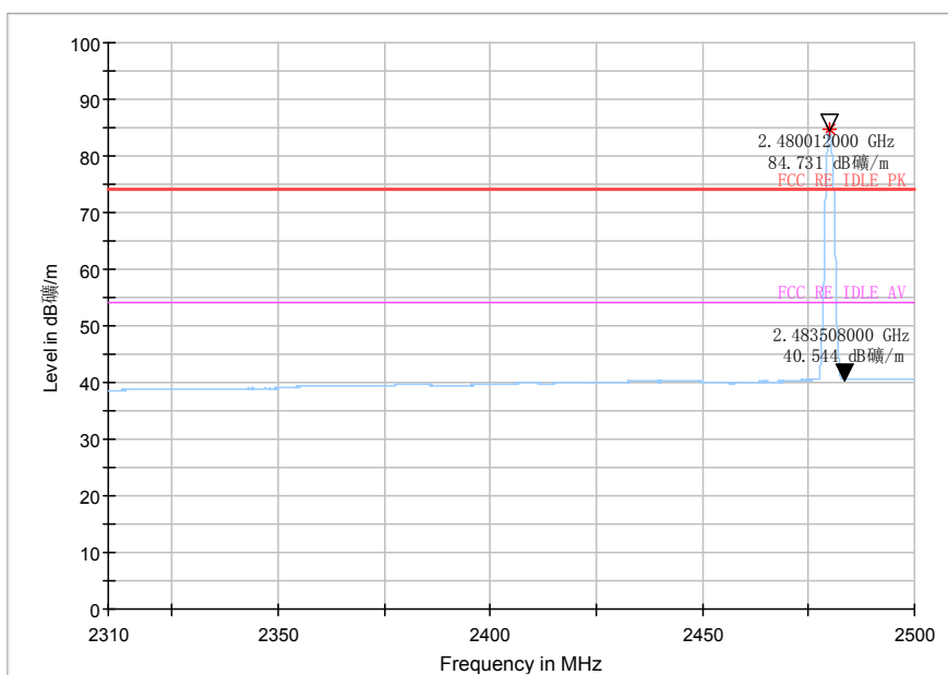
Fig.45 Bandedge (High): 8DPSK, high channel
