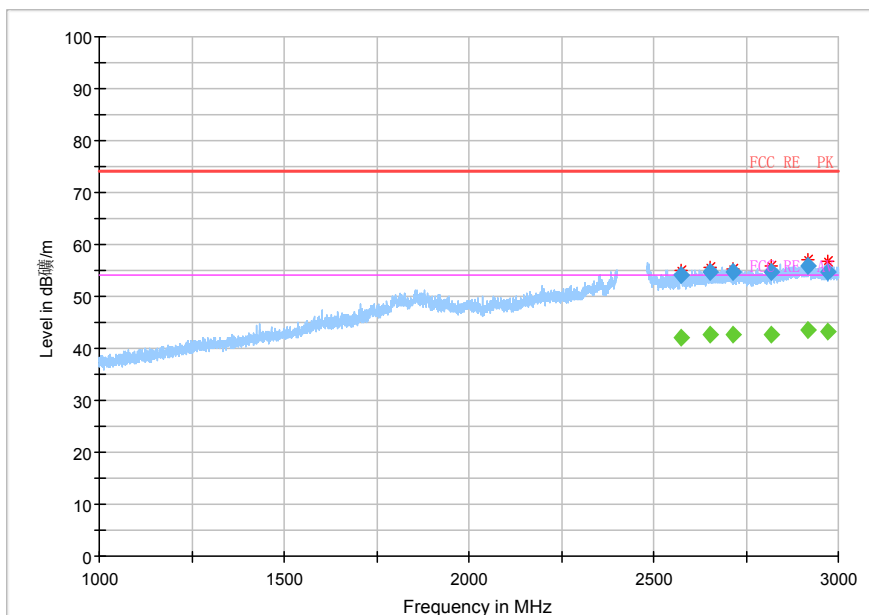
Fig.37 Radiated emission: \pi/4 DQPSK, Ch78, 1GHz~3GHz
