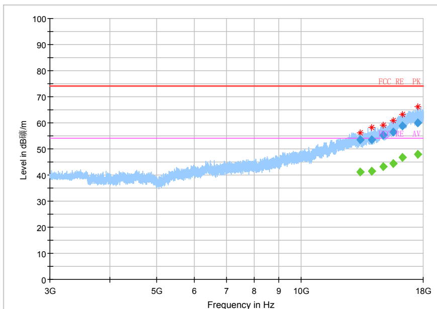
Fig.43 Radiated emission: 8DPSK, Ch78, 3GHz~18GHz
