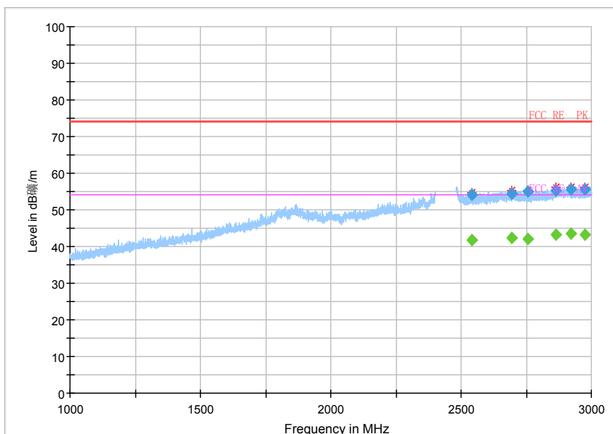
Fig.32 Radiated emission: GFSK, Ch78, 1GHz~3GHz
