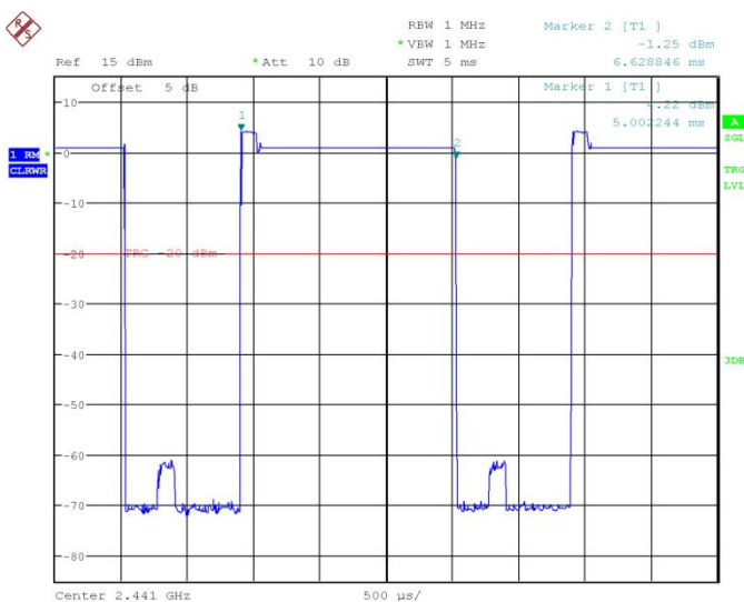
Fig.68 Number of Transmissions Measurement: Ch39, Packet 3-DH1
