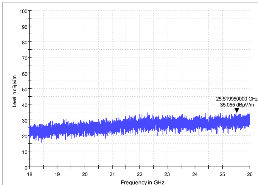
Radiated emission (Power):18G~26G
