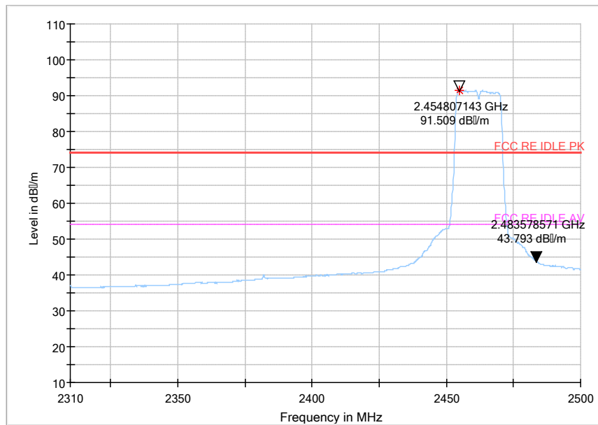
Fig 49. Radiated emission (Power): 802.11g, high channel
