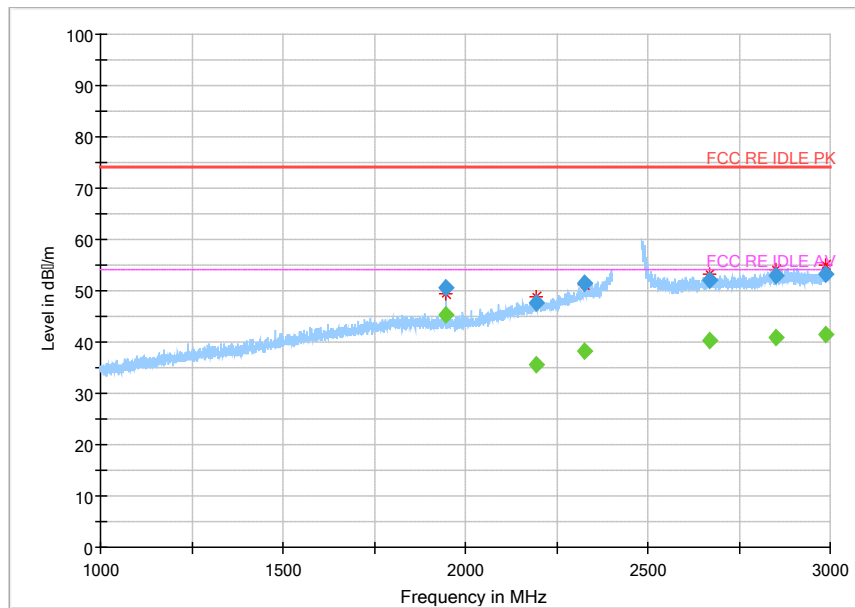
Fig 51. Radiated Spurious Emission (802.11g, Ch1, 1GHz~3GHz)
