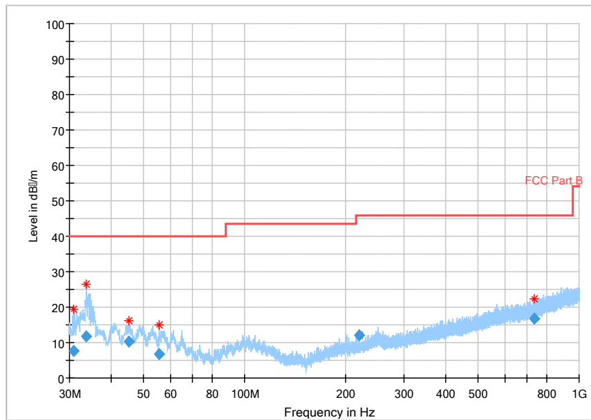
Fig 55. Radiated Spurious Emission (802.11 n-20MHz,Ch1,30MHz~1GHz)
