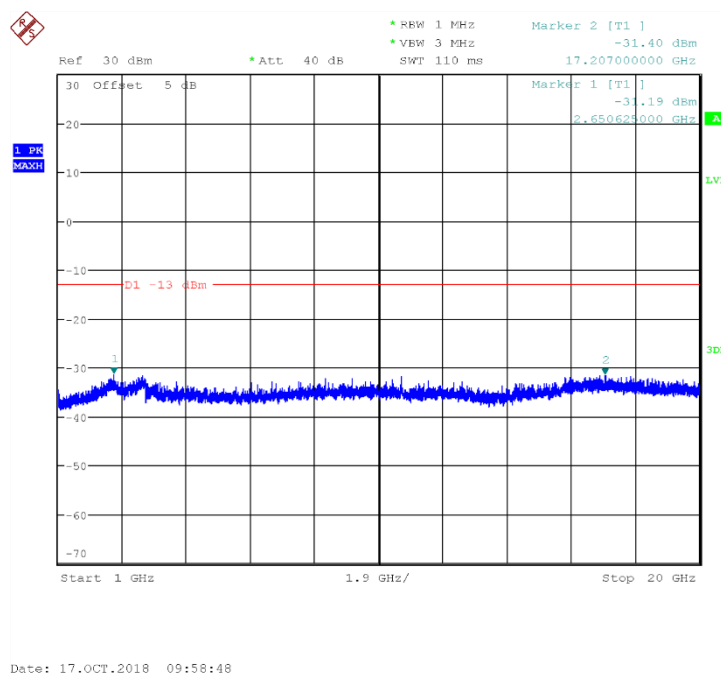
Fig.88 Channel 4233: 1GHz~20GHz
