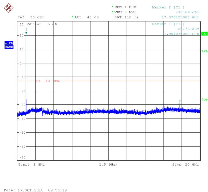
Fig.82 Channel 9538: 1GHz~20GHz
