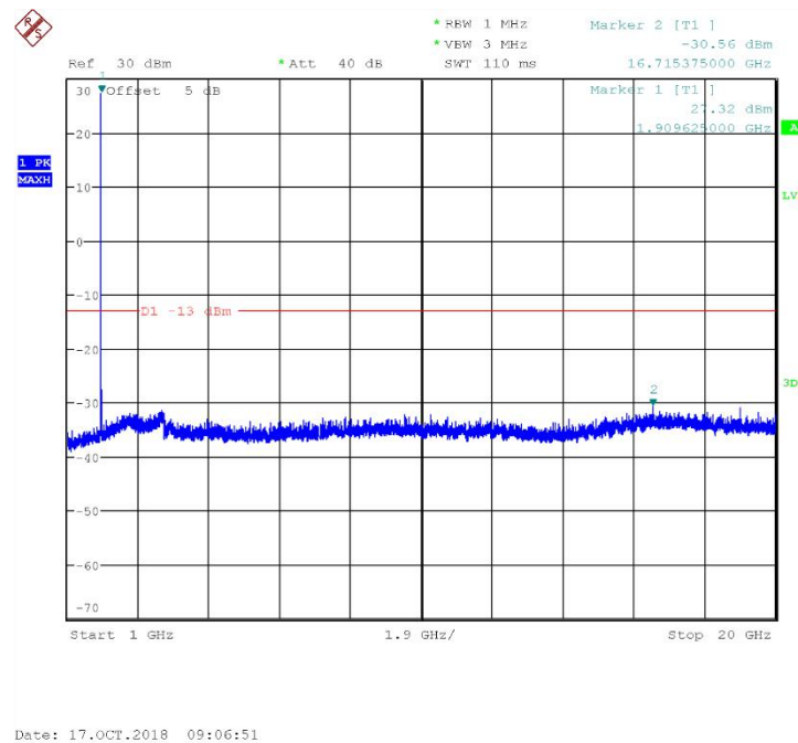
Fig.76 Channel 810: 1GHz~20GHz
