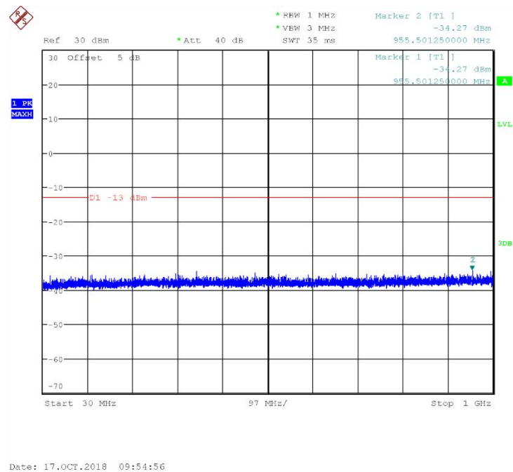
Fig.81 Channel 9538: 30MHz~1GHz
