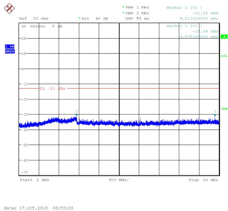
Fig.70 Channel 251: 1GHz~10GHz
