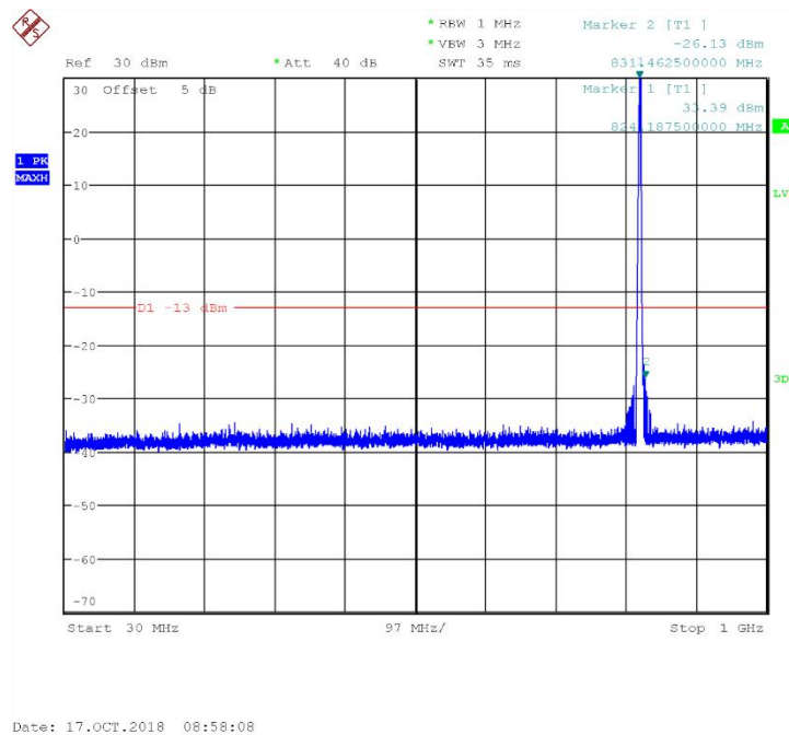
Fig.65 Channel 128: 30MHz~1GHz
