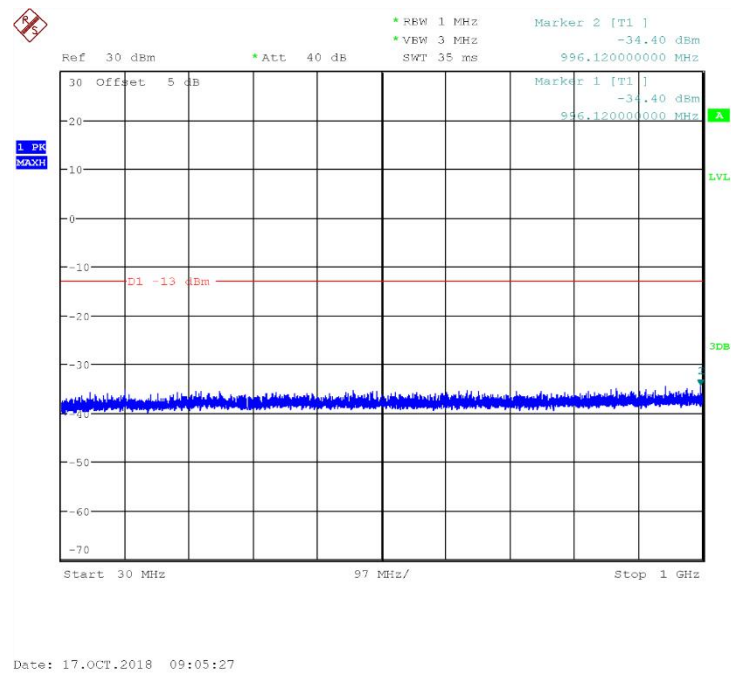
Fig.71 Channel 512: 30MHz~1GHz
