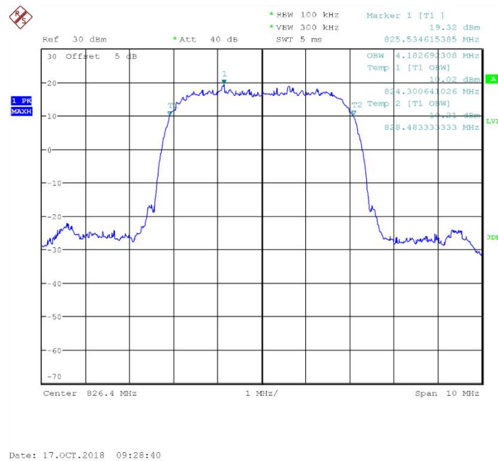
Fig.23 Channel 4132-Occupied Bandwidth (99%)
