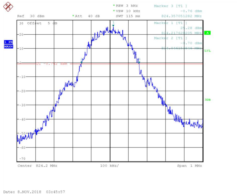
Fig.26 Channel 128- Emission Bandwidth (-26dBc BW)
