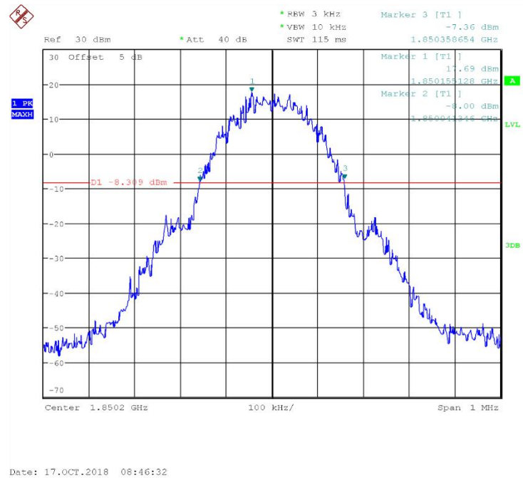
Fig.38 Channel 512- Emission Bandwidth (-26dBc BW)
