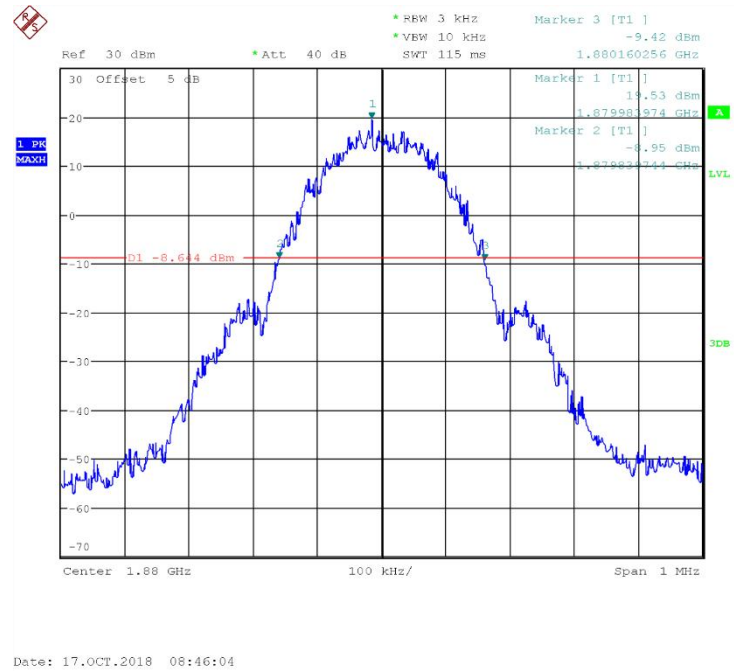
Fig.37 Channel 661- Emission Bandwidth (-26dBc BW)
