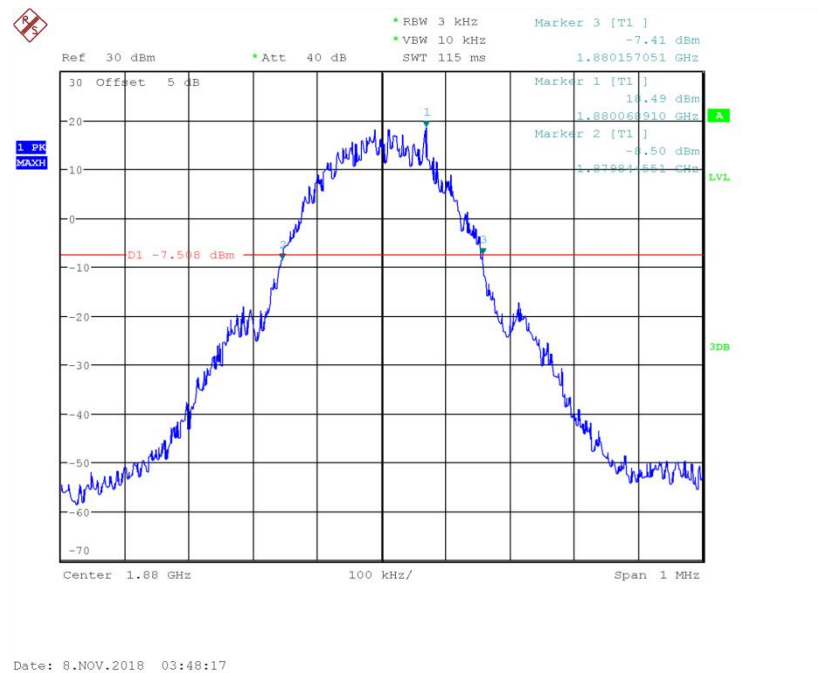
Fig.34 Channel 661- Emission Bandwidth (-26dBc BW)
