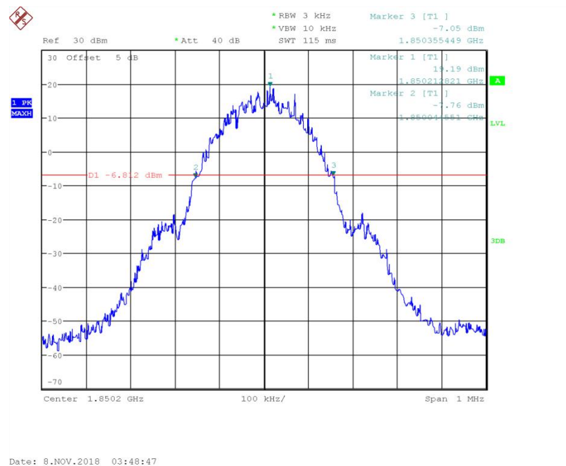
Fig.35 Channel 512- Emission Bandwidth (-26dBc BW)
