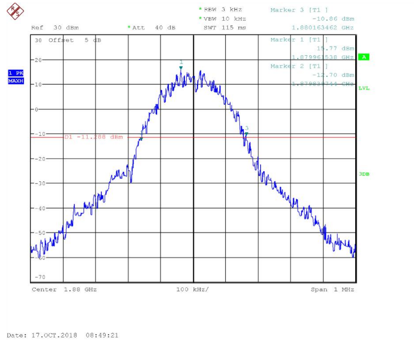
Fig.40 Channel 661- Emission Bandwidth (-26dBc BW)
