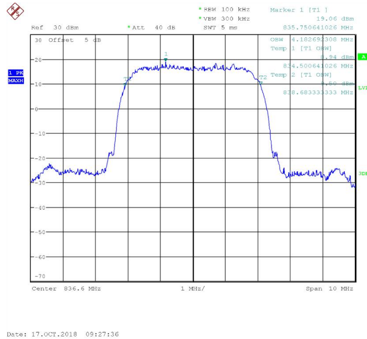
Fig.22 Channel 4183-Occupied Bandwidth (99%)
