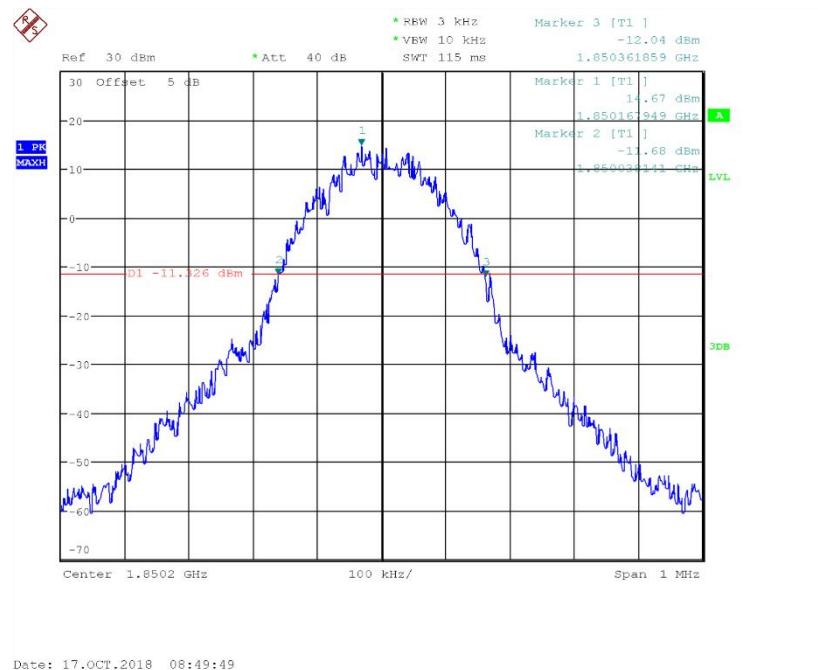
Fig.41 Channel 512- Emission Bandwidth (-26dBc BW)
