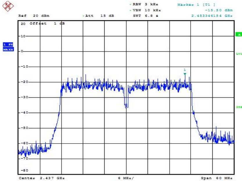
Fig 11. Power Spectral Density (802.11n-40MHz, Ch6)
