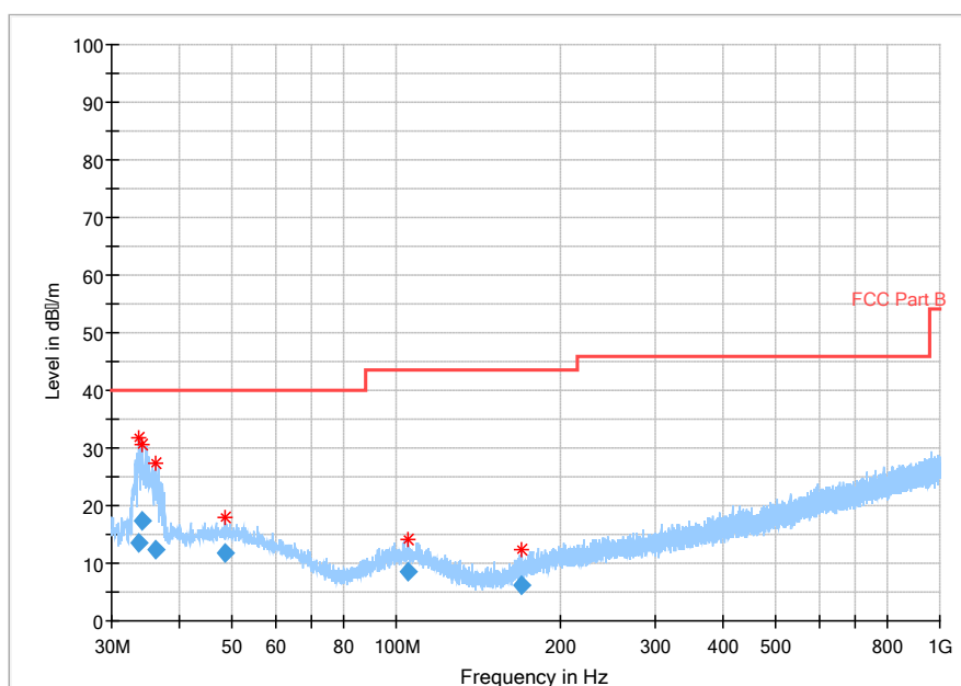
Fig.40 Radiated emission: GFSK, Ch78, 30MHz~1GHz
