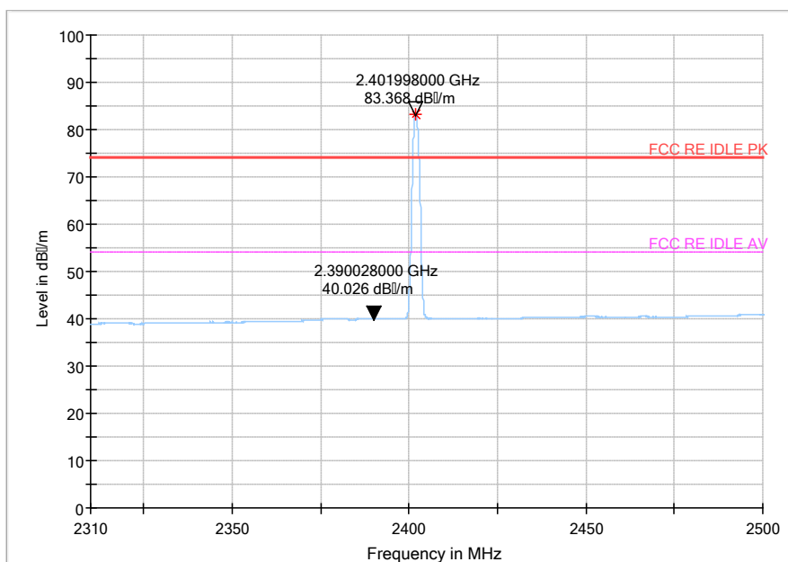
Fig.53 Radiated emission (Low): 8DPSK, low channel
