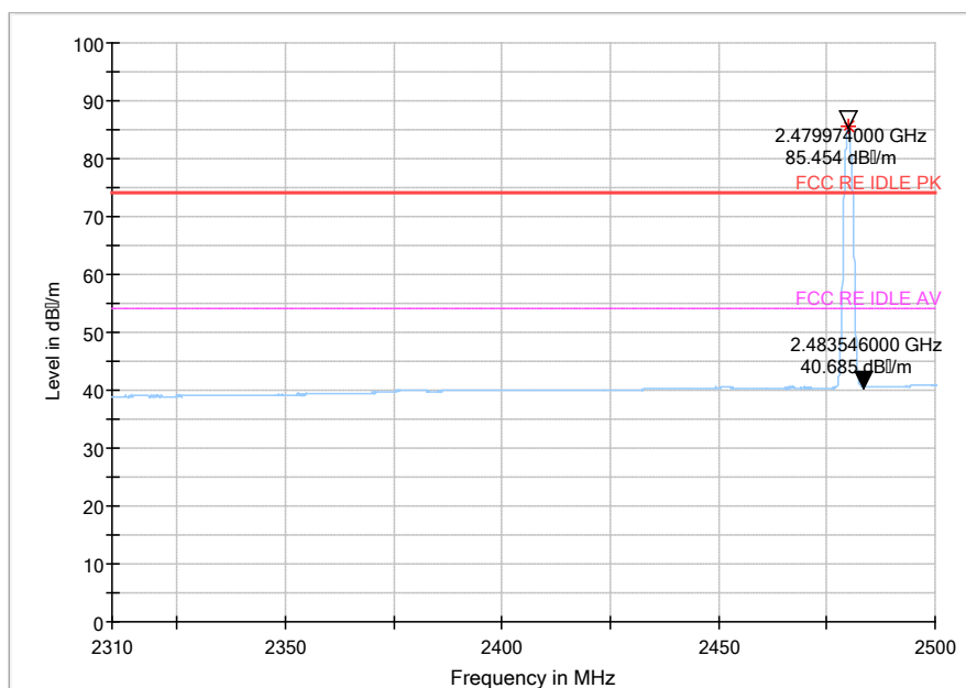
Fig.54 Radiated emission (High): 8DPSK, high channel
