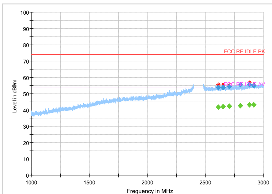
Fig.41 Radiated emission: GFSK, Ch78, 1GHz~3GHz
