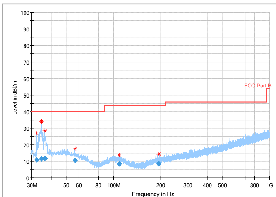
Fig.45 Radiated emission: \pi/4 DQPSK, Ch78, 30MHz~1GHz
