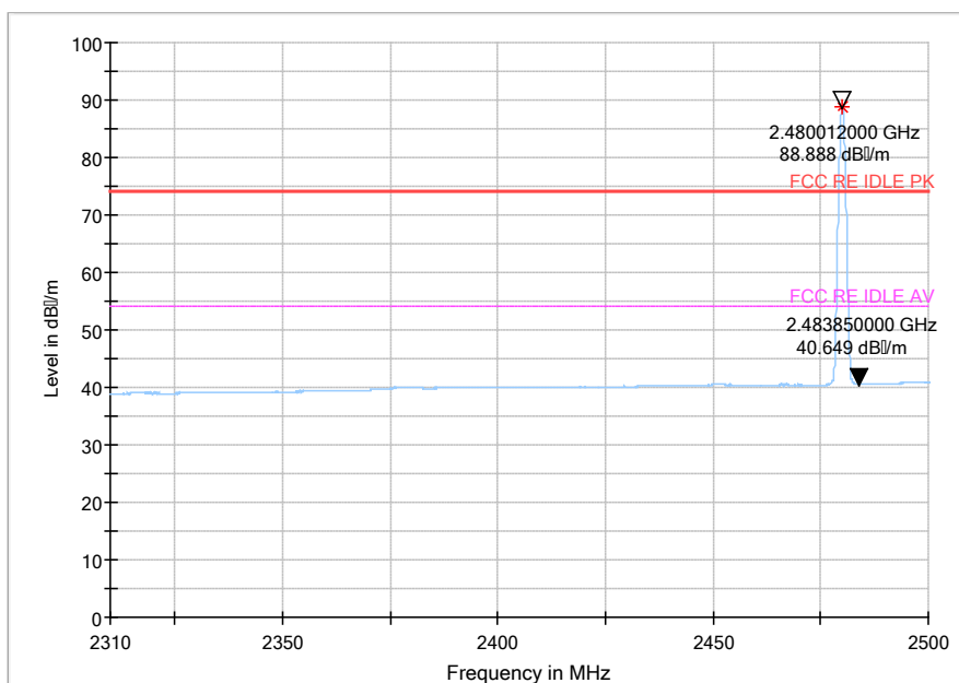
Fig.44 Radiated emission (High): GFSK, high channel
