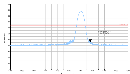
3DH5-Channel 78: Peak
