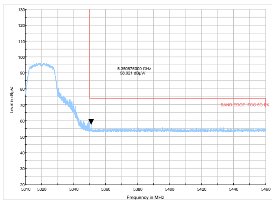
802.11a-Channel 64: Average
