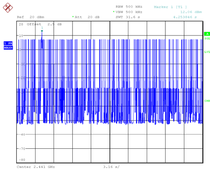
Fig.63 Time of occupancy (Dwell Time): Ch39,Packet 2-DH3
