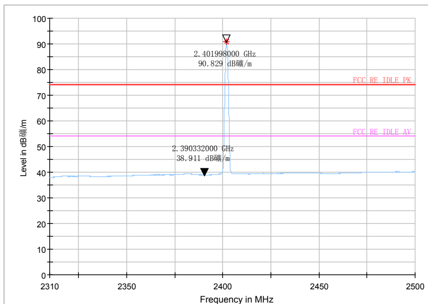
Fig.43 Bandedge (Low): GFSK, low channel
