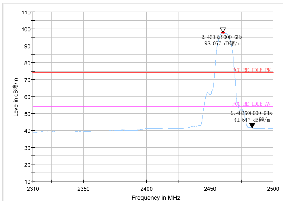
Fig 58. Bandedge: 802.11b, high channel
