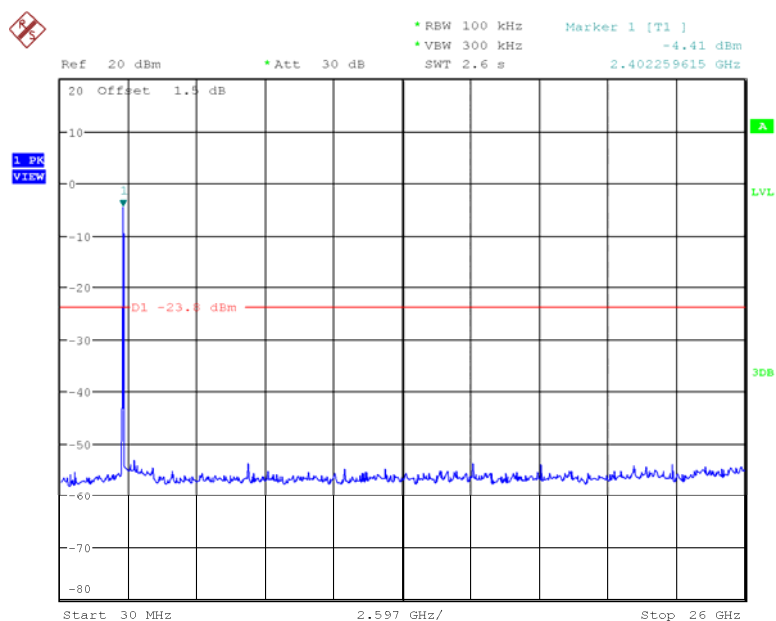
Fig 51. Conducted Spurious Emission (802.11n-40MHz, Ch3)
