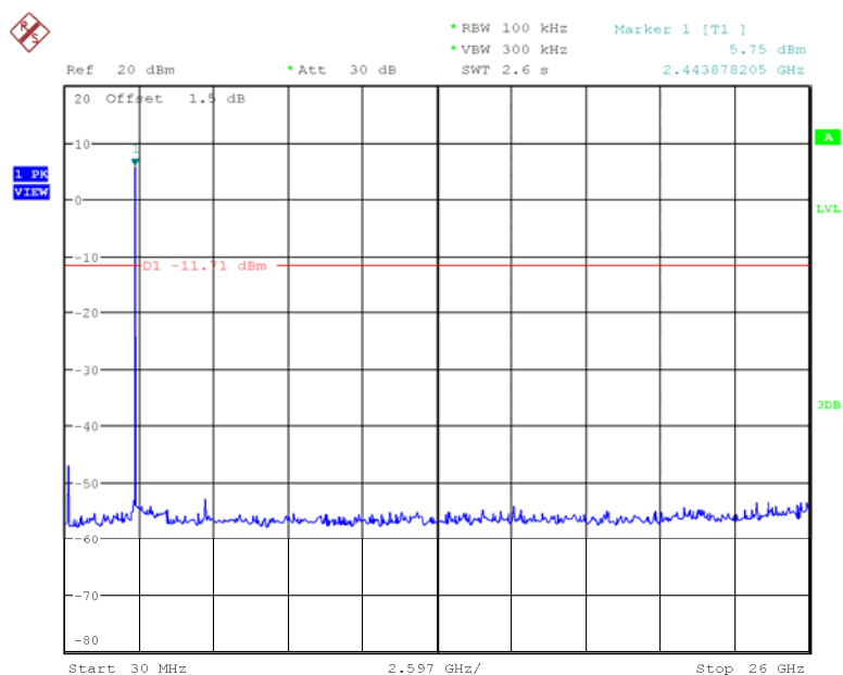
Fig 37. Conducted Spurious Emission (802.11b, Ch11)
