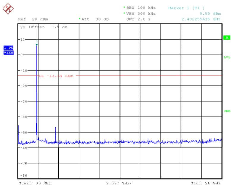
Fig 33. Conducted Spurious Emission (802.11b, Ch1)
