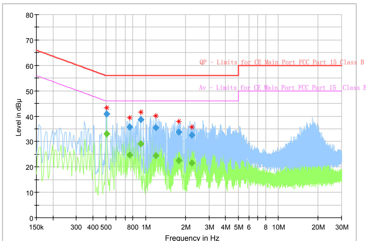
Fig 77. AC Powerline Conducted Emission
