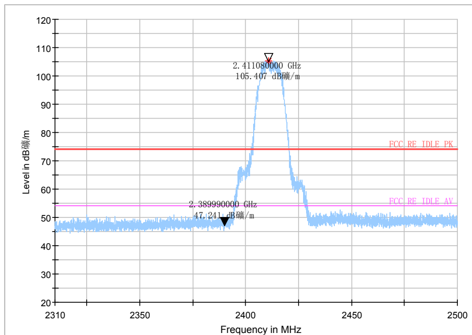
Peak detector
