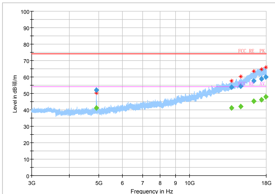
Fig 61. Radiated Spurious Emission (802.11b, Ch11, 3GHz~18GHz)
