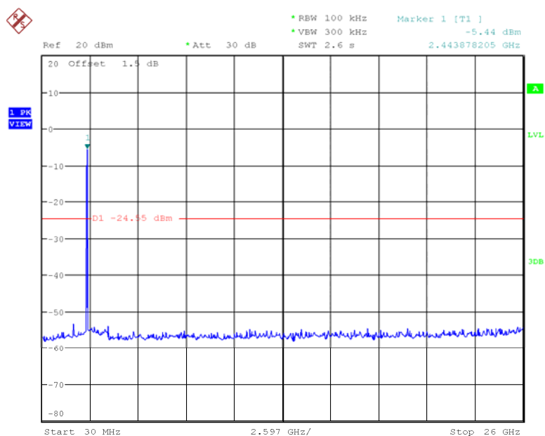
Fig 55. Conducted Spurious Emission (802.11n-40MHz, Ch9)
