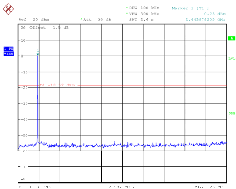
Fig 49. Conducted Spurious Emission (802.11n-20MHz, Ch11)
