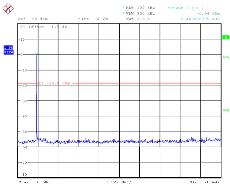
Fig 43. Conducted Spurious Emission (802.11g, Ch11)
