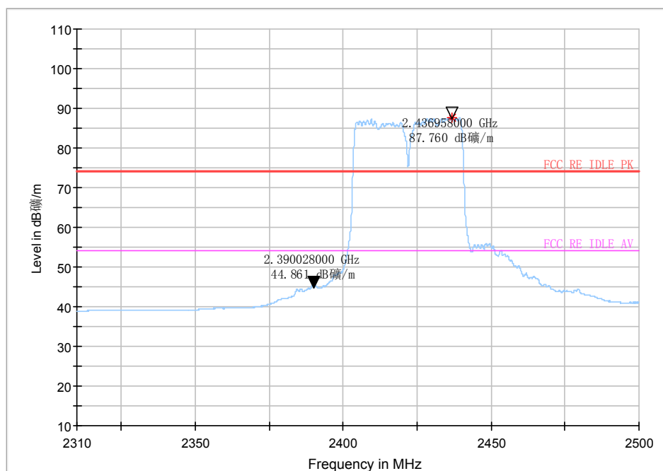
Average detector
