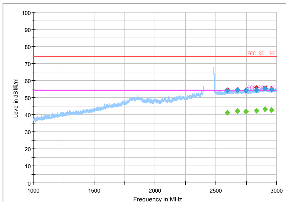
Fig 70. Radiated Spurious Emission (802.11 n-20MHz,Ch11, 1GHz~3GHz)
