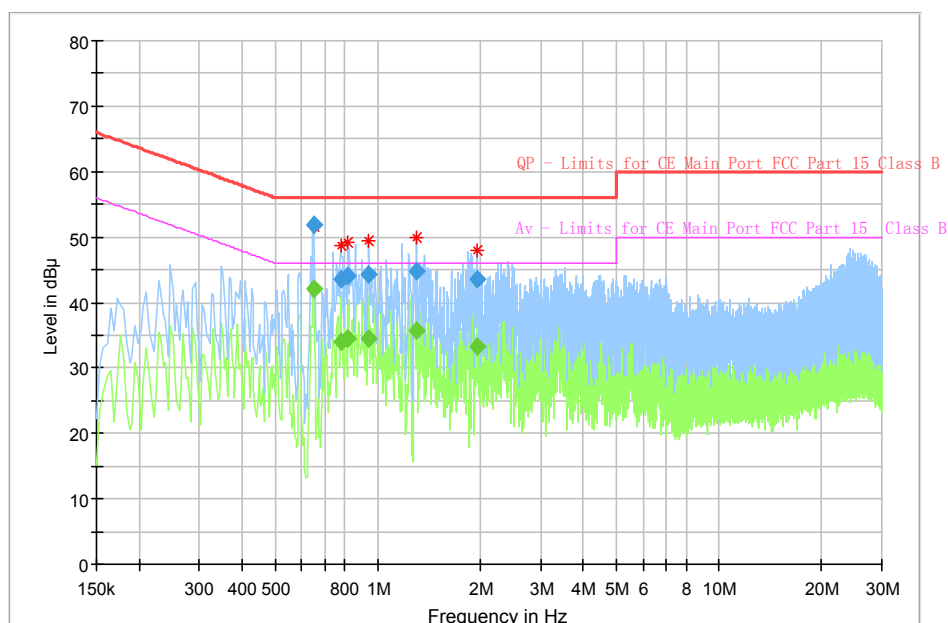
Fig.26 AC Powerline Conducted Emission
