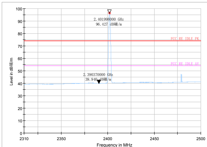
Fig.21 Bandedge:ch0
