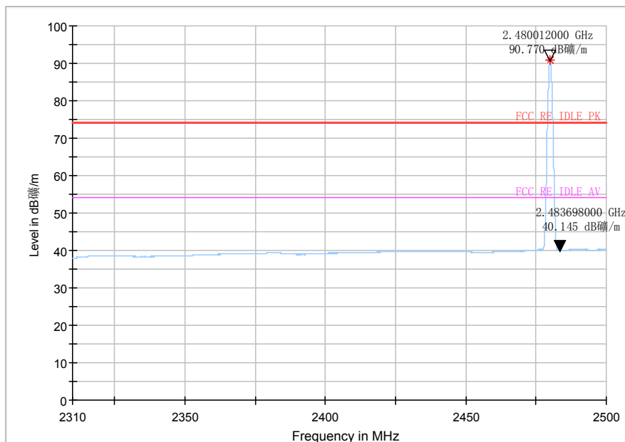
Fig.25 Bandedge:ch39
