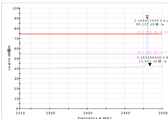
Radiated emission (High): GFSK, high channel
