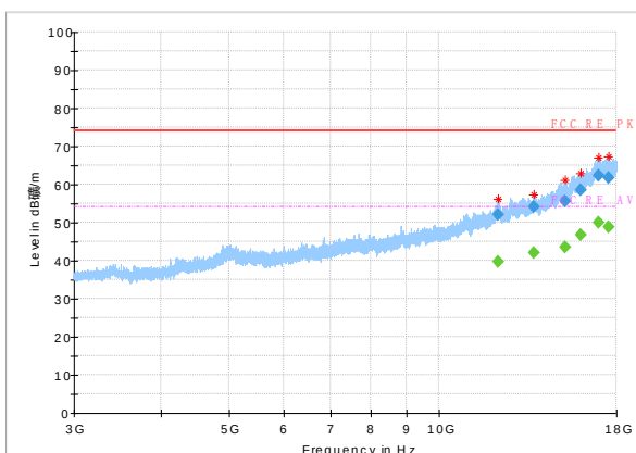
Radiated emission (High): GFSK, high channel
