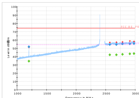
Radiated emission (Low): GFSK, low channel
