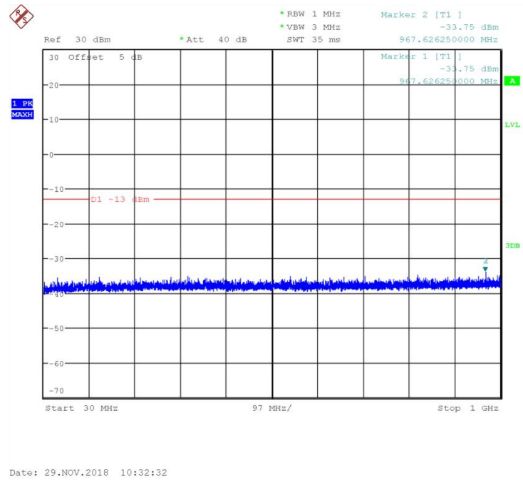
Fig.23 Channel 512: 30MHz~1GHz
