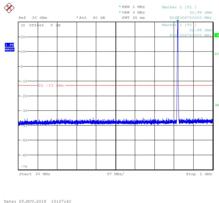
Fig.17 Channel 128: 30MHz~1GHz
