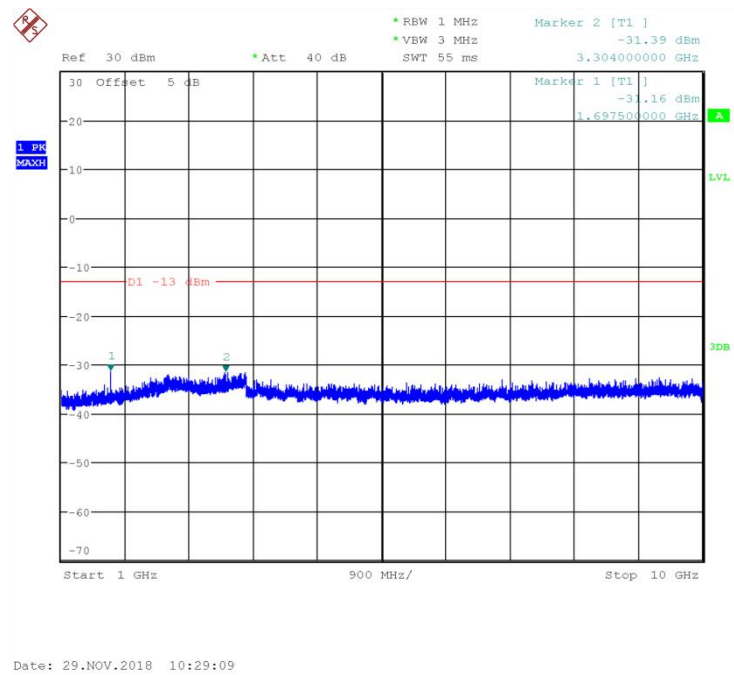
Fig.22 Channel 251: 1GHz~10GHz
