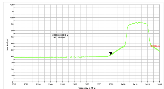
802.11g-Channel 1 Average
