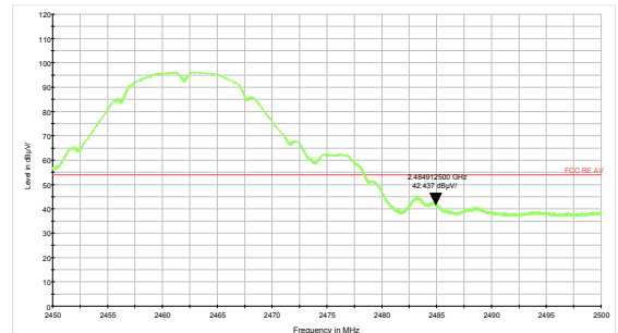
802.11b-Channel 11 Average
