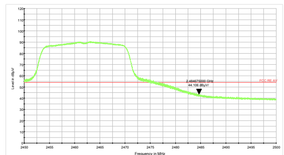
802.11g-Channel 11 Average
