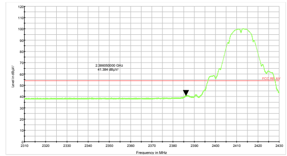
802.11b-Channel 1 Average
