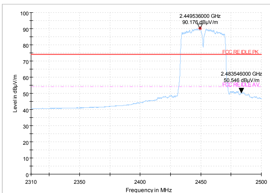
Fig.113 Radiated emission (Power): 802.11n (40M) , high channel
