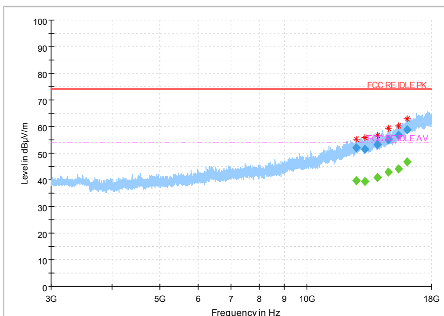
Fig.116 Radiated Spurious Emission (802.11 n-40MHz, Ch9, 3GHz~18GHz)
