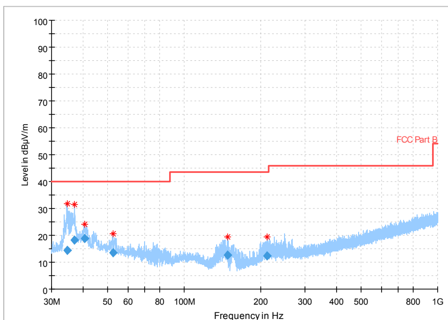
Fig.104 Radiated Spurious Emission (802.11g,Ch11,30MHz~1GHz)
