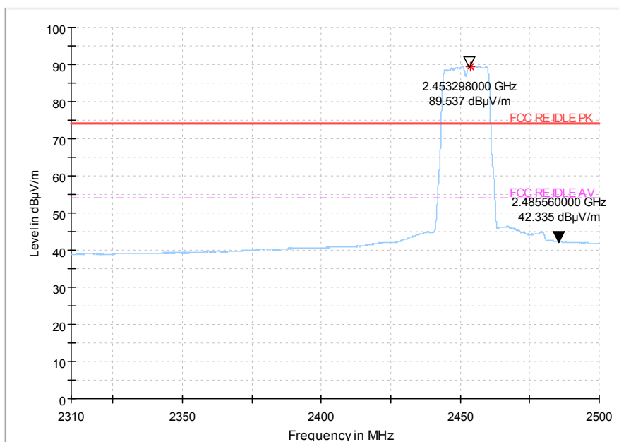
Fig.103 Radiated emission (Power): 802.11g, high channel
