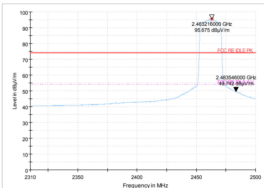
Fig.108 Radiated emission (Power): 802.11n, high channel
