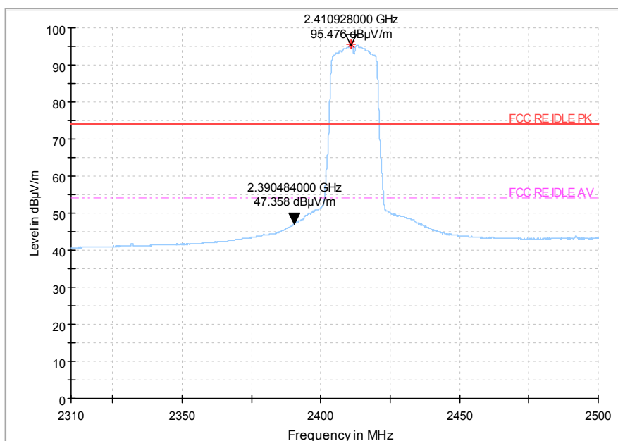
Fig.97 Radiated emission (Power): 802.11n(20M), low channel
