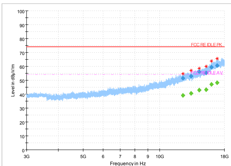
Fig.101 Radiated Spurious Emission (802.11n-20,Ch11,3GHz~18GHz)
