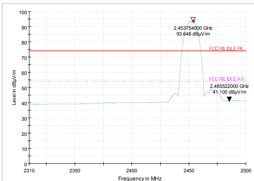
Fig.98 Radiated emission (Power): 802.11b, high channel
