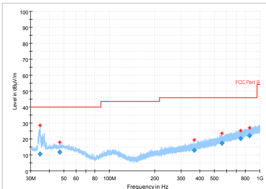
Fig.109 Radiated Spurious Emission (802.11 n-20MHz,Ch11,30MHz~1GHz)
