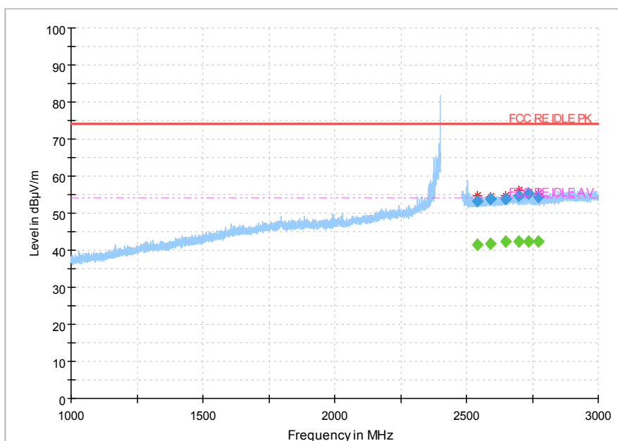
Fig.100 Radiated Spurious Emission (802.11n-20,Ch11,1GHz~3GHz)
