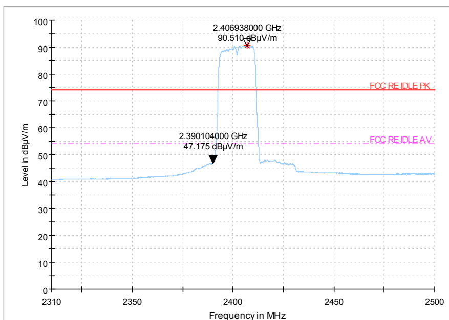
Fig.107 Radiated emission (Power): 802.11n, low channel
