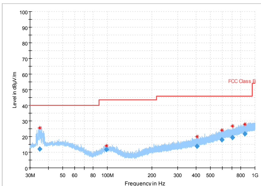
Fig.99 Radiated Spurious Emission (802.11n-20,Ch11,30MHz~1GHz)
