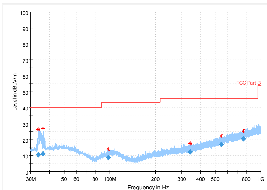
Fig.114 Radiated Spurious Emission (802.11 n-40MHz,Ch9,30MHz~1GHz)
