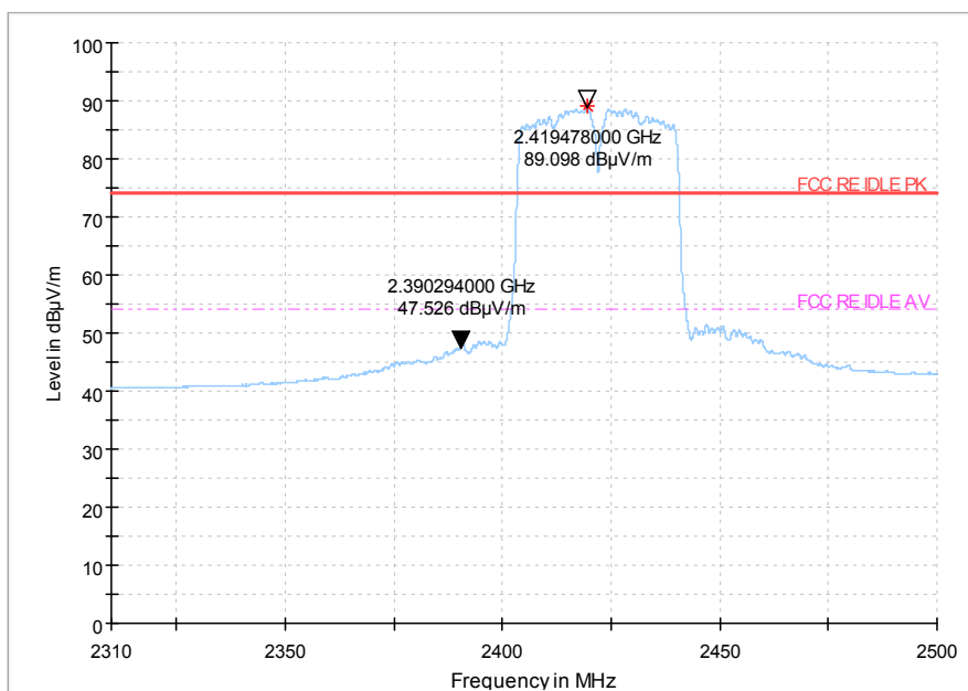
Fig.112 Radiated emission (Power): 802.11n (40M) , low channel
