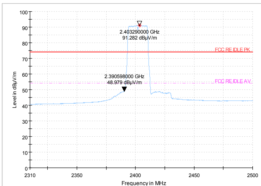
Fig.102 Radiated emission (Power): 802.11g, low channel
