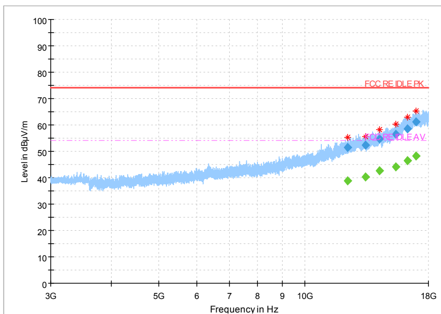
Fig.111 Radiated Spurious Emission (802.11 n-20MHz,Ch11,3GHz~18GHz)
