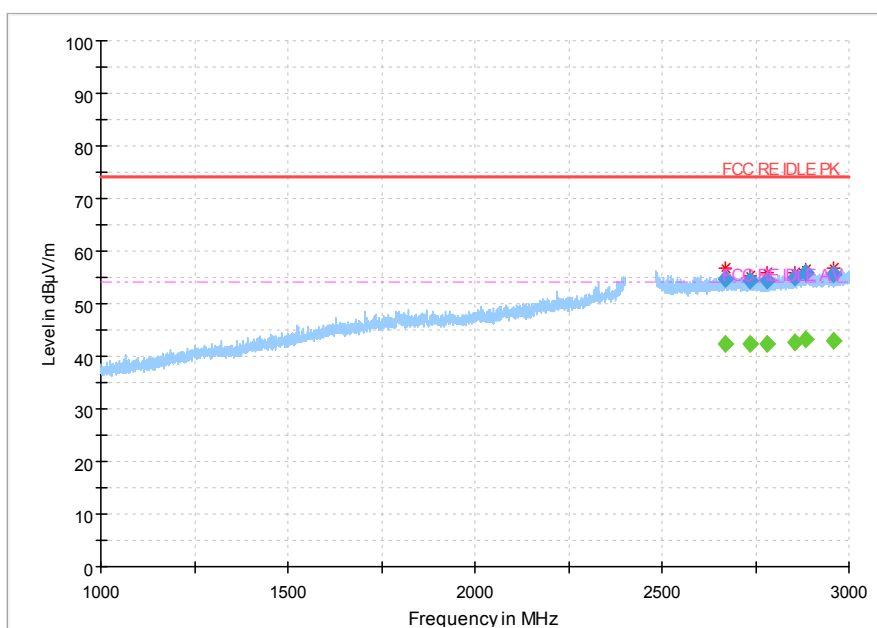
Fig.105 Radiated Spurious Emission (802.11g,Ch11,1GHz~3GHz)
