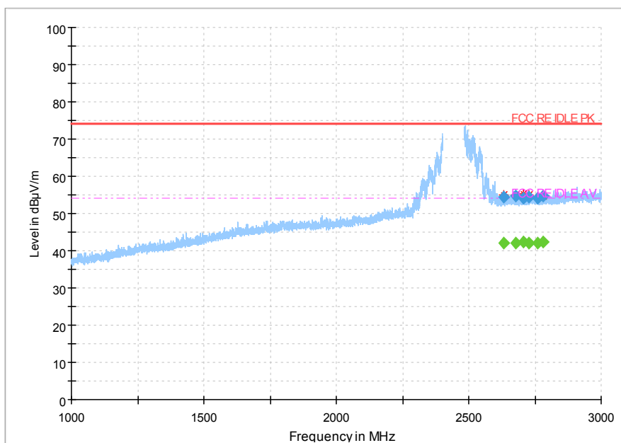
Fig.115 Radiated Spurious Emission (802.11 n-40MHz,Ch9,1GHz~3GHz)
