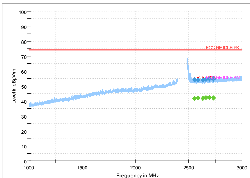
Fig.110 Radiated Spurious Emission (802.11 n-20MHz,Ch11,1GHz~3GHz)
