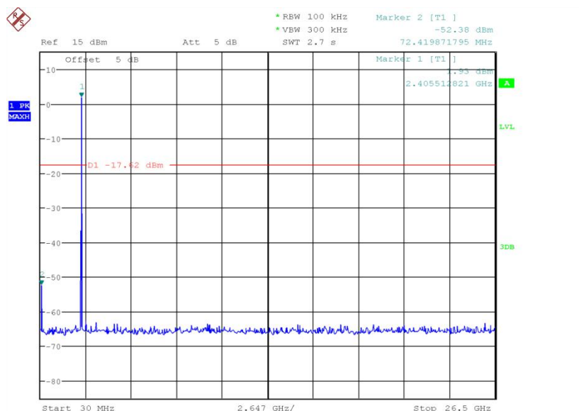
Fig.12 Conducted spurious emission: Ch0, 2402MHz
