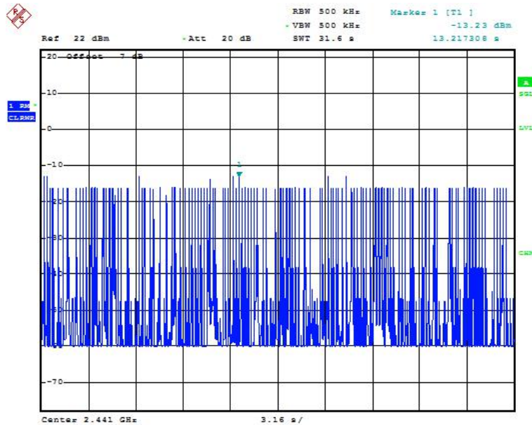
Fig.74 Time of occupancy (Dwell Time): Ch39,Packet 3-DH3
