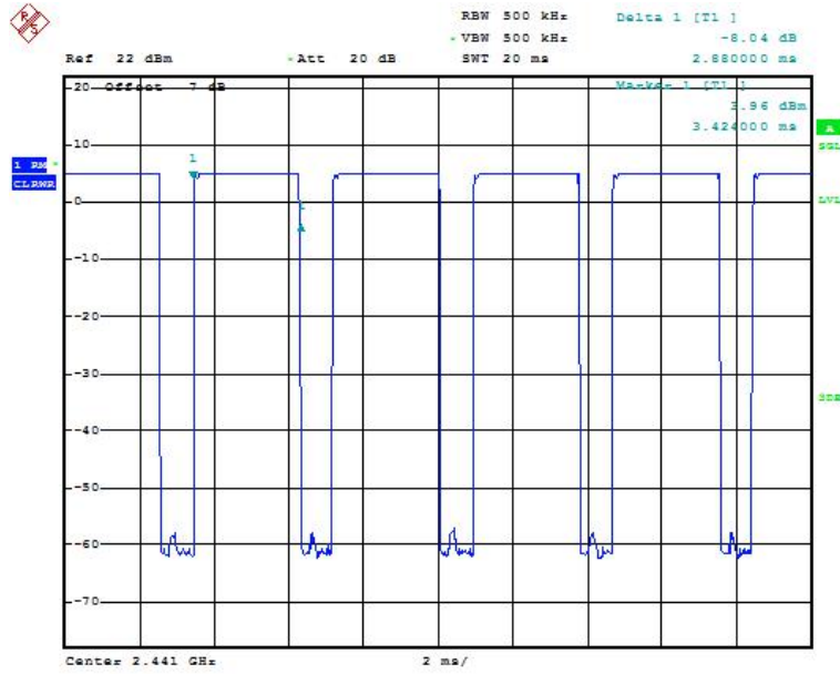
Fig.64 Time of occupancy (Dwell Time): Ch39,Packet DH5
