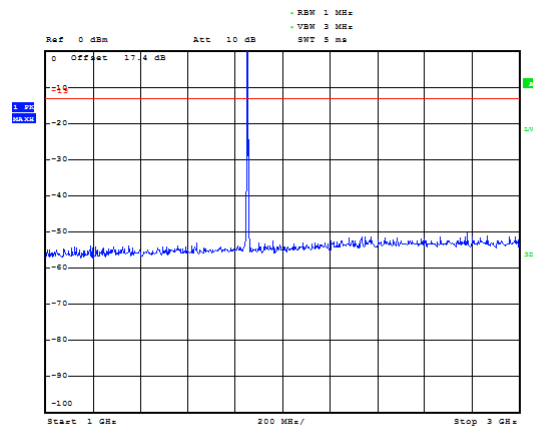
GPRS 1900 CH-Low 1GHz~3GHz
