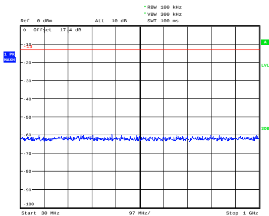
GPRS 1900 CH-Low 30MHz~1GHz
