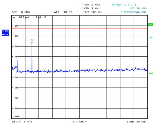
GPRS 1900 CH-Low 3GHz~20GHz
