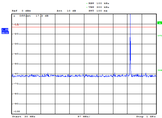
GPRS 850 CH-Low 30MHz ~ 1GHz
