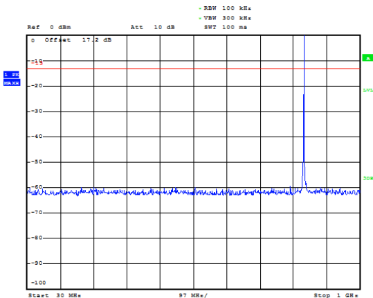
GPRS 850 CH-Middle 30MHz ~ 1GHz
