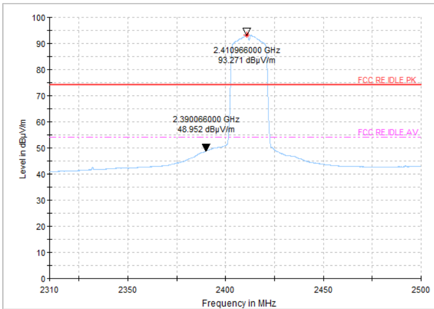
Fig.67 Radiated emission (Power): 802.11n, low channel
