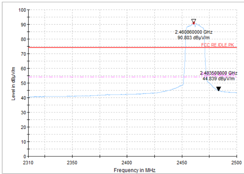
Fig.63 Radiated emission (Power): 802.11g, high channel
