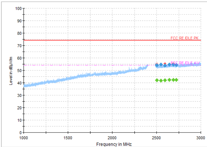
Fig.60 Radiated Spurious Emission (802.11b,Ch11,1GHz~3GHz)
