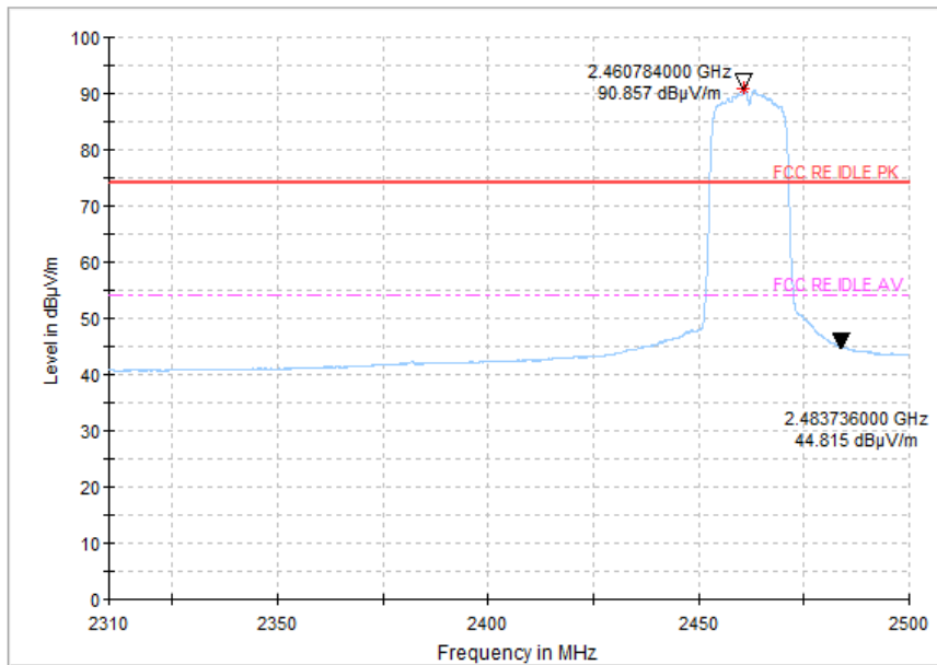
Fig.68 Radiated emission (Power): 802.11n, high channel
