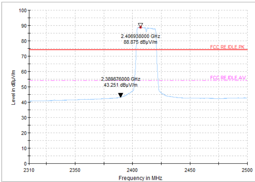
Fig.62 Radiated emission (Power): 802.11g, low channel
