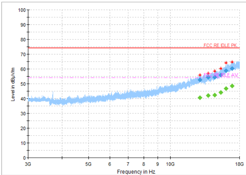
Fig.66 Radiated Spurious Emission (802.11g,Ch11,3GHz~18GHz)
