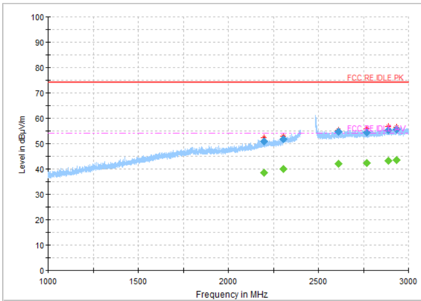
Fig.65 Radiated Spurious Emission (802.11g,Ch11,1GHz~3GHz)
