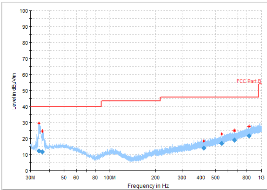
Fig.59 Radiated Spurious Emission (802.11b,Ch11,30MHz~1GHz)
