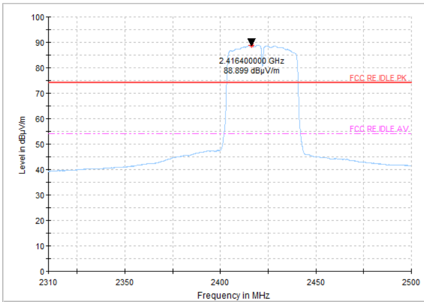
Fig.72 Radiated emission (Power): 802.11n (40M) , low channel
