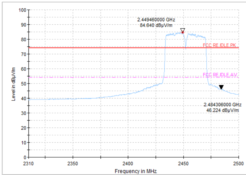
Fig.73 Radiated emission (Power): 802.11n (40M) , high channel
