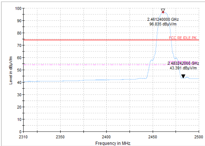
Fig.58 Radiated emission (Power): 802.11b, high channel
