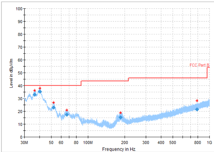
Fig.69 Radiated Spurious Emission (802.11 n-20MHz,Ch11,30MHz~1GHz)
