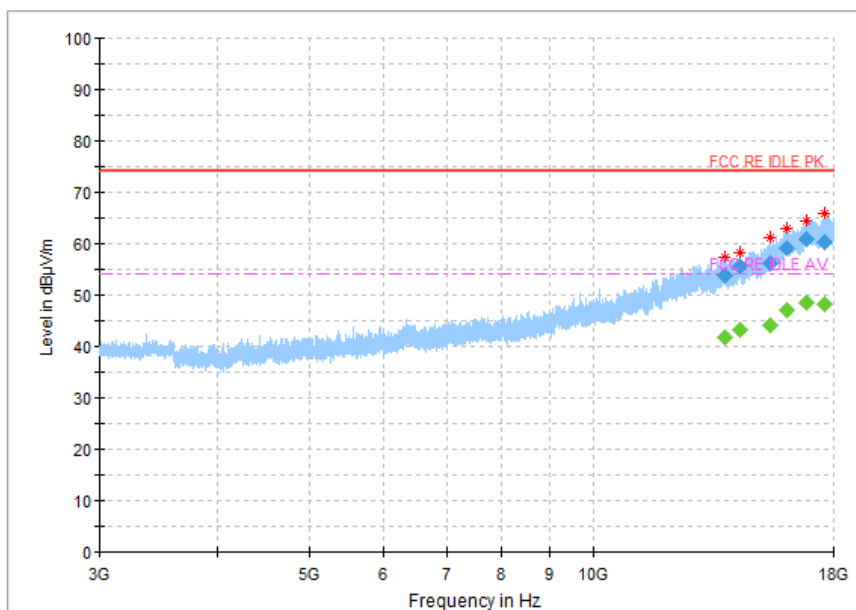
Fig.76 Radiated Spurious Emission (802.11 n-40MHz,Ch3,3GHz~18GHz)
