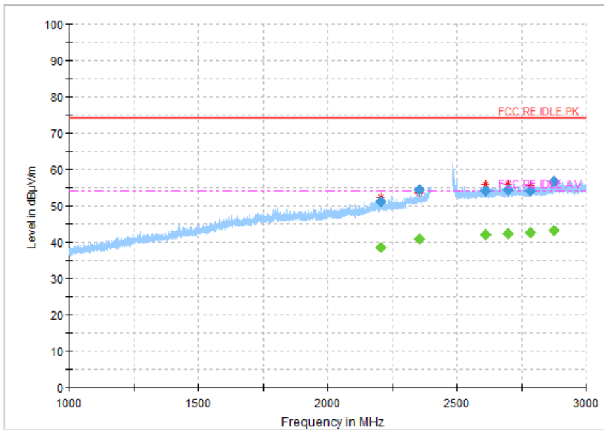
Fig.70 Radiated Spurious Emission (802.11 n-20MHz,Ch11,1GHz~3GHz)
