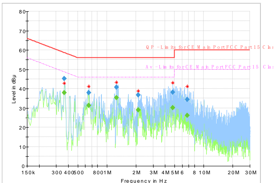
Fig.77 AC Power line Conducted Emission
