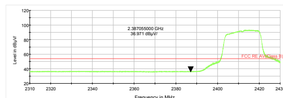
802.11g-Channel 1 Average
