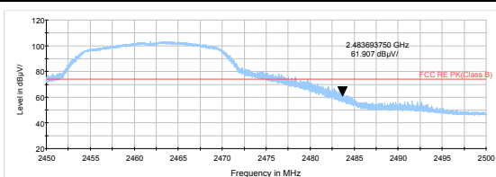
802.11g-Channel 11 Peak
