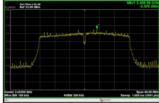
802.11n(HT40), Channel No.: 9
