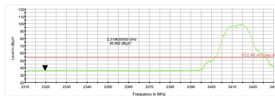
802.11b-Channel 1 Average
