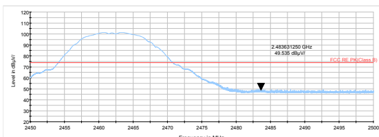
802.11b-Channel 11 Peak
