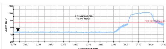
802.11g-Channel 1 Peak
