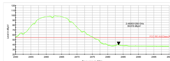
802.11b-Channel 11 Average
