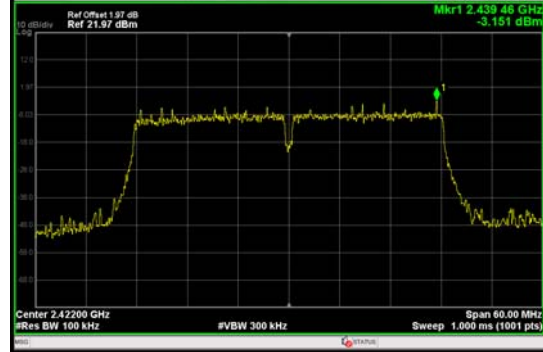
802.11n(HT40), Channel No.: 3
