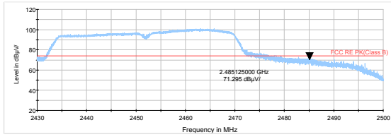
802.11n HT40 -Channel 9 Peak
