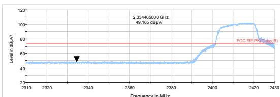
802.11n HT20 -Channel 1 Peak
