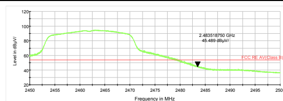
802.11g-Channel 11 Average
