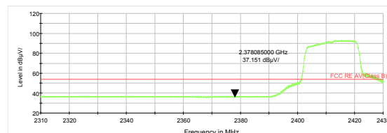
802.11n HT20 -Channel 1 Average
