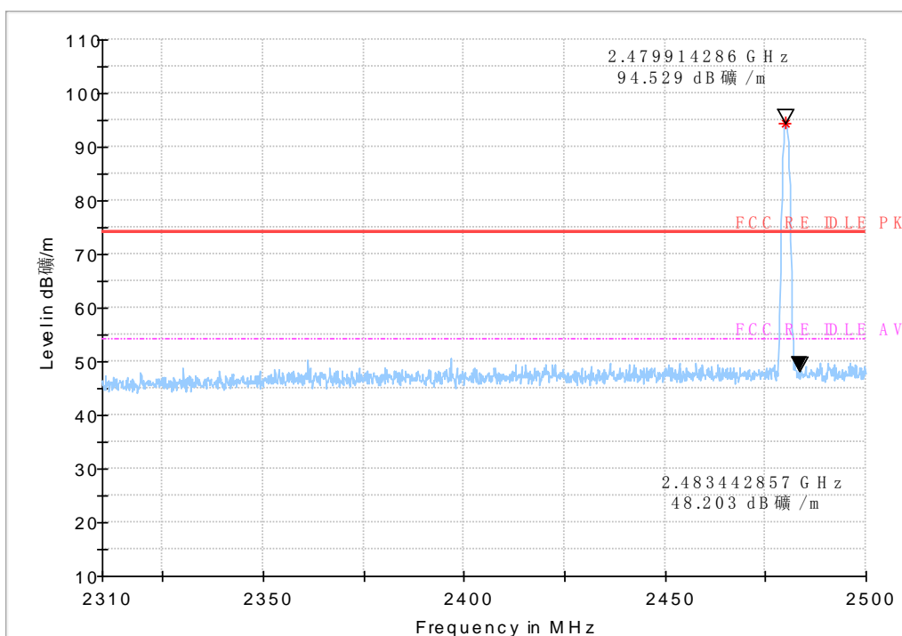
Fig.44 Radiated emission (Power): GFSK, high channel
