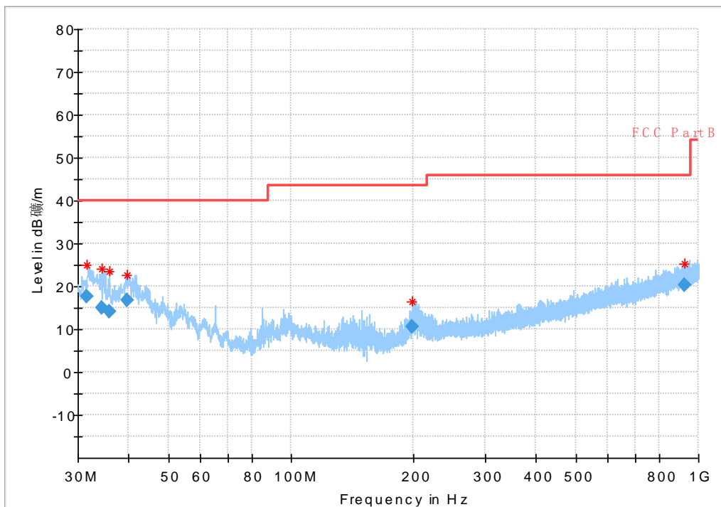
Fig.45 Radiated emission: \pi/4 DQPSK, Ch0, 30MHz~1GHz
