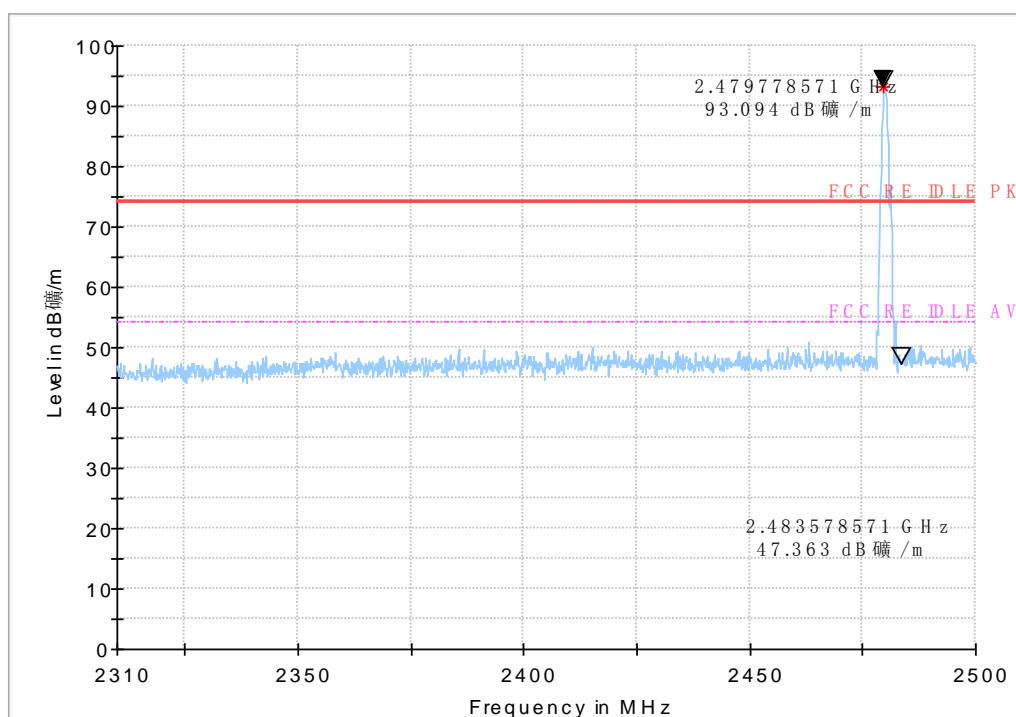
Fig.49 Radiated emission (Power): \pi/4 DQPSK, high channel
