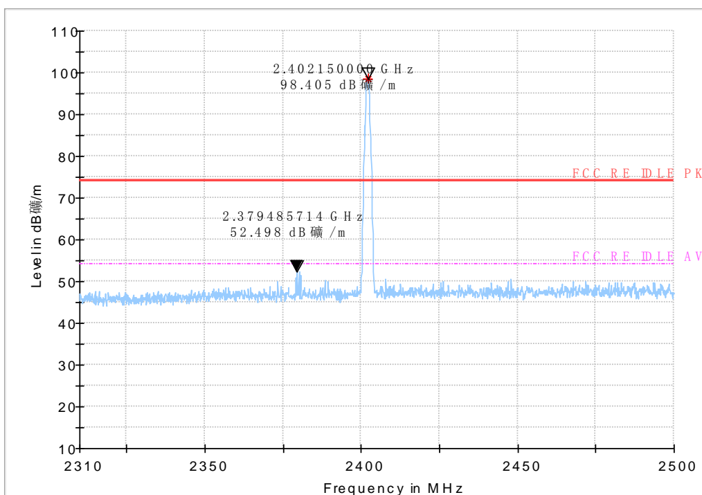
Fig.43 Radiated emission (Power): GFSK, low channel
