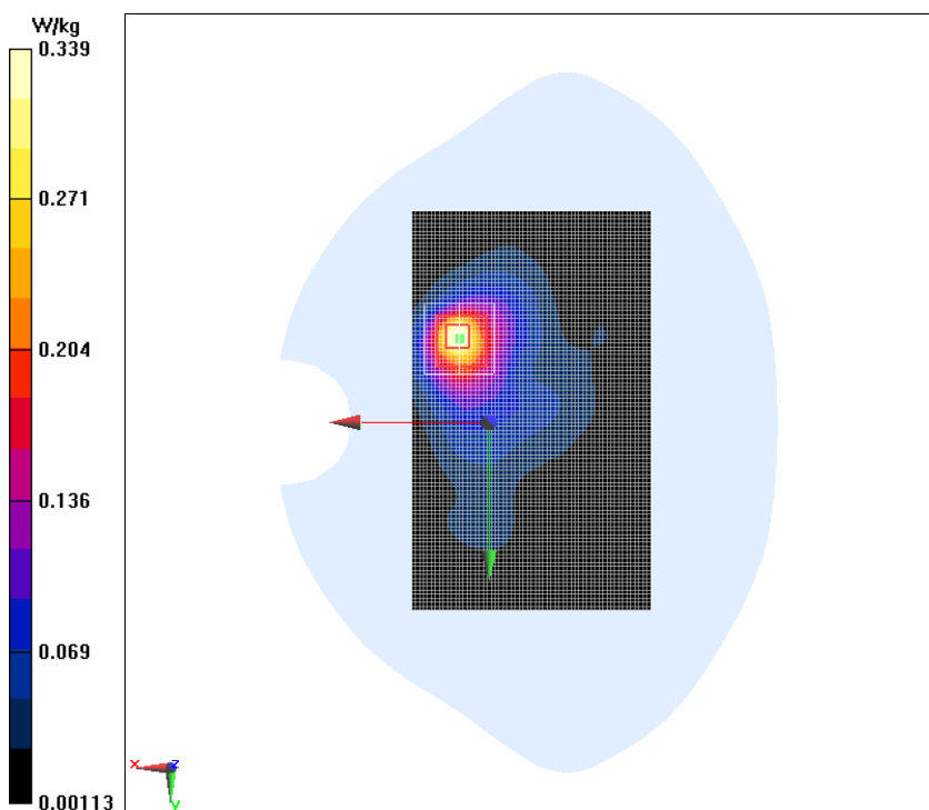
Fig.9 WiFi 802.11b Phantom Mode Middle
