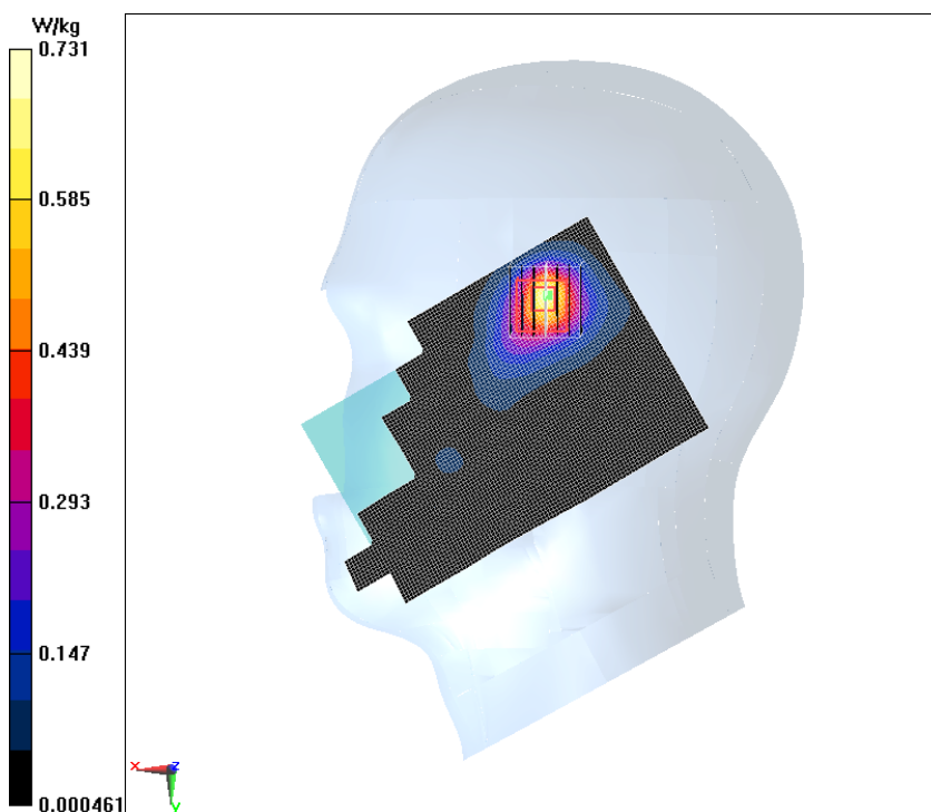
Fig.8 WiFi 802.11b Right Cheek Low
