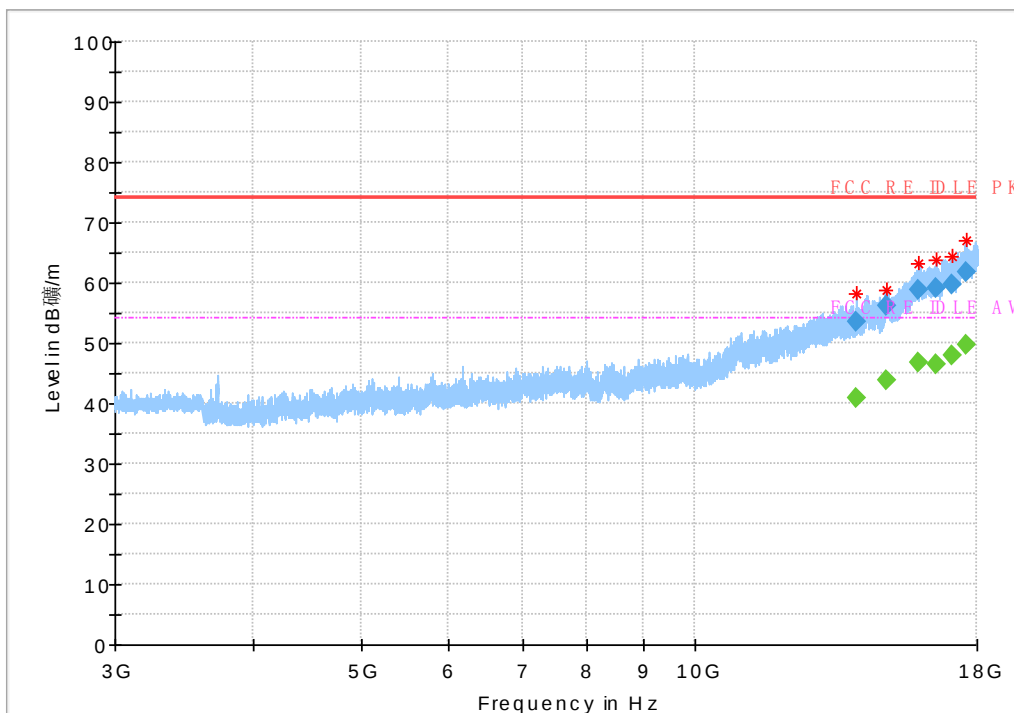
Fig.146 Radiated Spurious Emission (802.11 n-20Mhz,Ch13,3GHz~18GHz)
