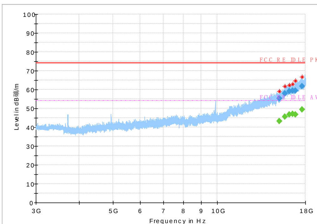
Fig.126 Radiated Spurious Emission (802.11b,Ch13,3GHz~18GHz)
