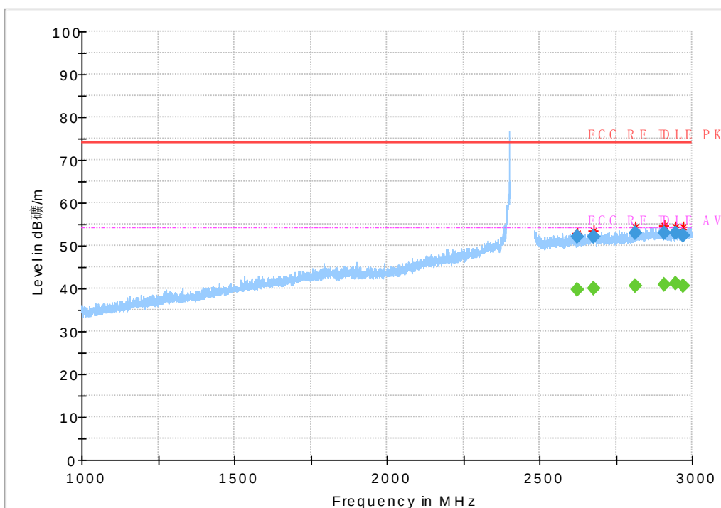
Fig.105 Radiated Spurious Emission (802.11g,Ch1,1GHz~3GHz)
