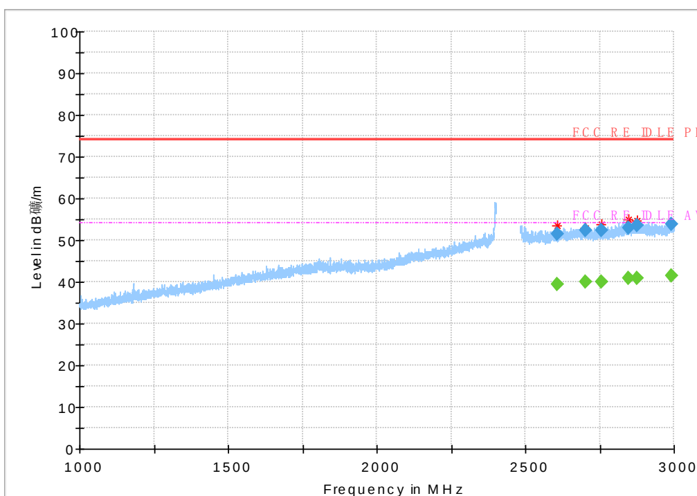
Fig.100 Radiated Spurious Emission (802.11b,Ch1,1GHz~3GHz)
