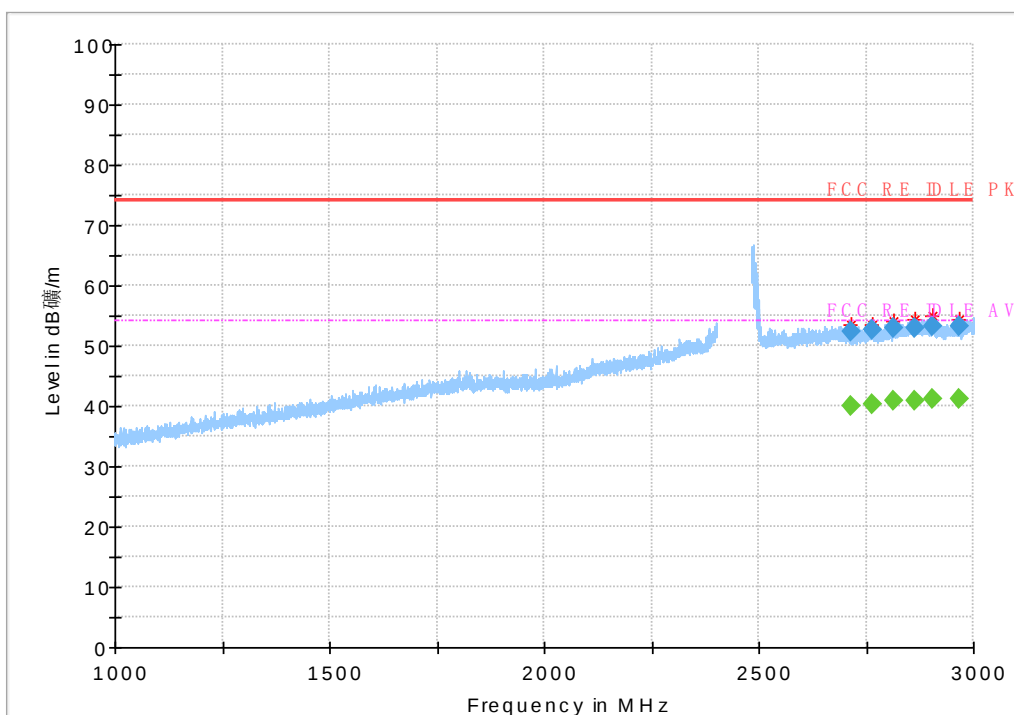
Fig.135 Radiated Spurious Emission (802.11g,Ch13,1GHz~3GHz)
