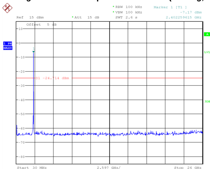
Fig.67 Conducted Spurious Emission (802.11g, Ch1)
