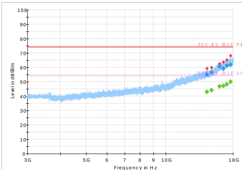
Fig.116 Radiated Spurious Emission (802.11 n-40MHz,Ch3,3GHz~18GHz)
