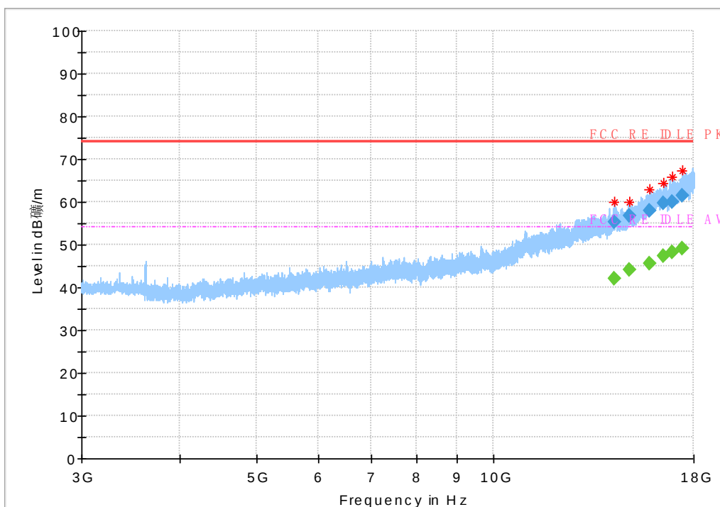
Fig.106 Radiated Spurious Emission (802.11g,Ch1,3GHz~18GHz)
