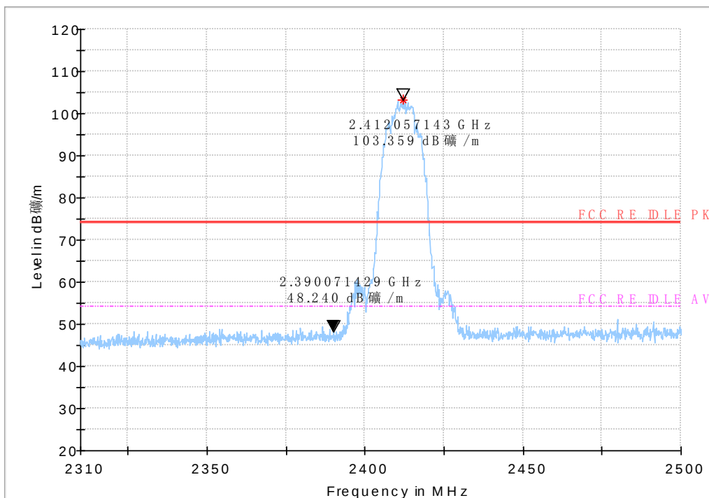
Fig.97 Radiated emission (Power): 802.11b, low channel
