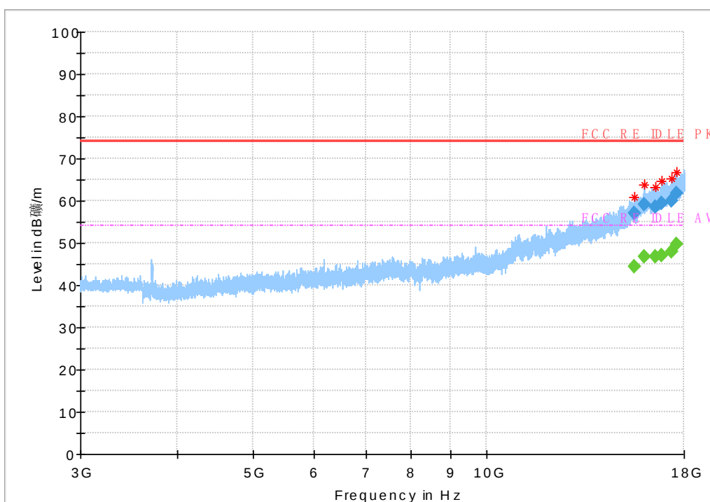
Fig.136 Radiated Spurious Emission (802.11g,Ch13,3GHz~18GHz)
