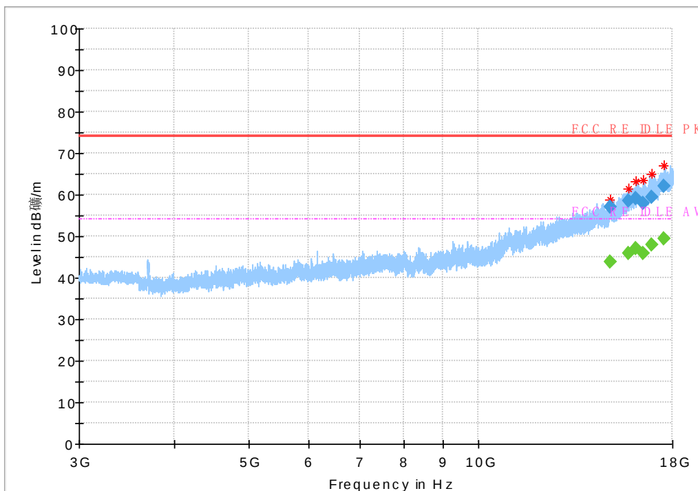
Fig.155 Radiated Spurious Emission (802.11 n-40Mhz,Ch11,3GHz~18GHz)
