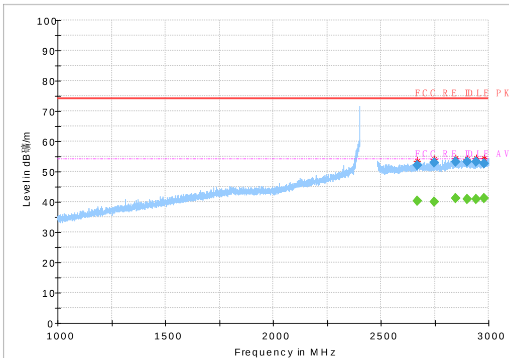
Fig.115 Radiated Spurious Emission (802.11 n-40MHz,Ch3,1GHz~3GHz)
