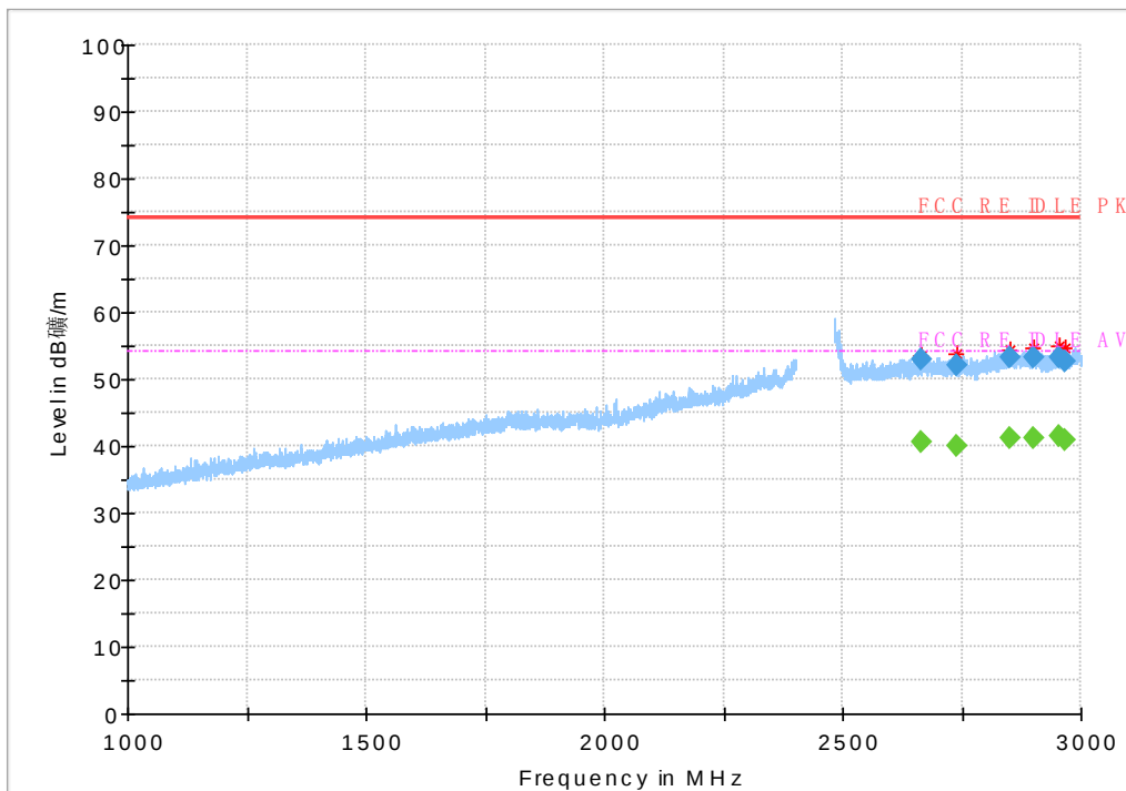
Fig.145 Radiated Spurious Emission (802.11 n-20Mhz,Ch13,1GHz~3GHz)
