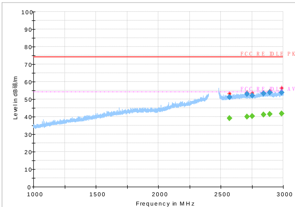
Fig.154 Radiated Spurious Emission (802.11 n-40Mhz,Ch11,1GHz~3GHz)
