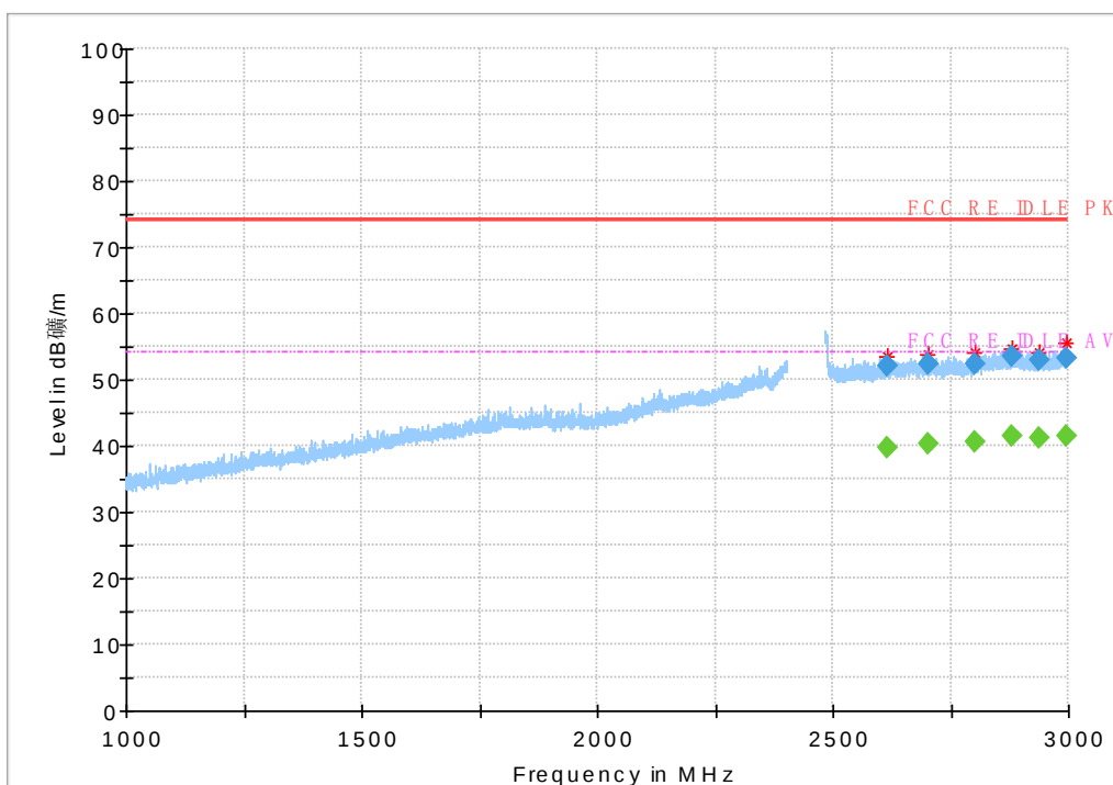
Fig.125 Radiated Spurious Emission (802.11b,Ch13,1GHz~3GHz)
