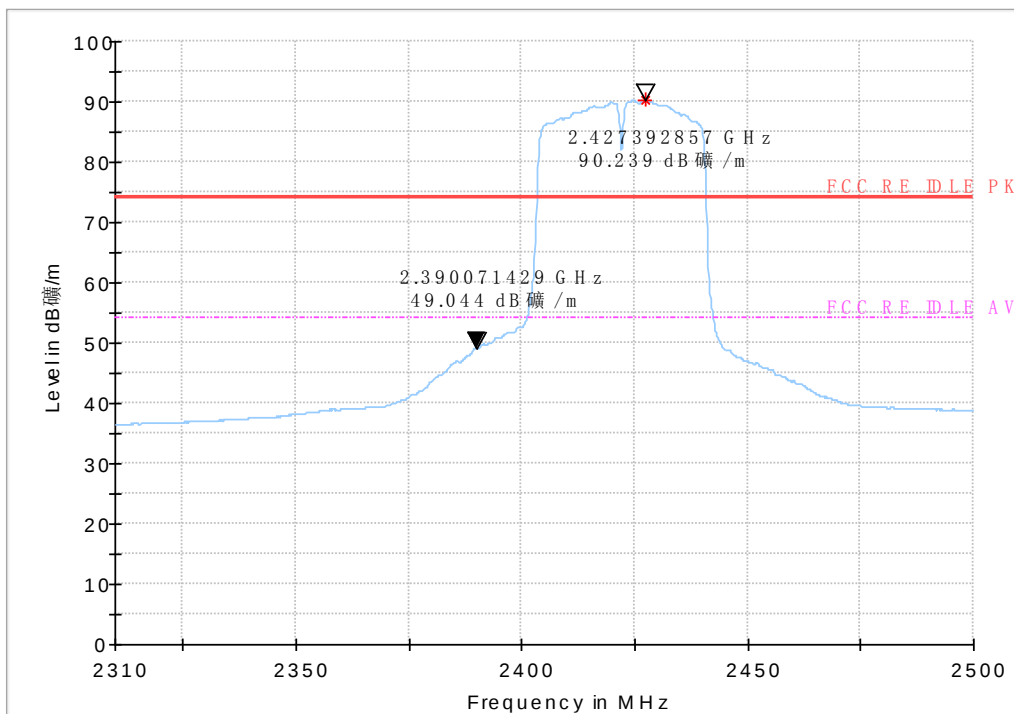
Fig.112 Radiated emission (Power): 802.11n (40M) , low channel
