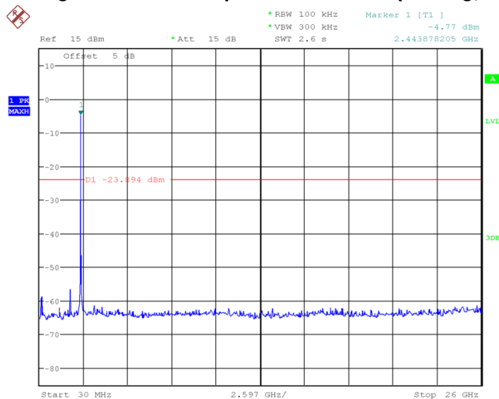
Fig.73 Conducted Spurious Emission (802.11g, Ch12)
