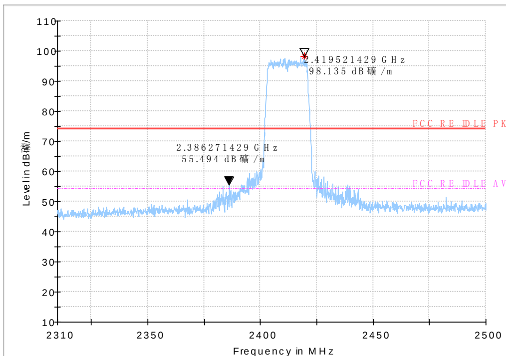
Fig.107 Radiated emission (Power): 802.11n, low channel
