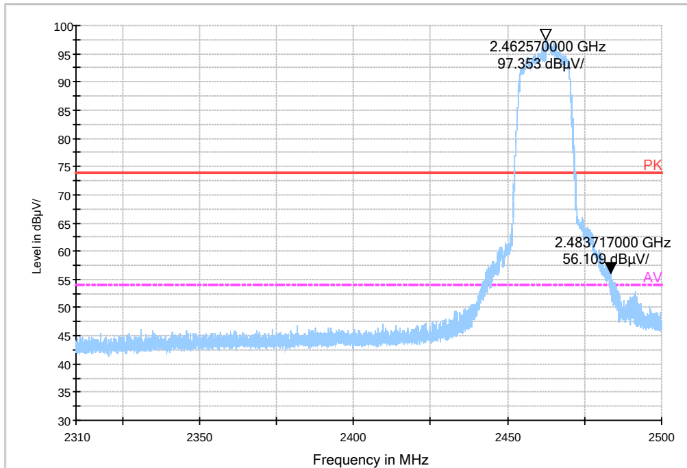
Fig.63 Radiated emission (Power): 802.11g, high channel
