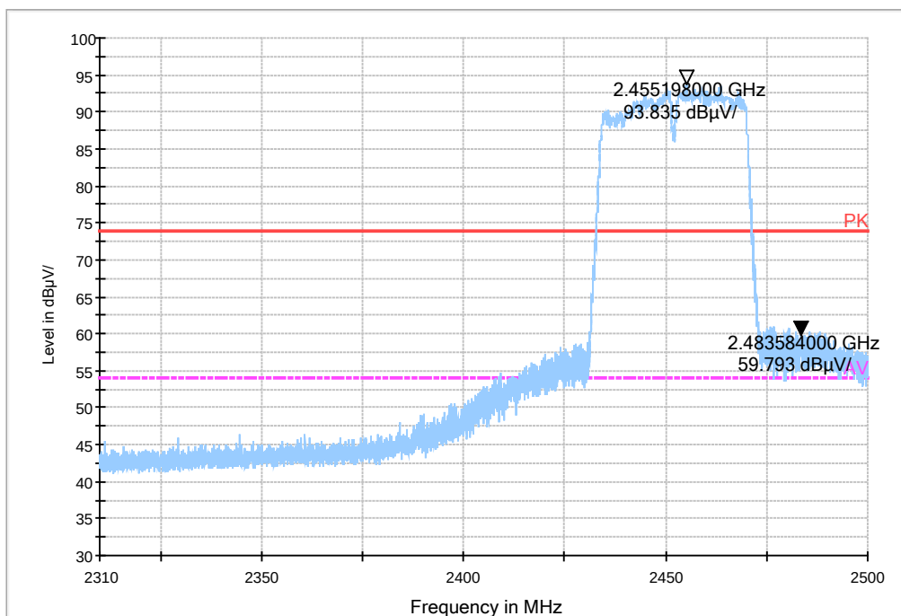
Fig.73 Radiated emission (Power): 802.11n (40M) , high channel
