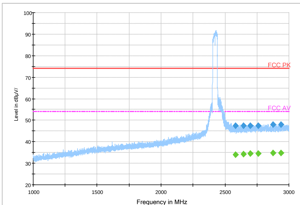
Fig.75 Radiated Spurious Emission (802.11 n-40MHz,Ch3,1GHz~3GHz)
