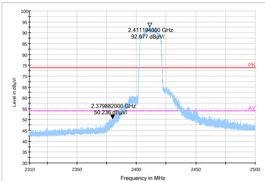
Fig.67 Radiated emission (Power): 802.11n, low channel
