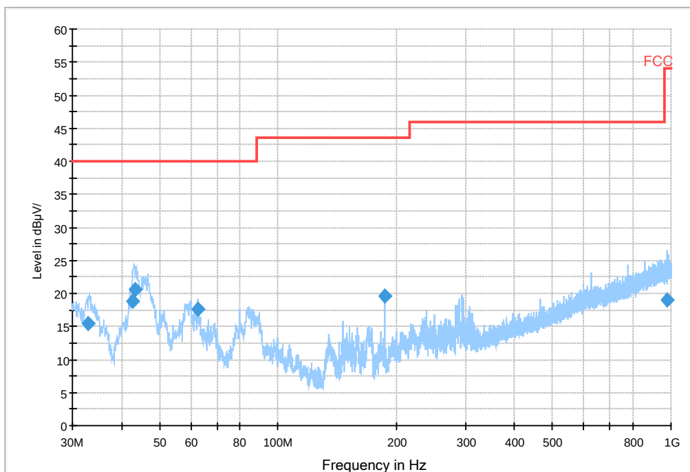
Fig.74 Radiated Spurious Emission (802.11 n-40MHz,Ch3,30MHz~1GHz)
