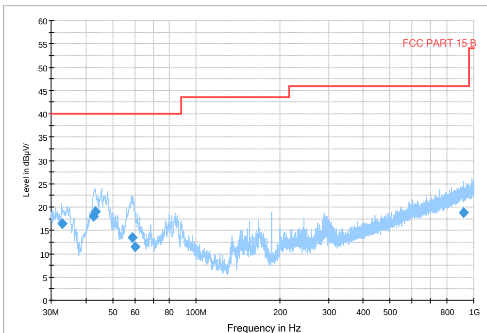
Fig.59 Radiated Spurious Emission (802.11b,Ch1,30MHz~1GHz)
