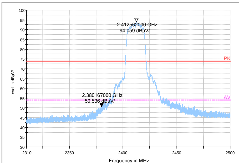
Fig.62 Radiated emission (Power): 802.11g, low channel
