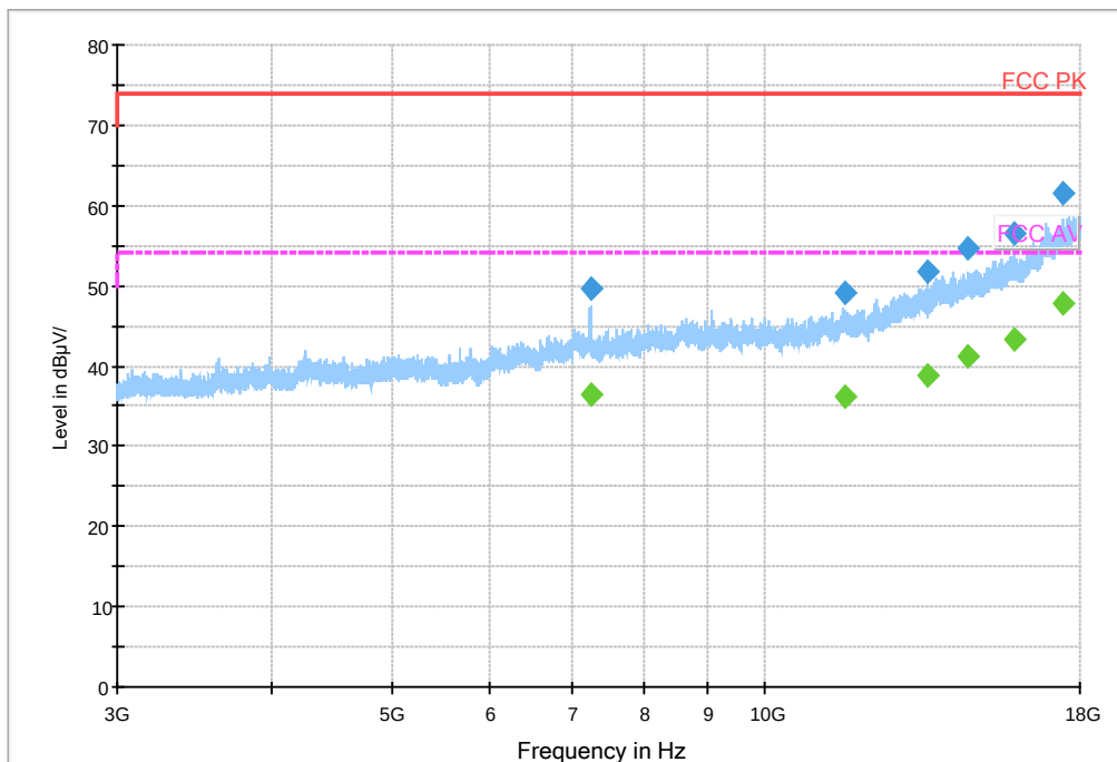
Fig.71 Radiated Spurious Emission (802.11 n-20MHz,Ch1,3GHz~18GHz)
