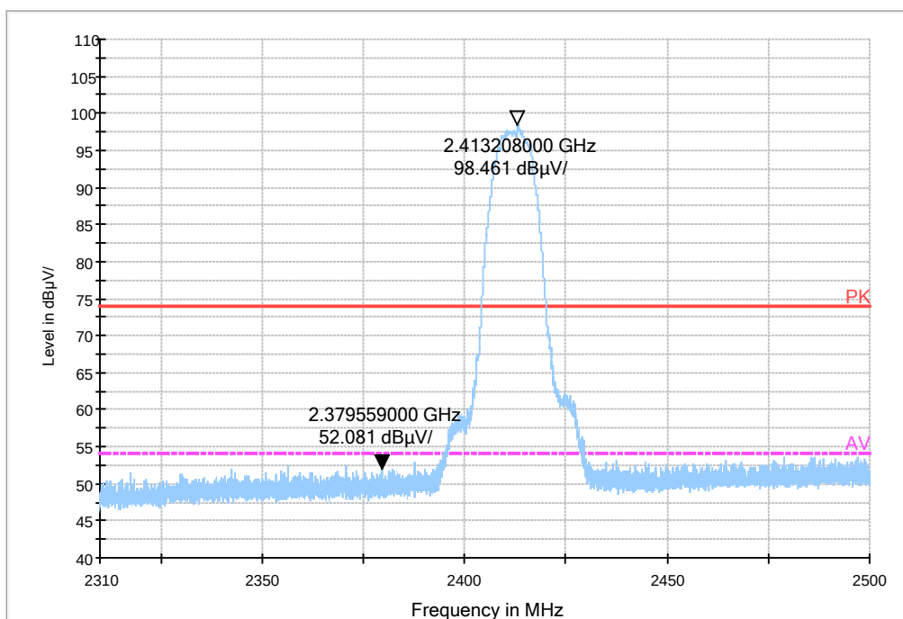
Fig.57 Radiated emission (Power): 802.11b, low channel
