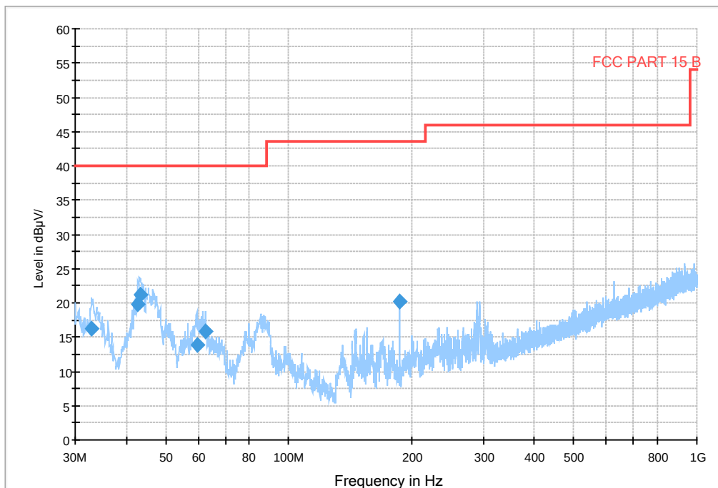
Fig.6.9 Radiated Spurious Emission (802.11 n-20MHz,Ch1,30MHz~1GHz)
