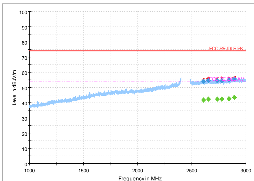
Fig 60. Radiated Spurious Emission (802.11b, Ch1, 1GHz~3GHz)
