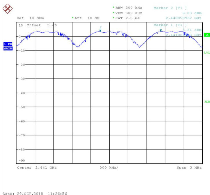
Fig.82 Carrier separation measurement: GFSK, Ch39
