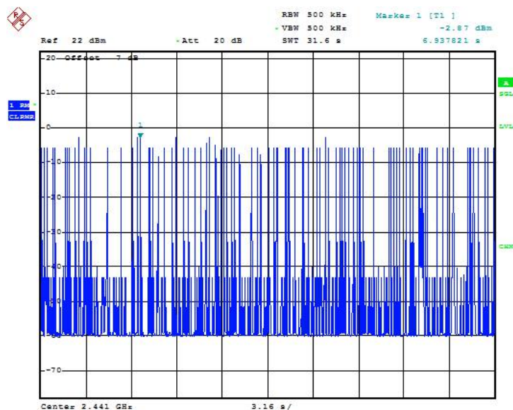
Fig.59 Time of occupancy (Dwell Time): Ch39,Packet DH5
