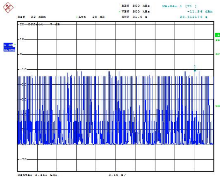
Fig.69 Time of occupancy (Dwell Time): Ch39,Packet 3-DH3
