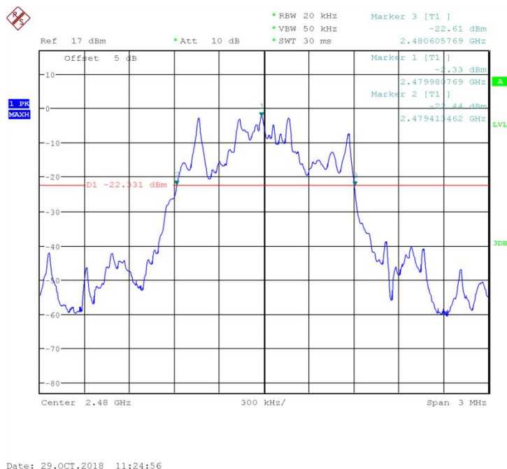
Fig.81 20dB Bandwidth: 8DPSK, Ch78
