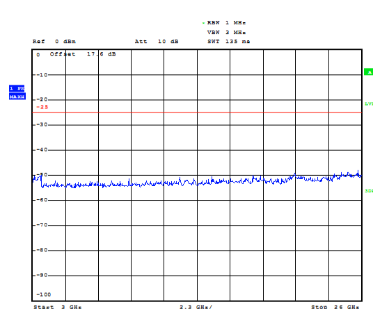
LTE Band 7 5MHz CH-Middle 3GHz~26GHz
