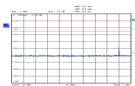
LTE Band 7 5MHz CH-Middle 30MHz~1GHz
