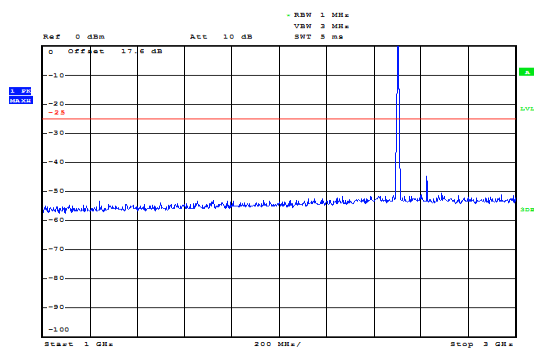
LTE Band 7 5MHz CH-Low 1GHz~3GHz
