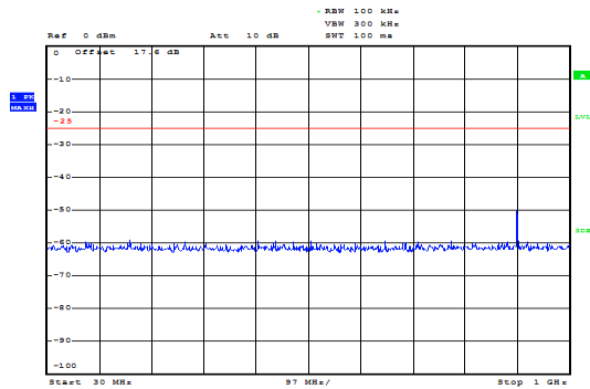
LTE Band 7 5MHz CH-Low 30MHz~1GHz
