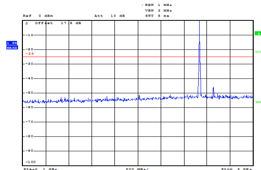
LTE Band 7 5MHz CH-Middle 1GHz~3GHz
