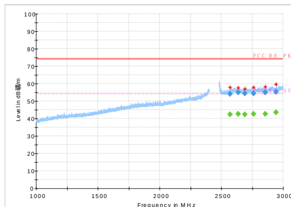
Radiated Spurious Emission (802.11n-20MHz, Ch11, 1GHz~3GHz)
