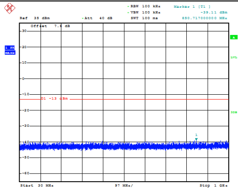
Channel 512: 30MHz~1GHz
