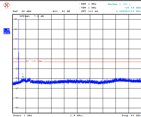
Channel 512: 1GHz~20GHz
