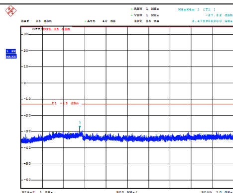
Channel 251: 1GHz~10GHz
