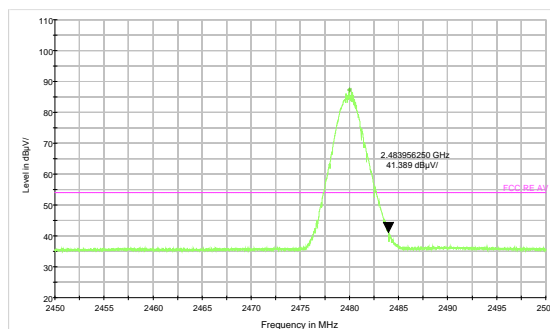
3DH5-Channel 78: Average
