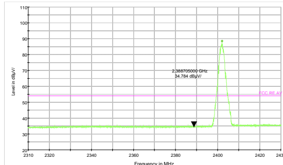
3DH5-Channel 0: Average
